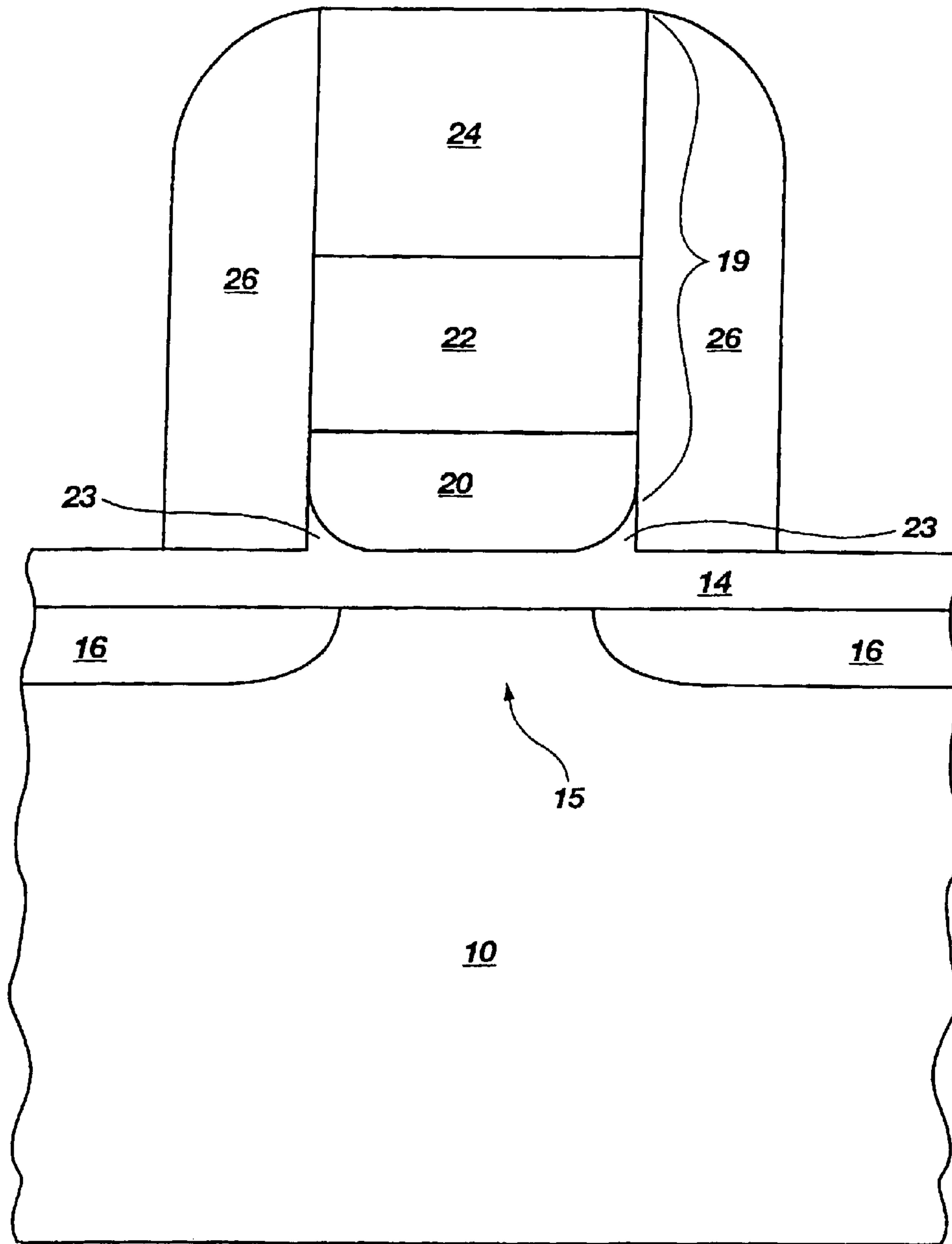
Fig. 1 (PRIOR ART)
