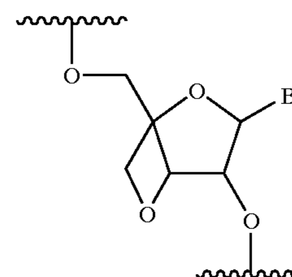
3' - 4' LNA
