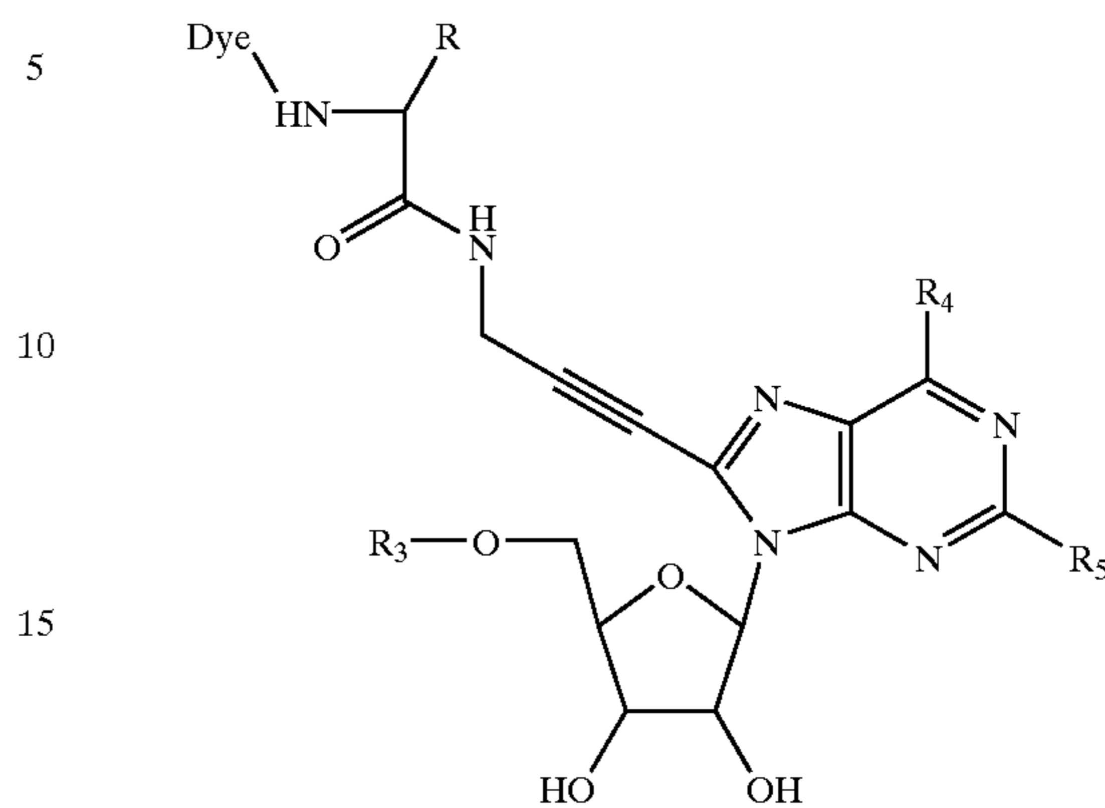
Formula VII
