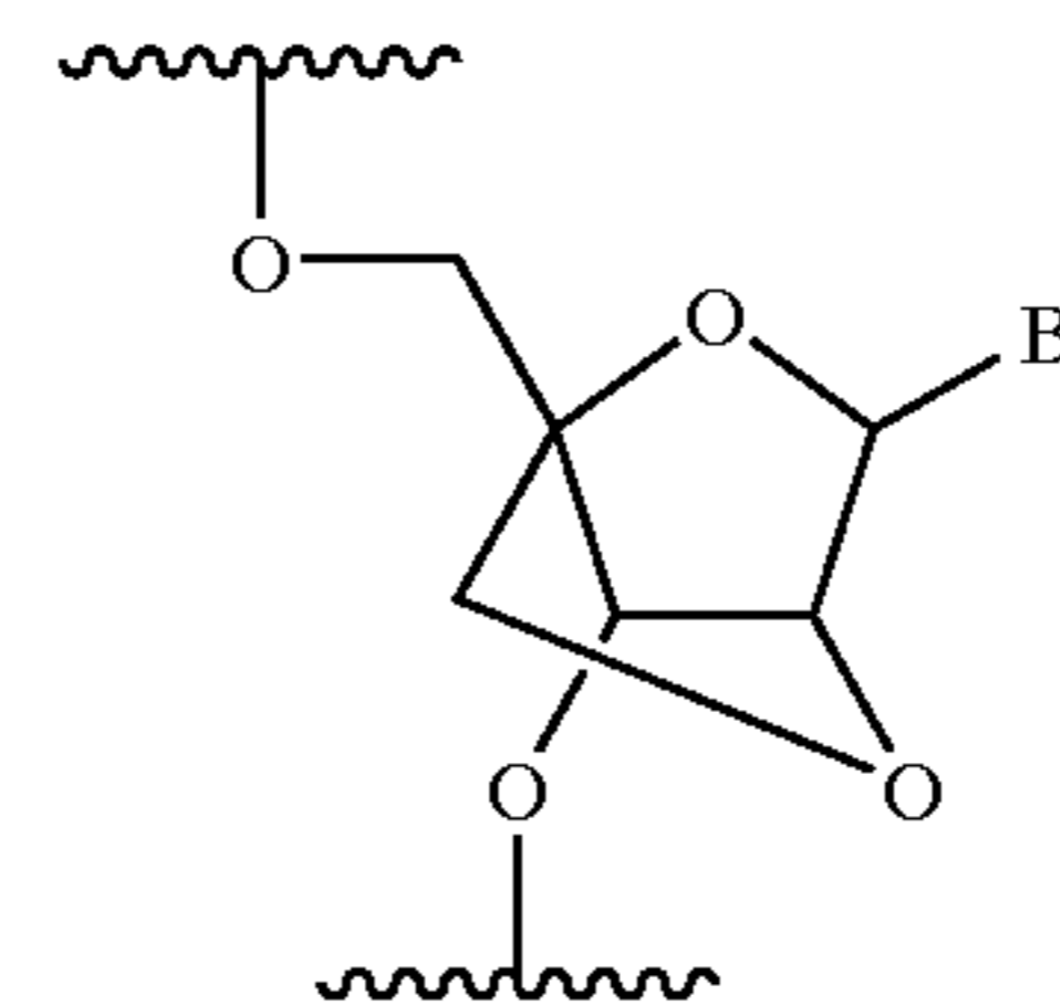
2' - 4' LNA
