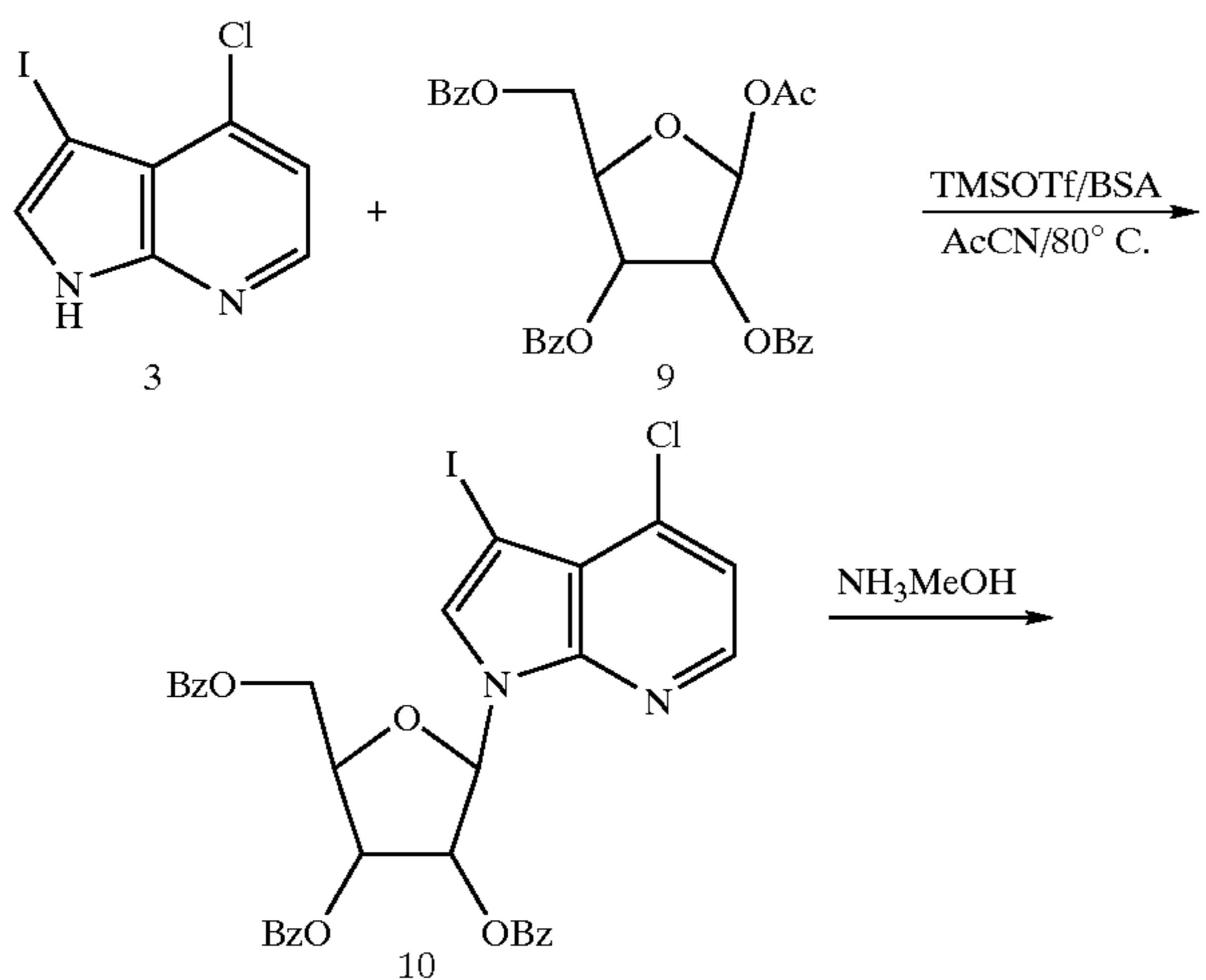
Scheme II
