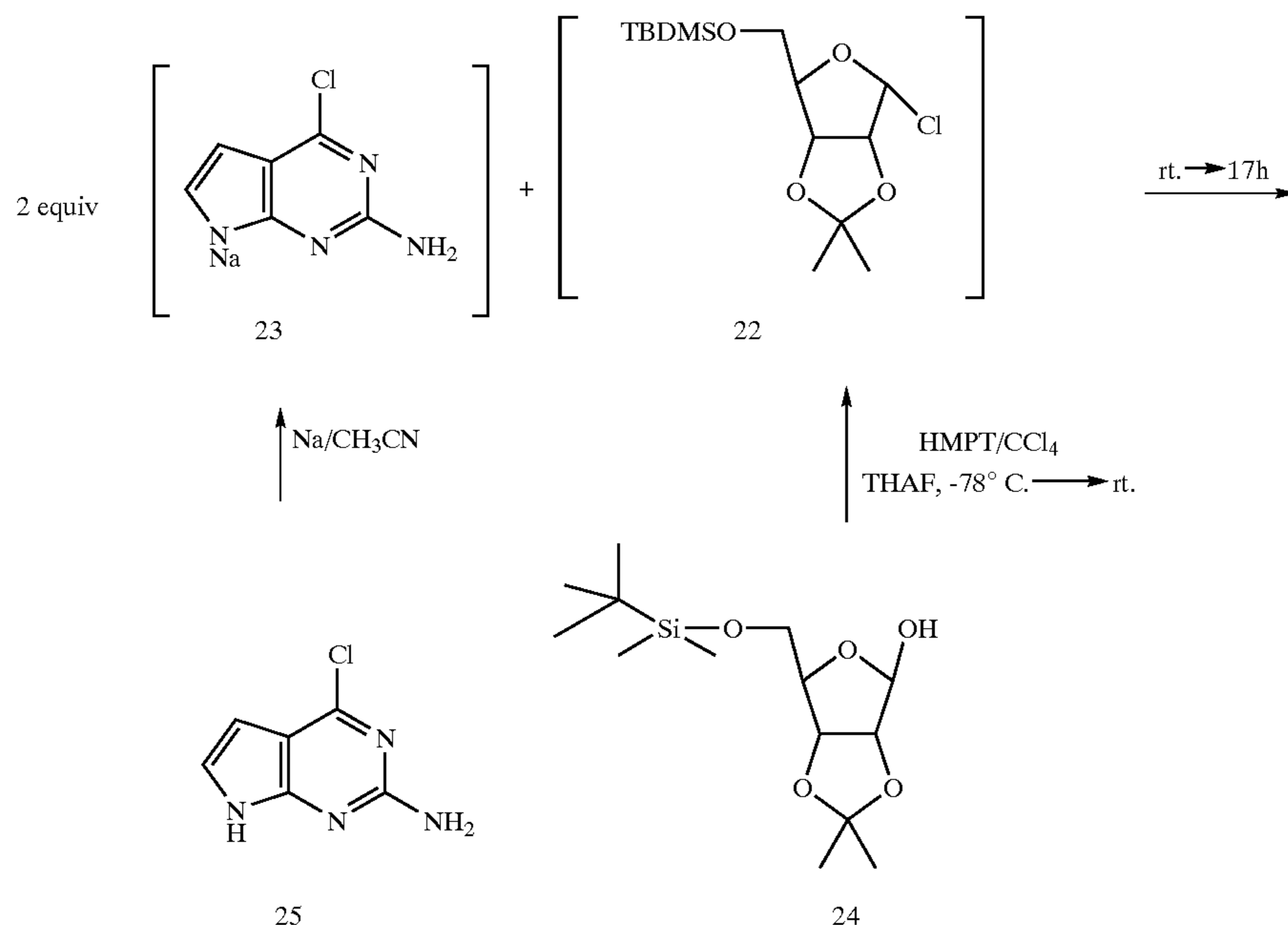
Scheme III
