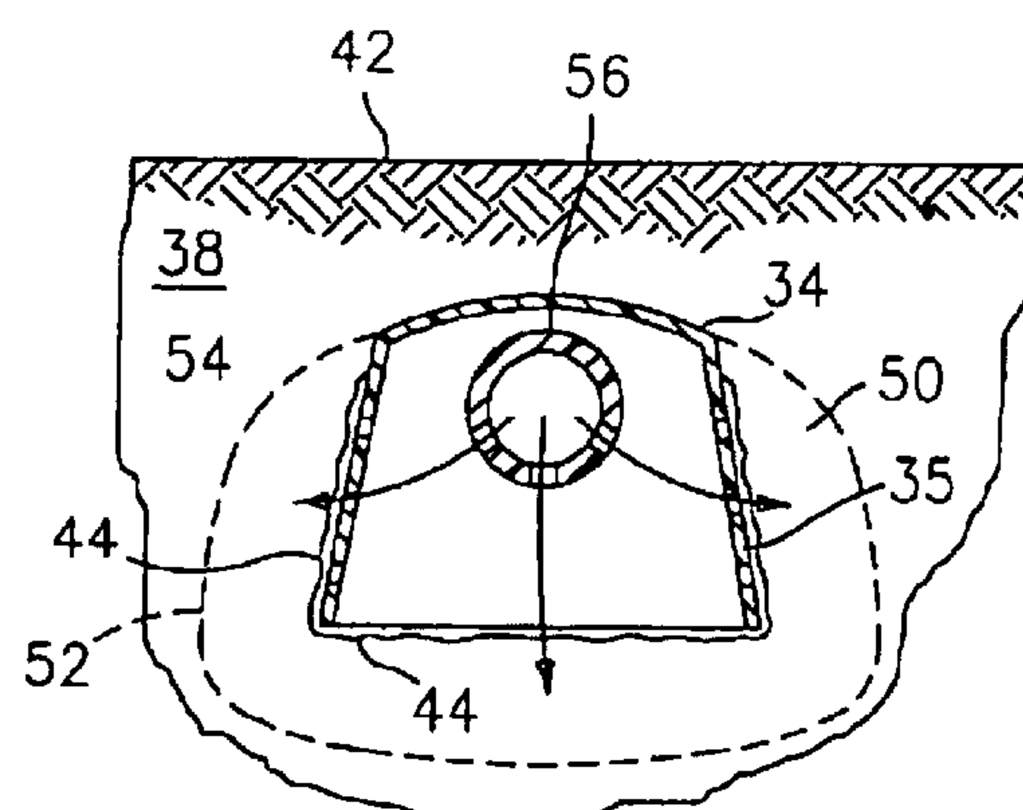
FIG. 3 (PRIOR ART)
