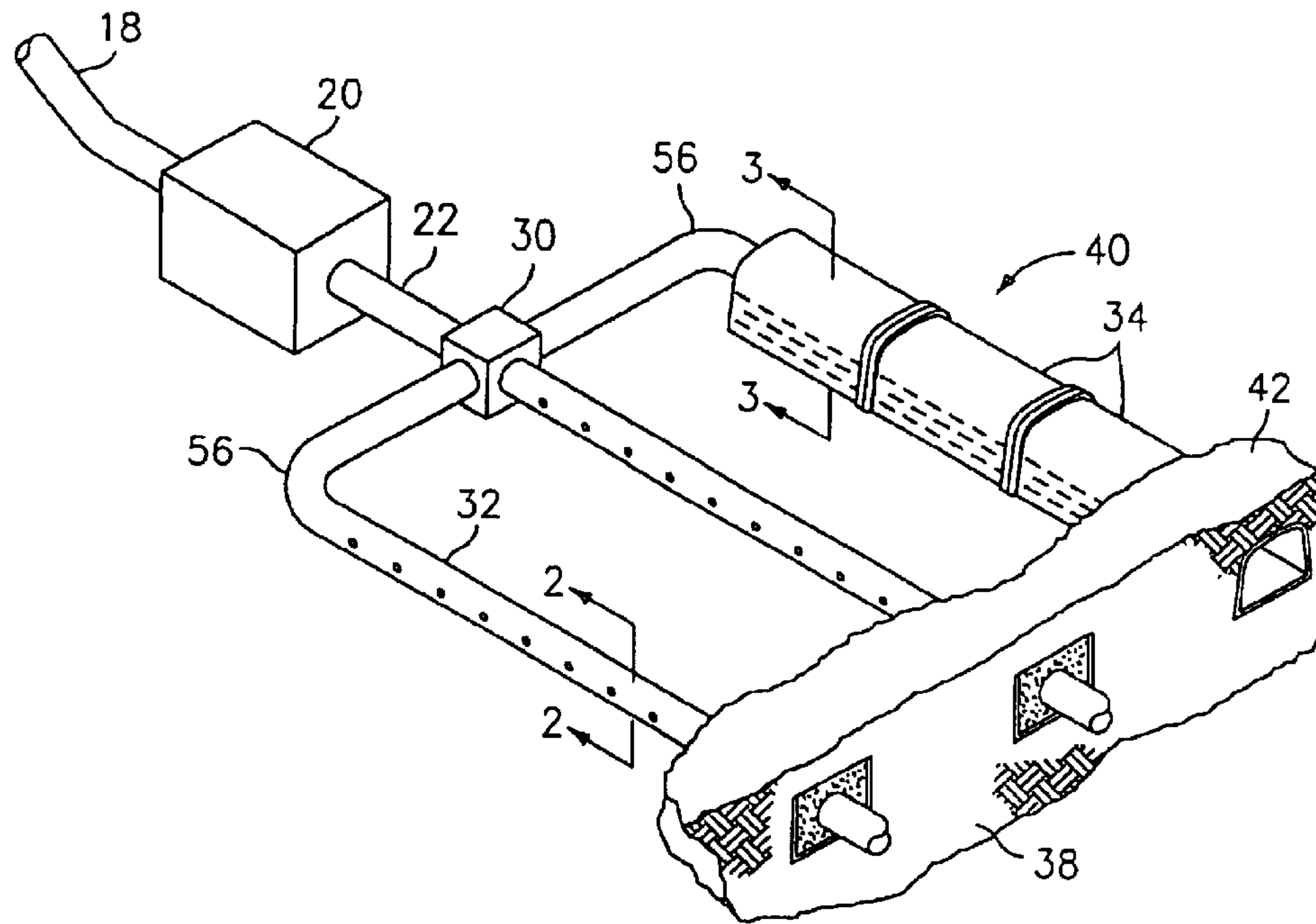
FIG. 1 (PRIOR ART)
