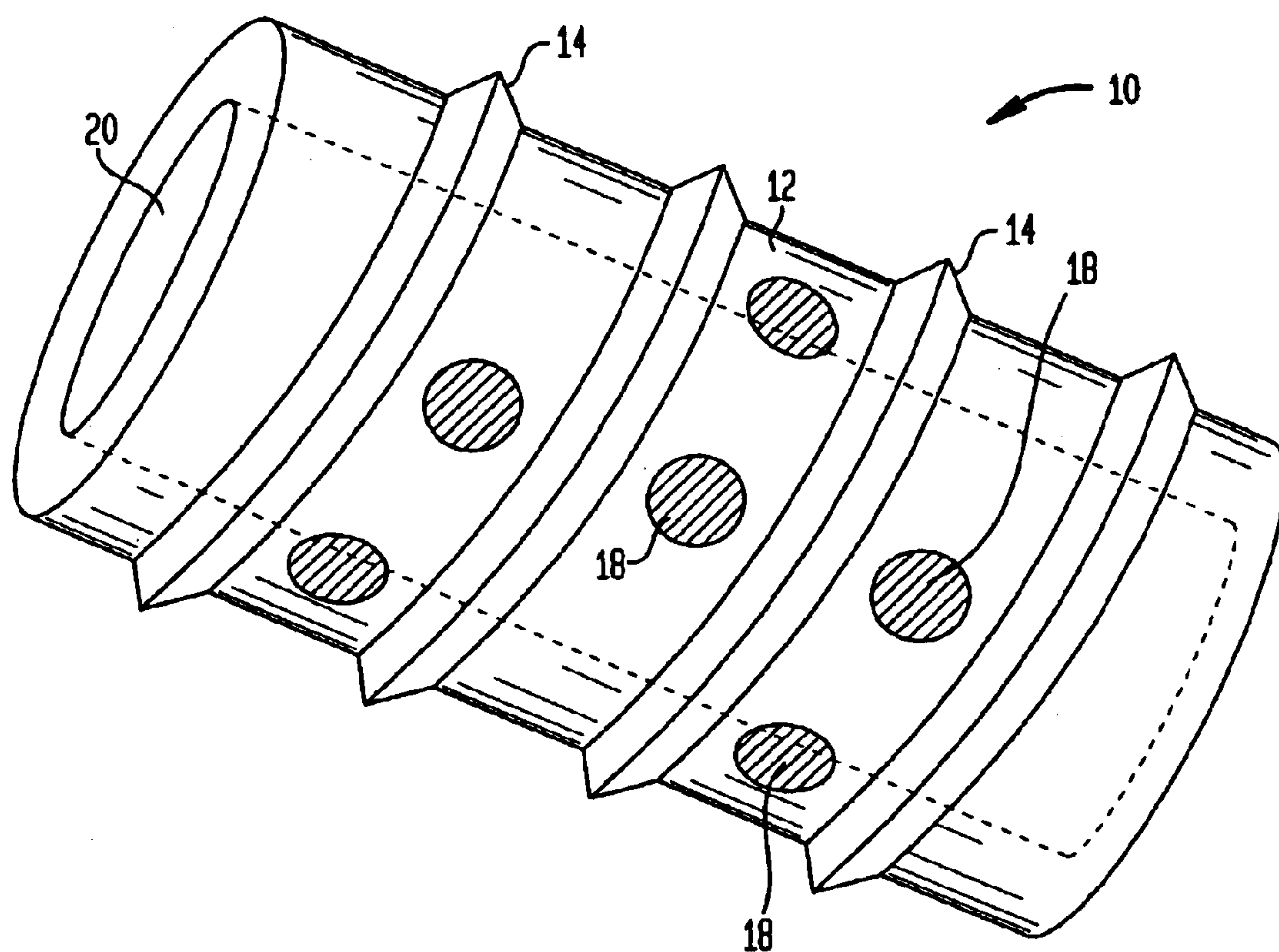
FIG. 1 (PRIOR ART)
