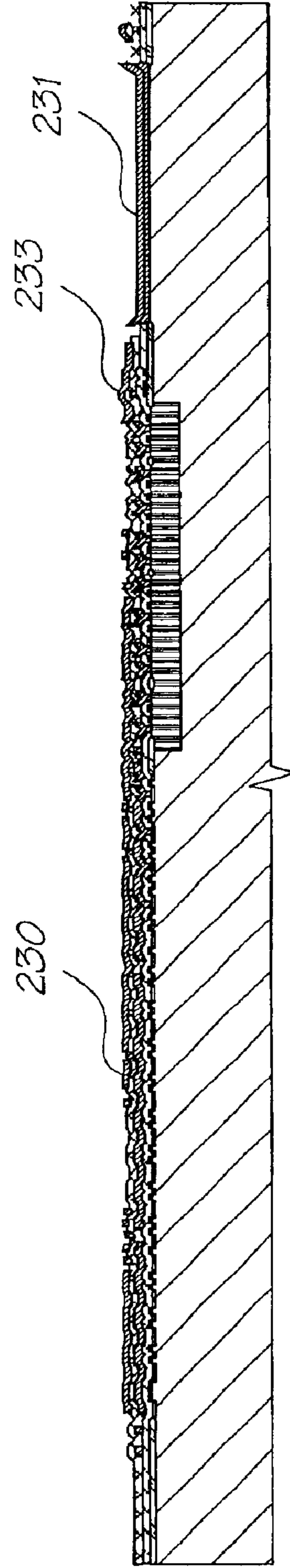
Deposit metal 2
