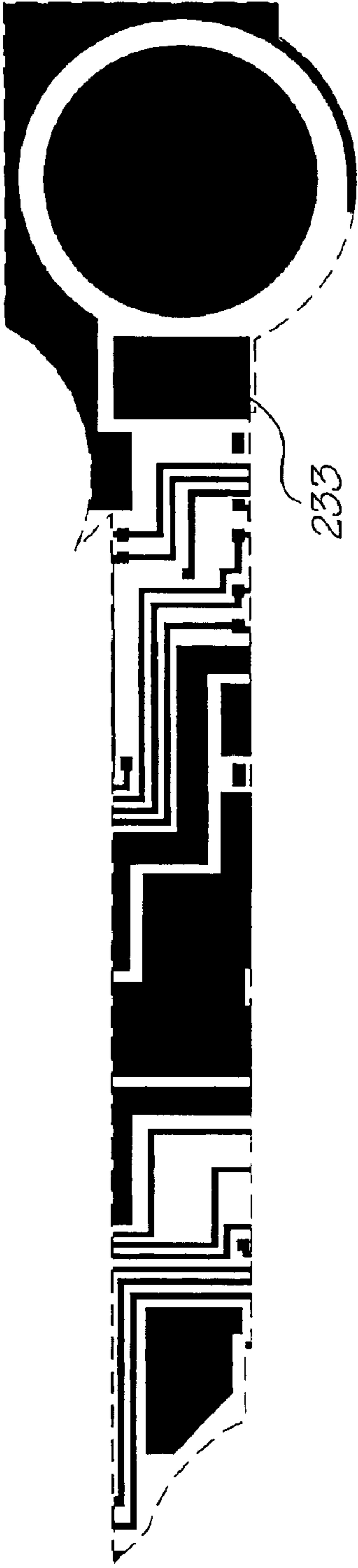
Metal 2 mask
