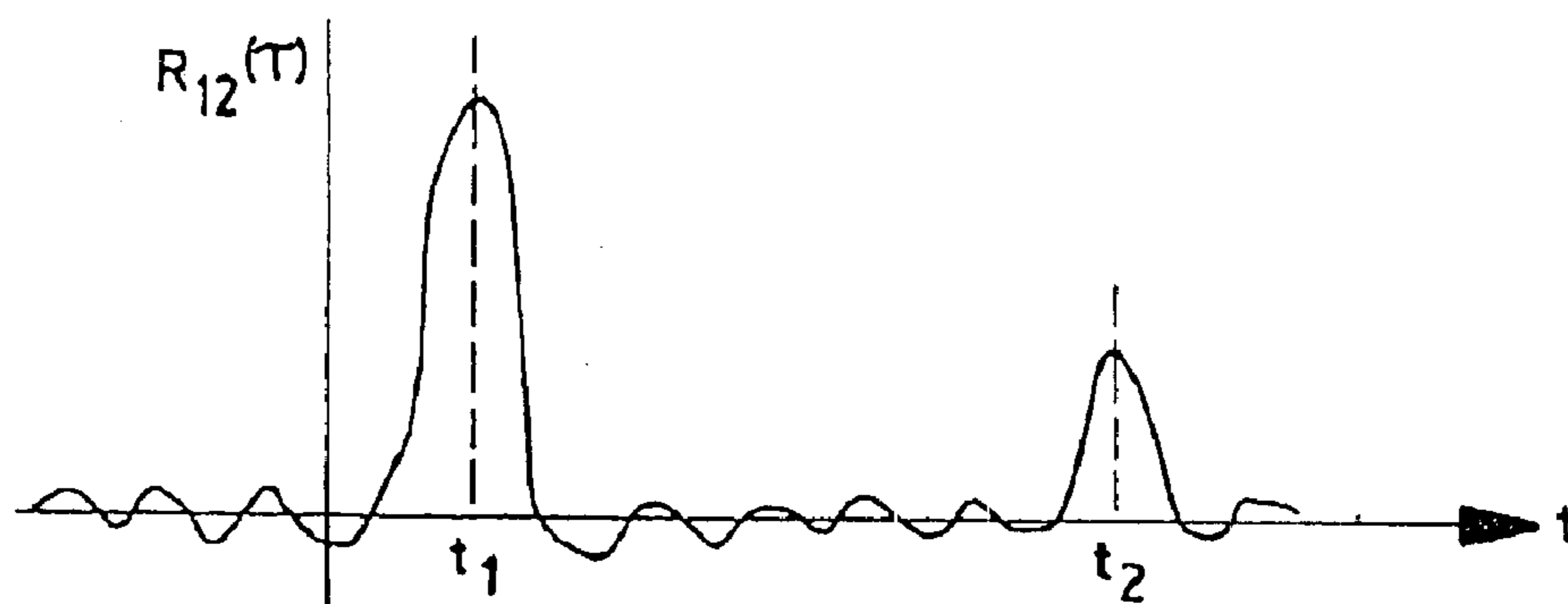
TYPICAL CROSS-CORRELATION FUNCTION
