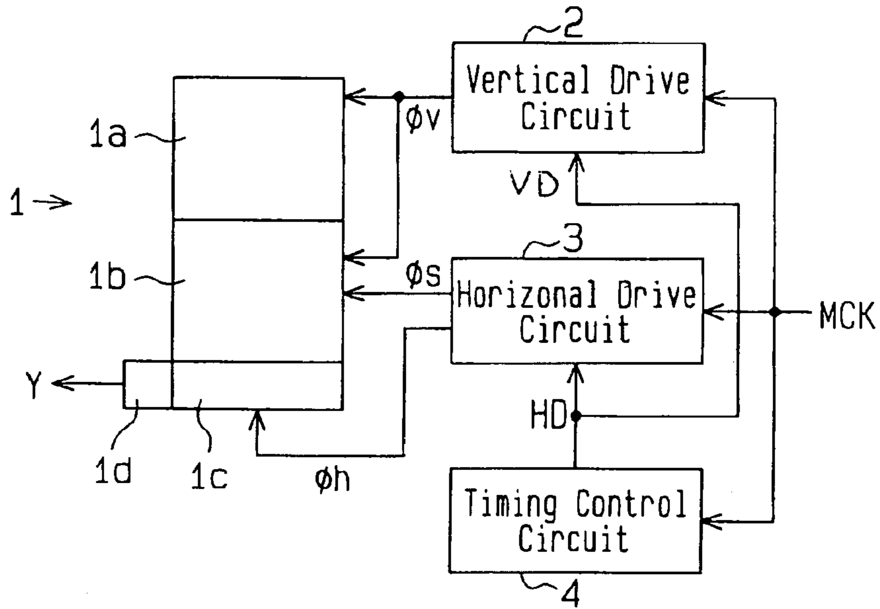
Fig.1 (Prior Art)
