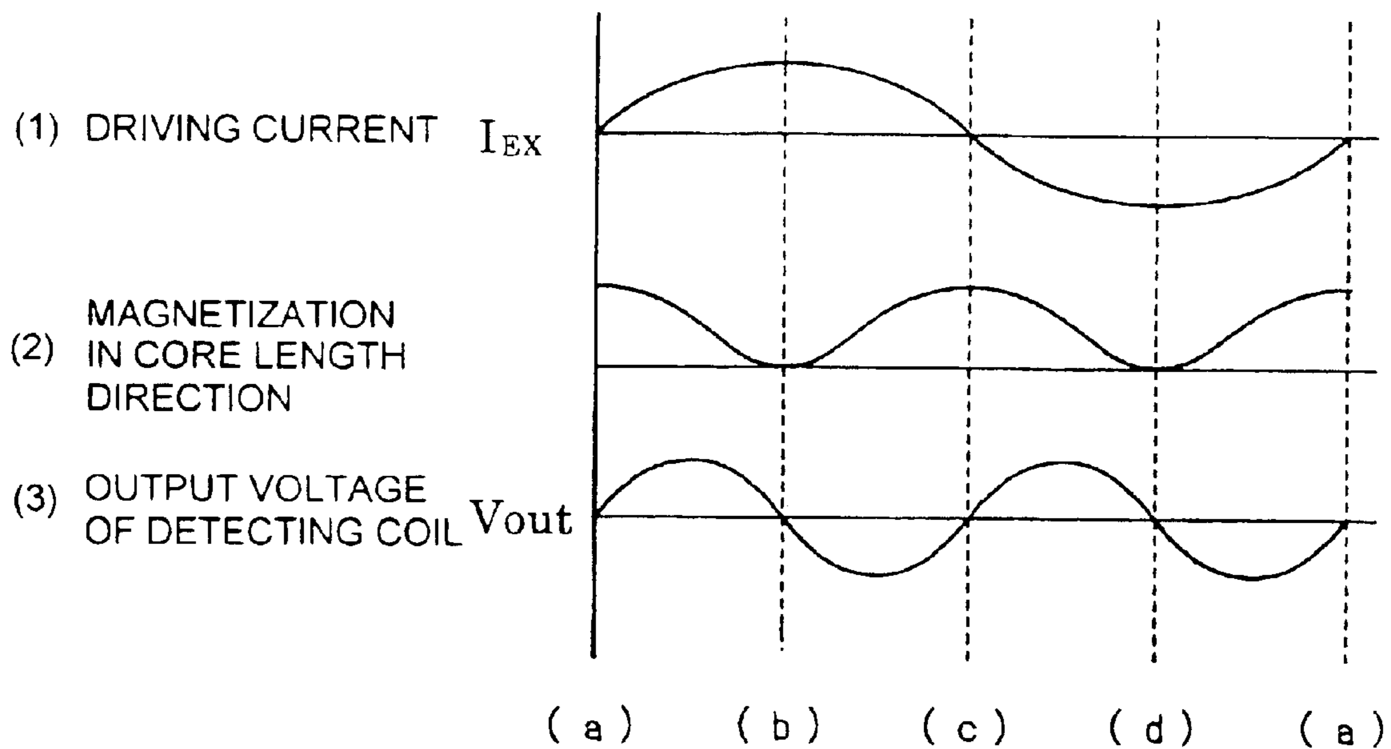
FIG. 5 (PRIOR ART)
