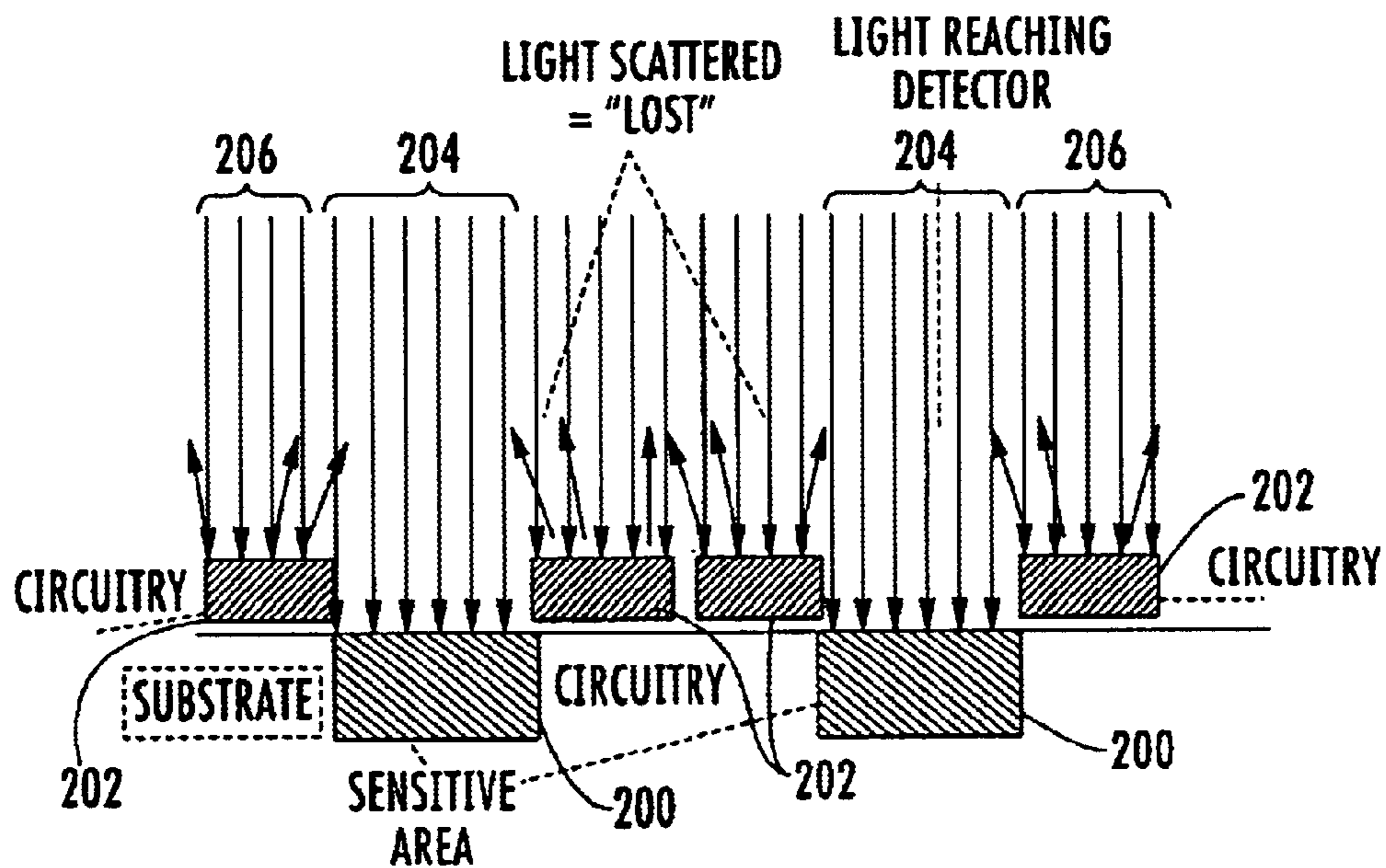
FIG. 1 (PRIOR ART)
