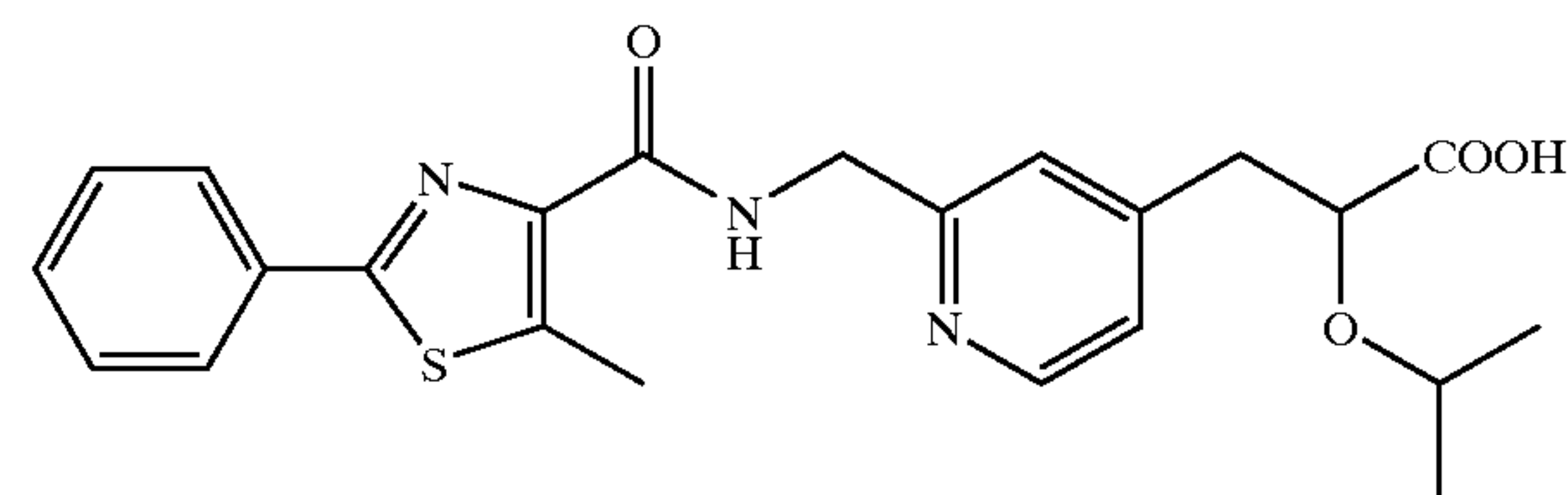
CF 3 COOH
