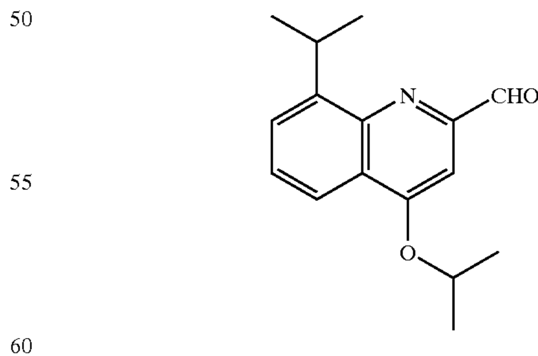
4-Isopropoxy-8-isopropylquinoxaline-2-carbaldehyde
