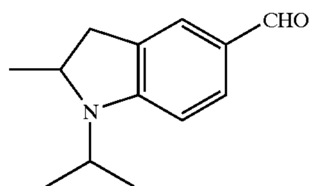
Referential Example 39 1-Isopropyl-2-methylindoline-5-carbaldehyde
