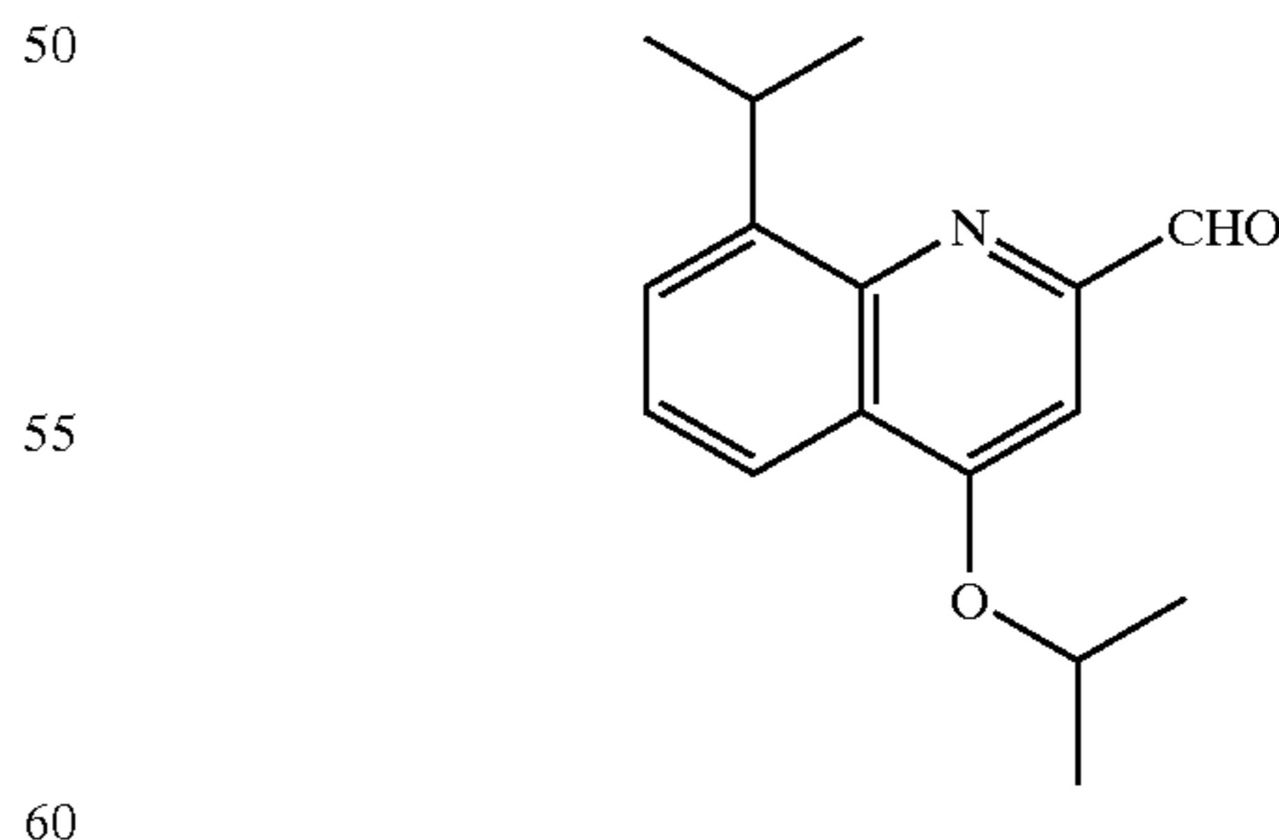
4-Isopropoxy-8-isopropylquinoxaline-2-carbaldehyde
