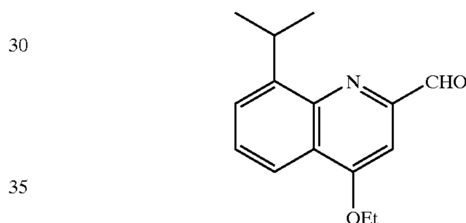
4-Ethoxy-8-isopropylquinoxaline-2-carbaldehyde
