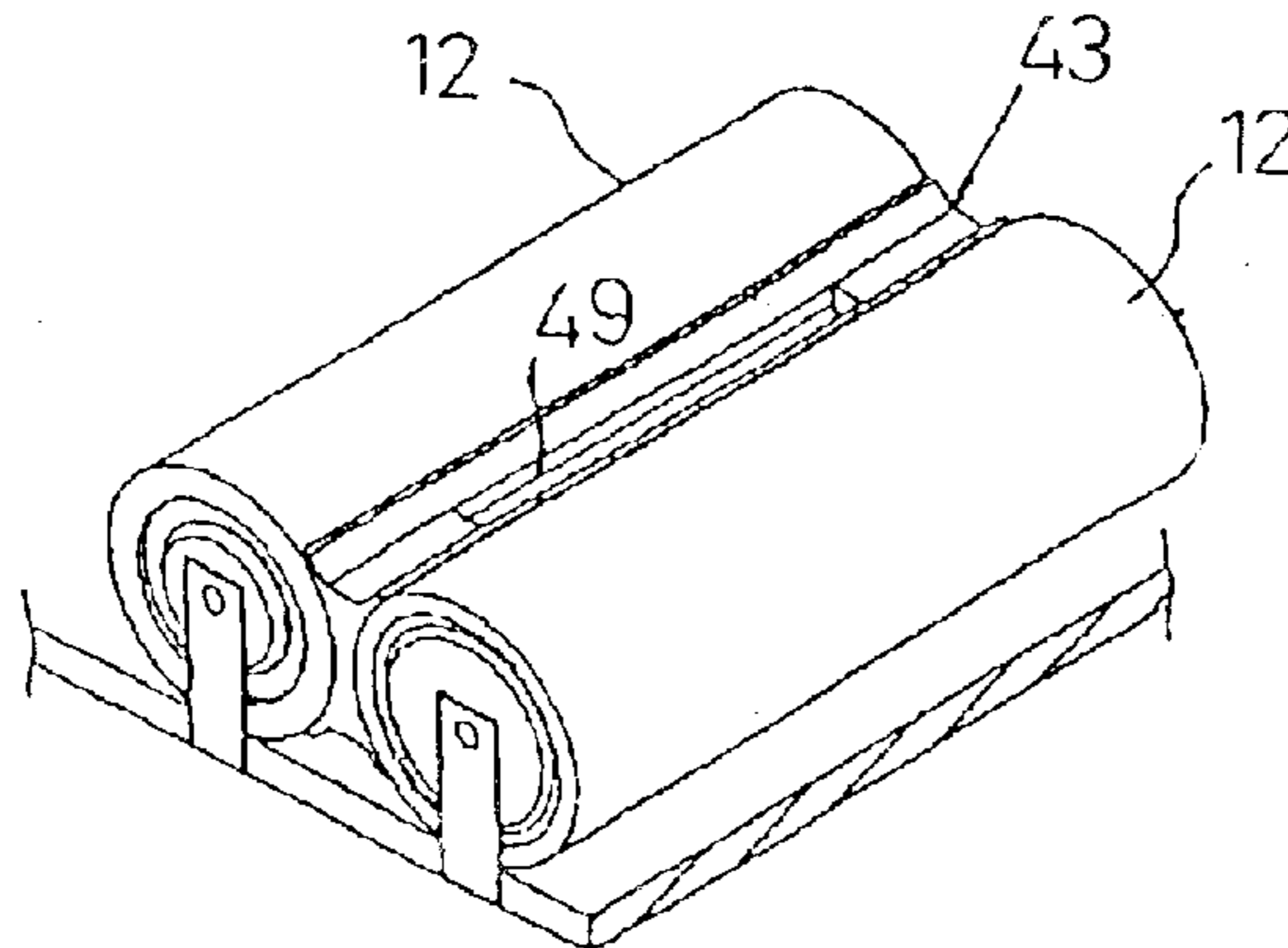
Fig. 11 Prior Art
