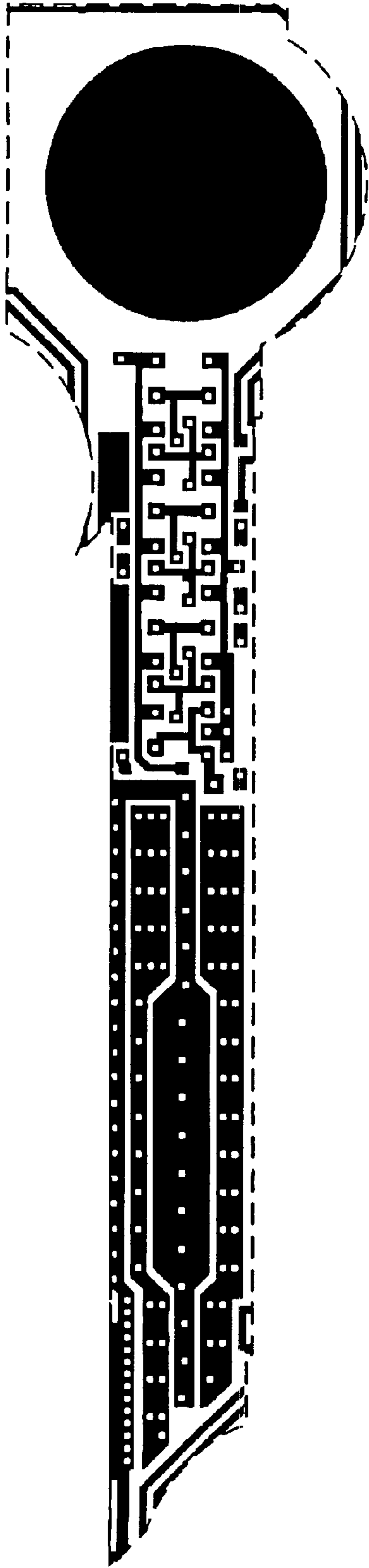
Metal 1 mask
