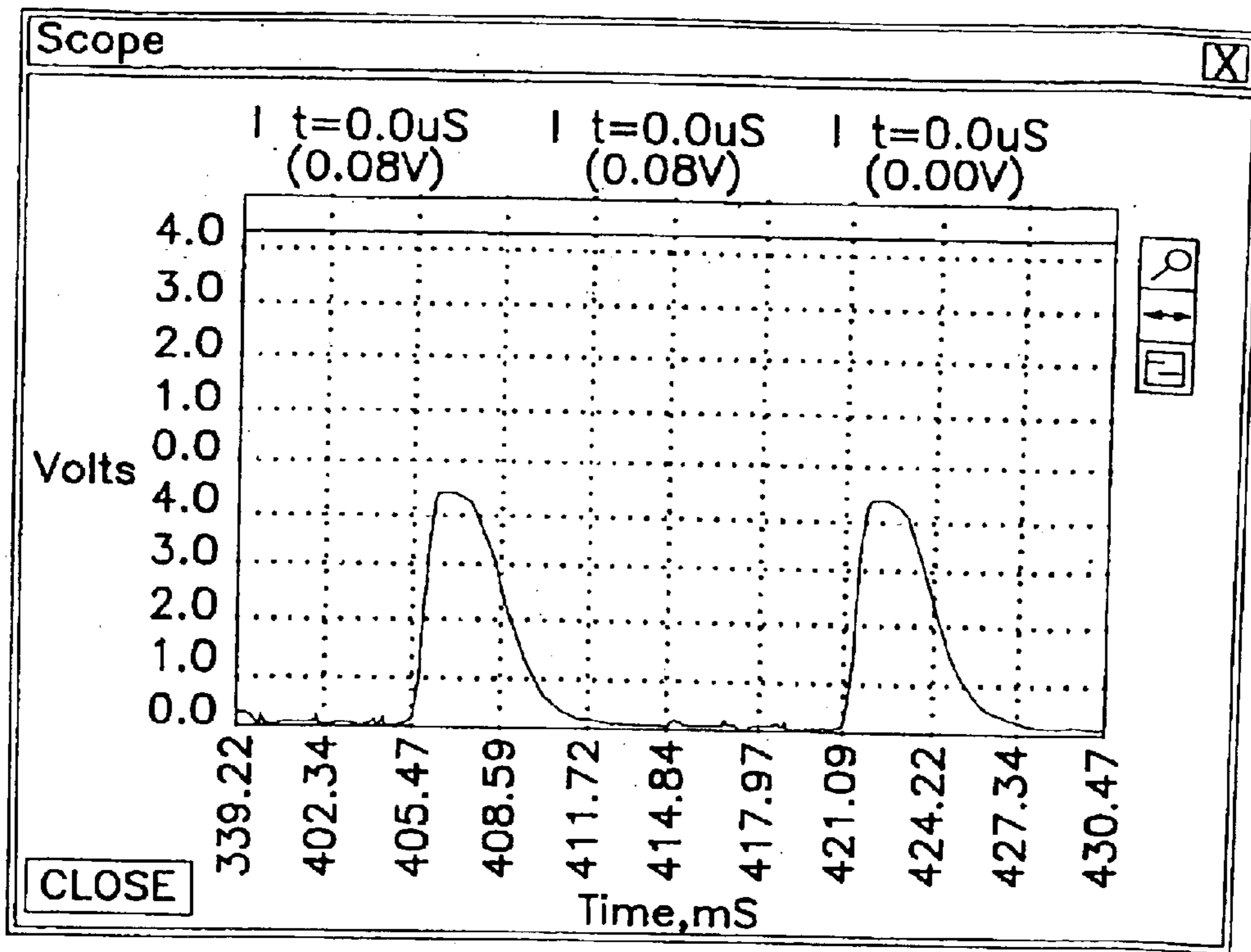
CRT photoresponse
