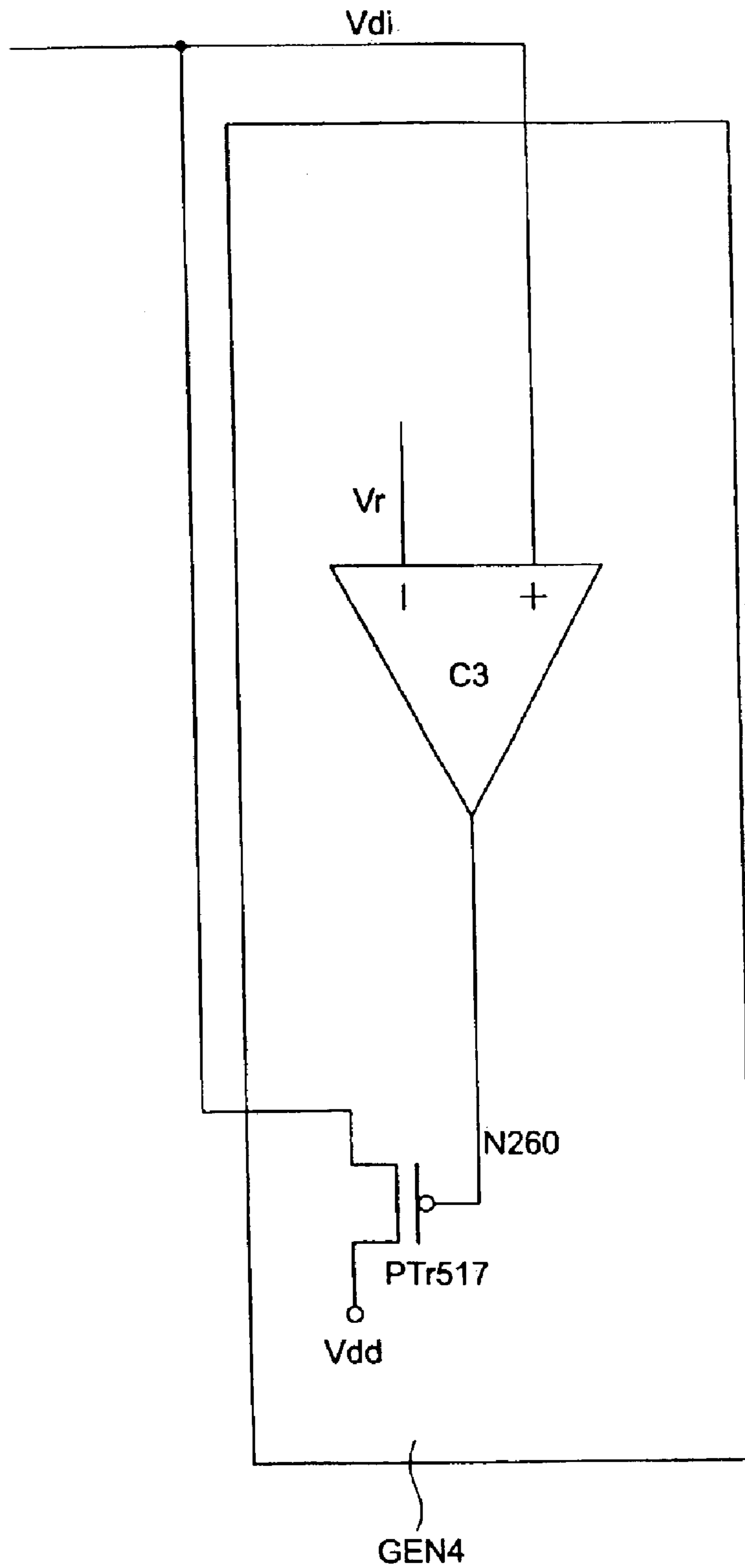
FIG. 8 PRIOR ART
