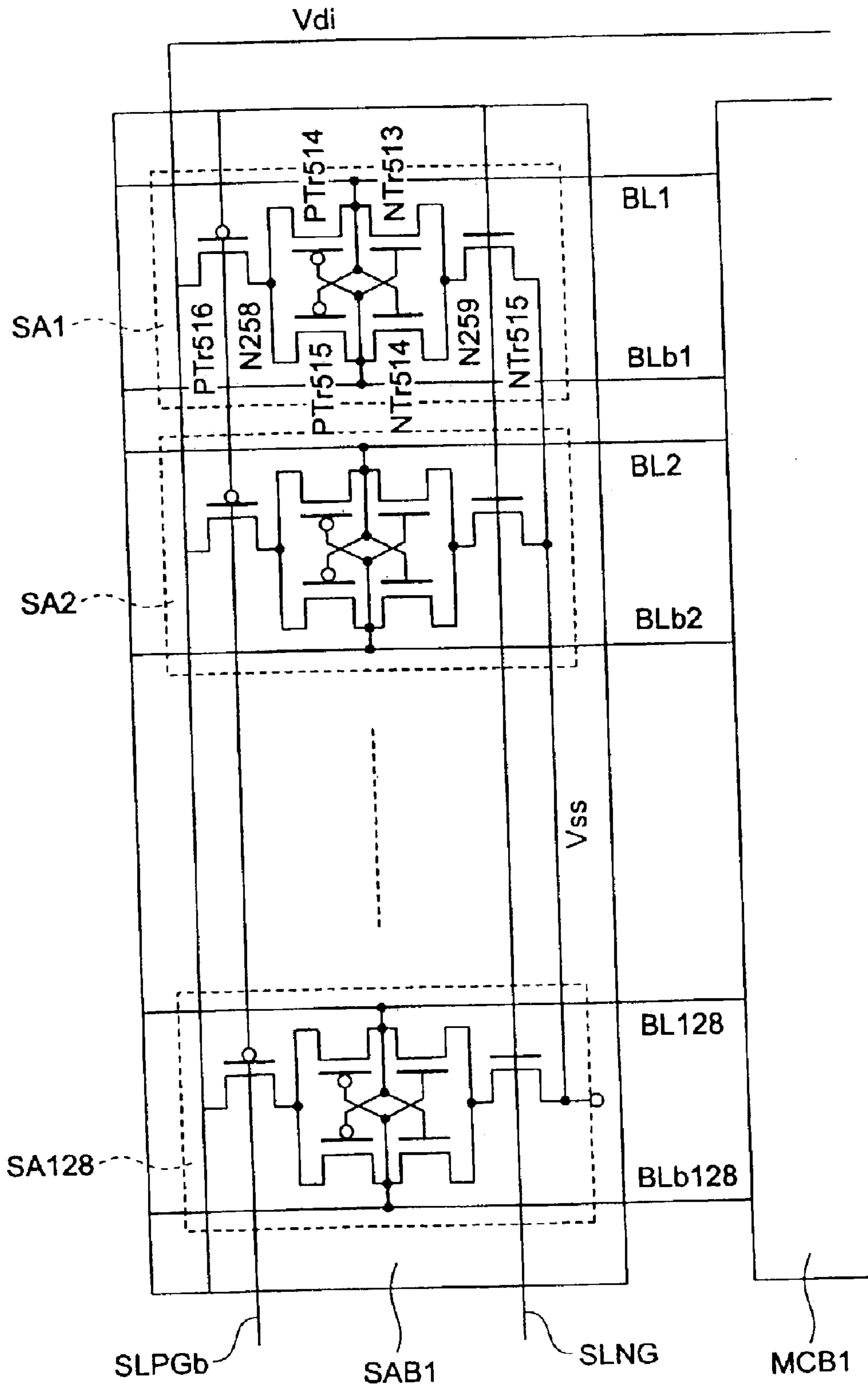
FIG. 7 PRIOR ART
