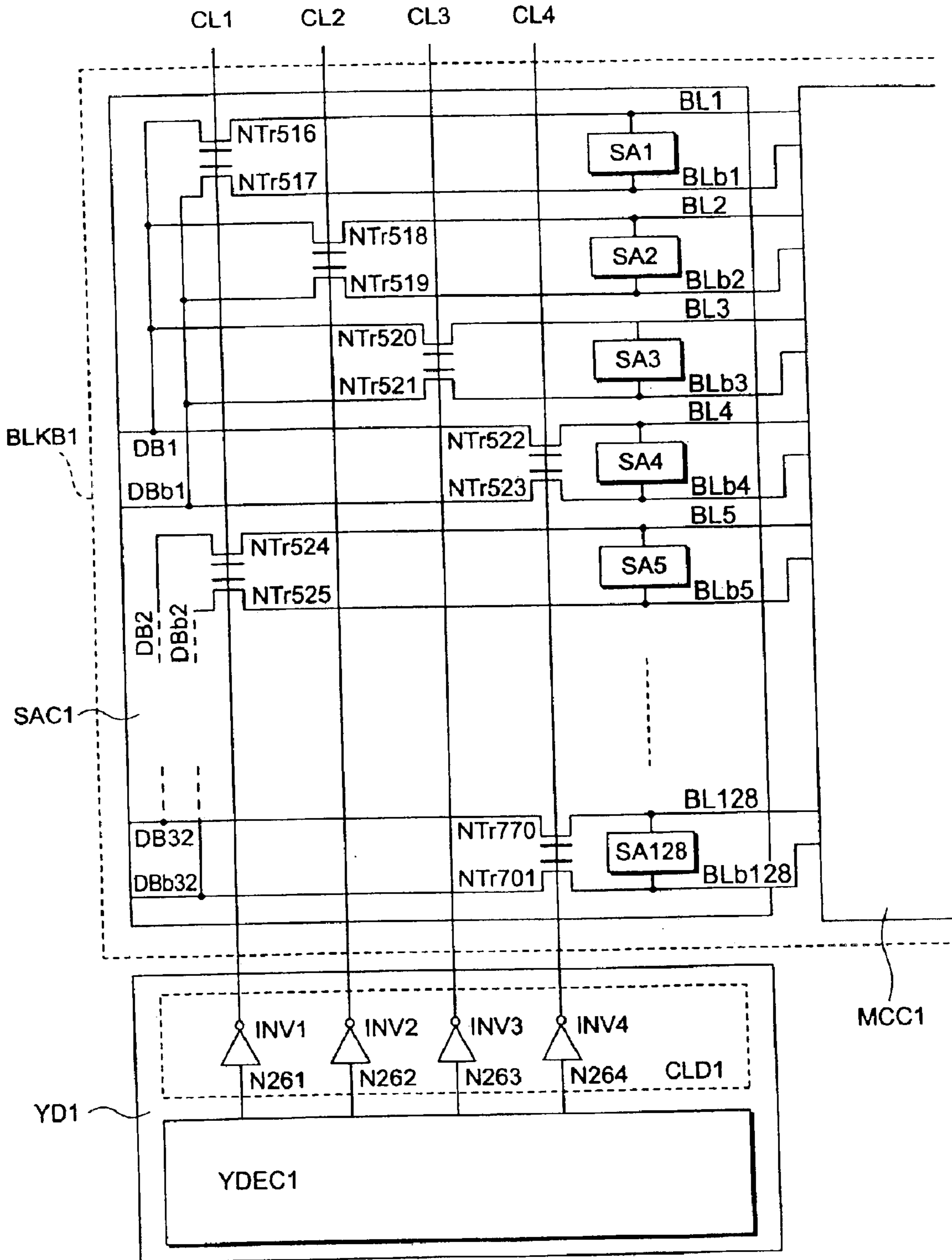
FIG. 10 PRIOR ART
