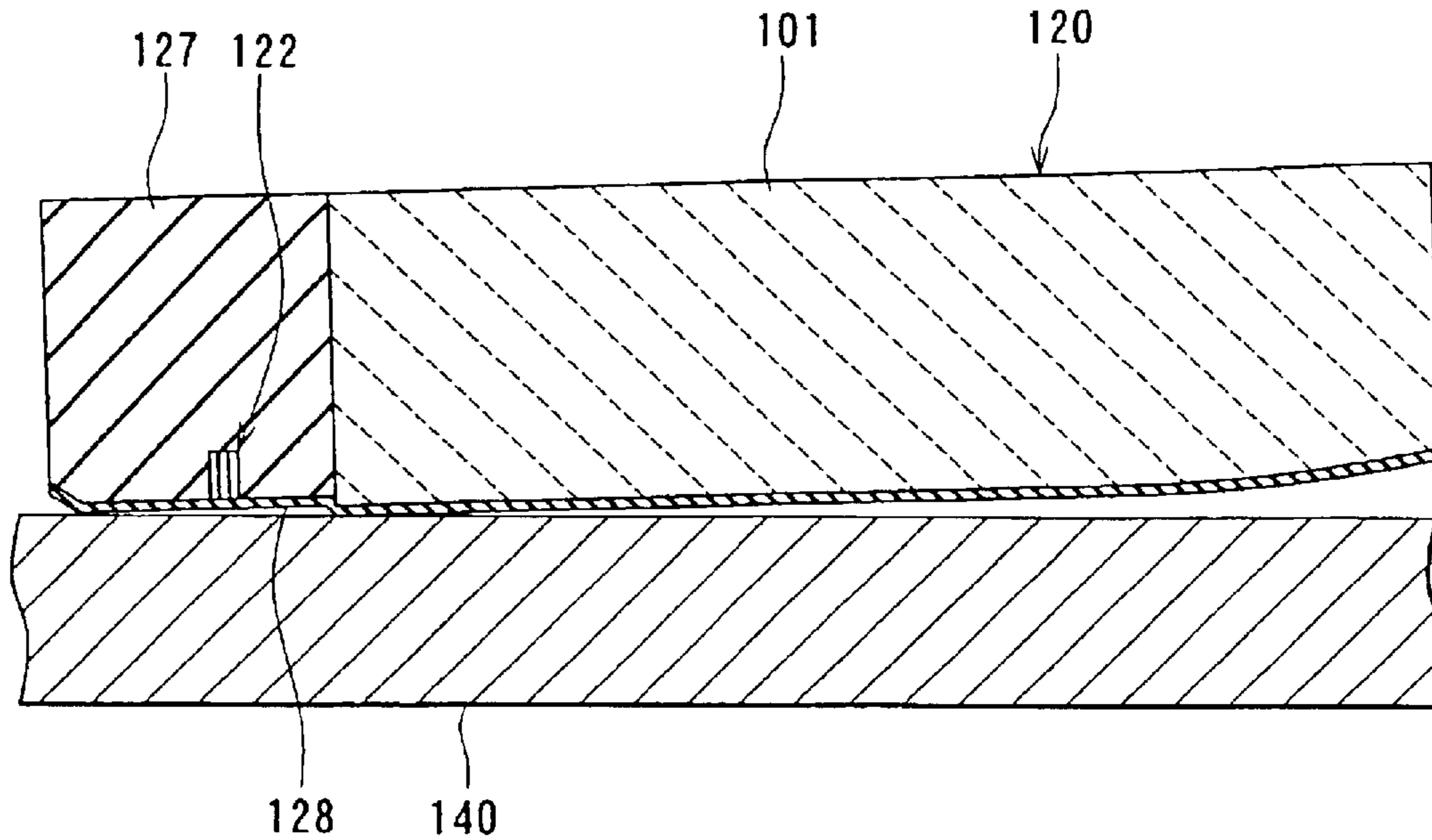
FIG. 41 RELATED ART
