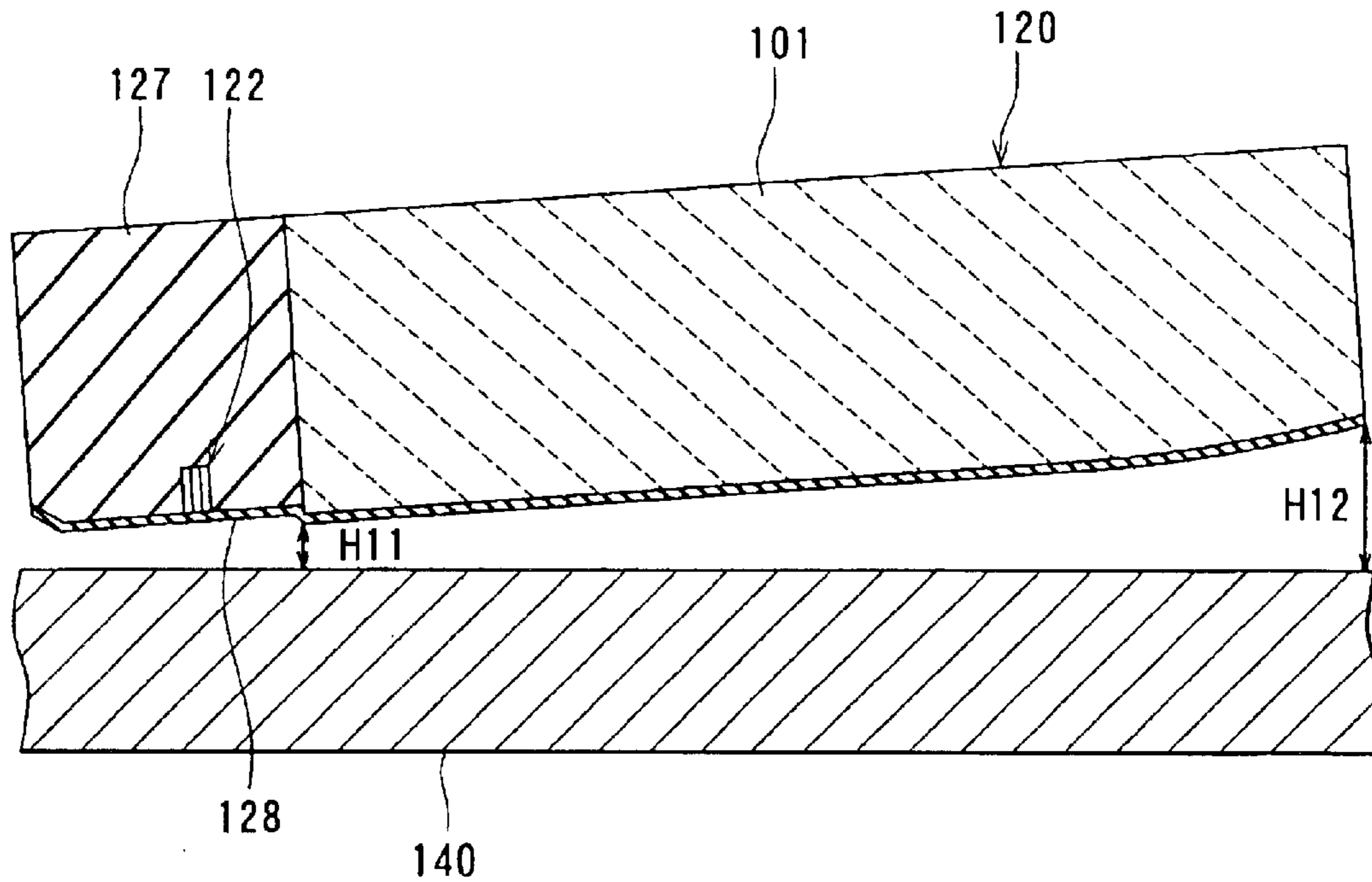
FIG. 42 RELATED ART
