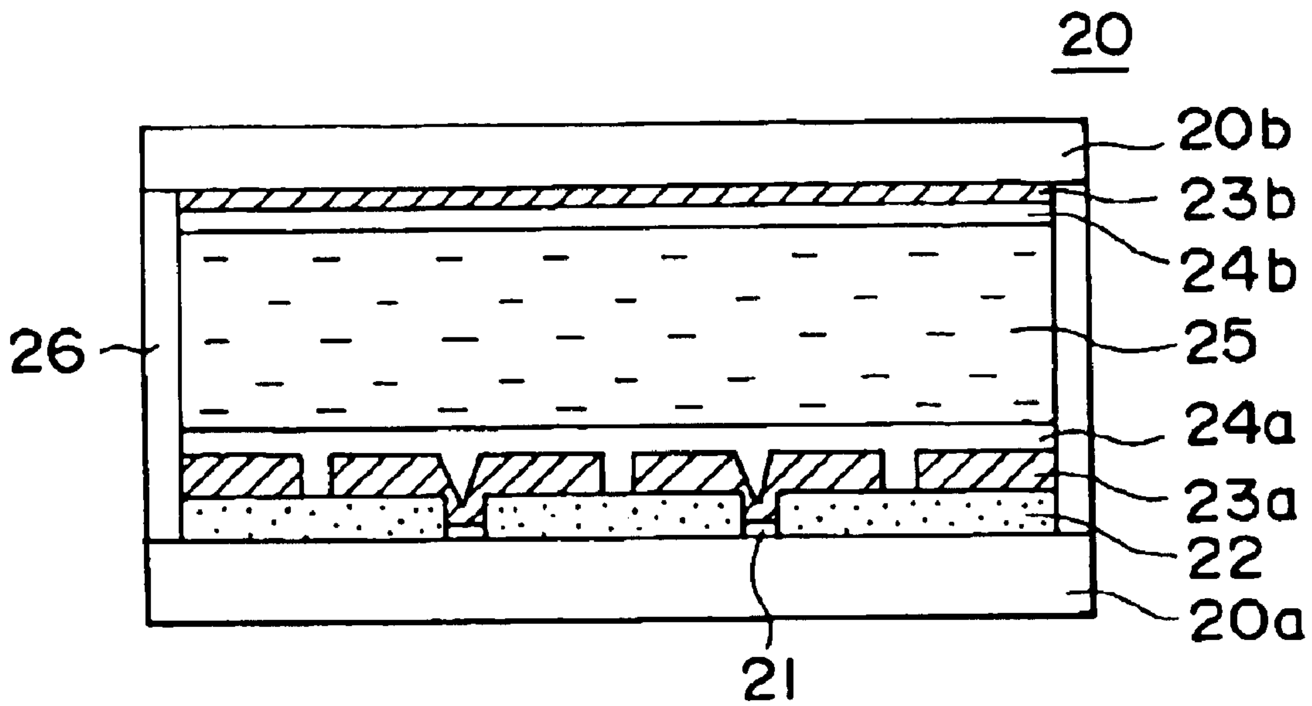
FIG.15 PRIOR ART
