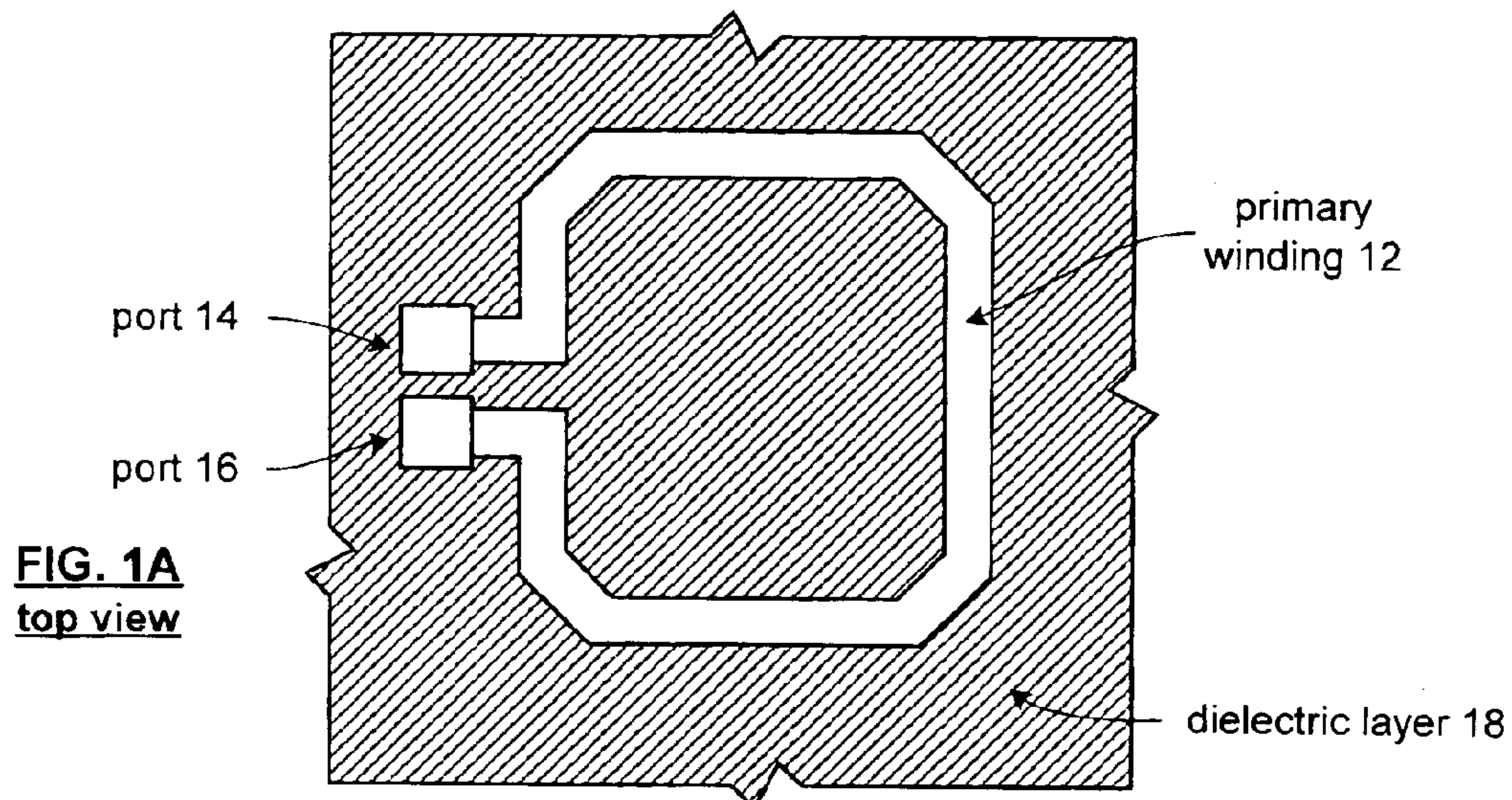
on-chip transformer 10
