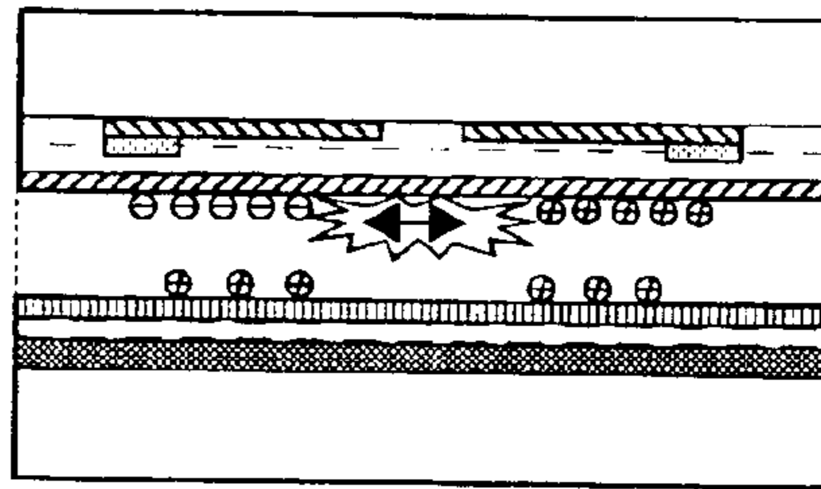
FIG. 19D (PRIOR ART)
