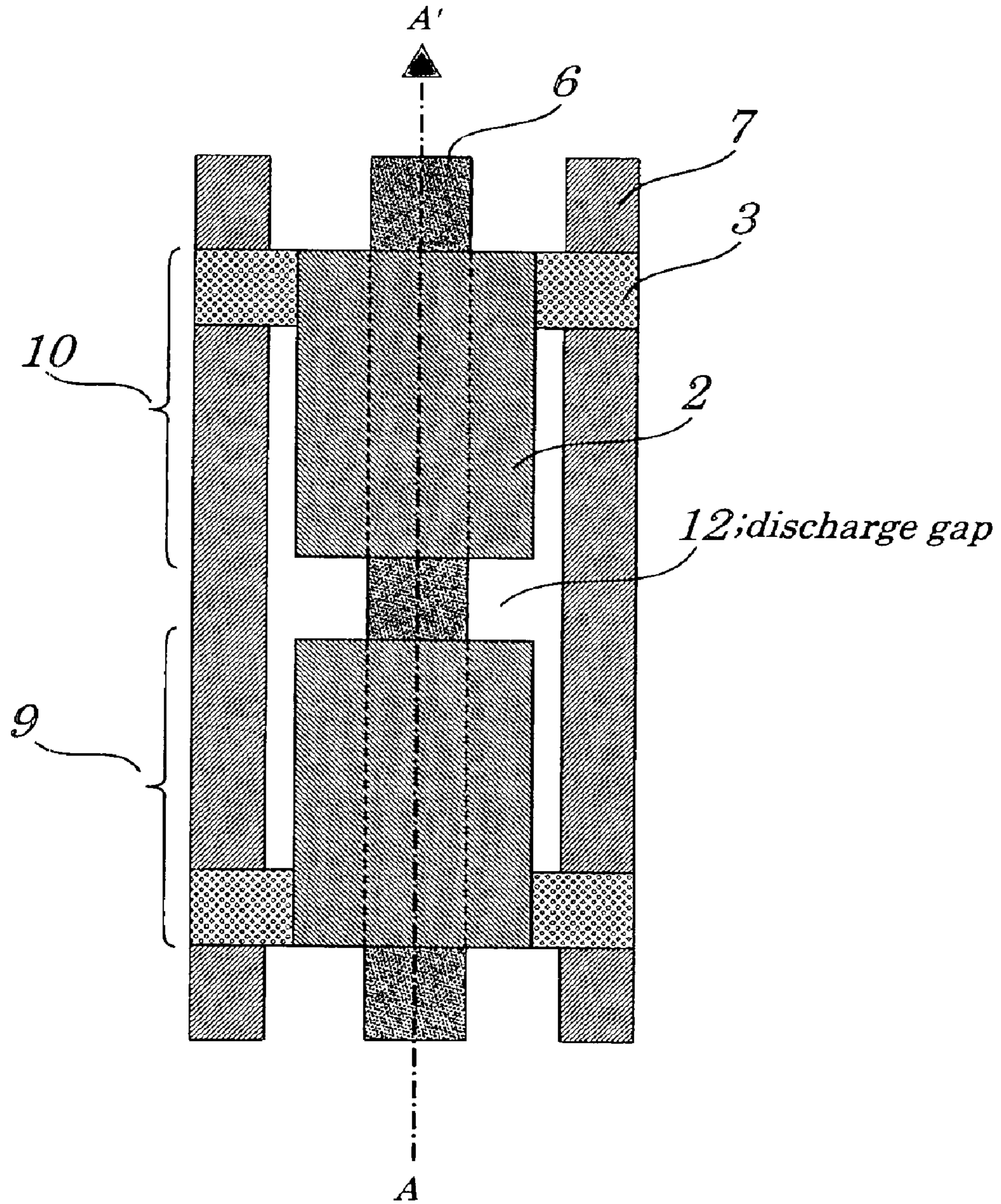
FIG. 16 (PRIOR ART)
