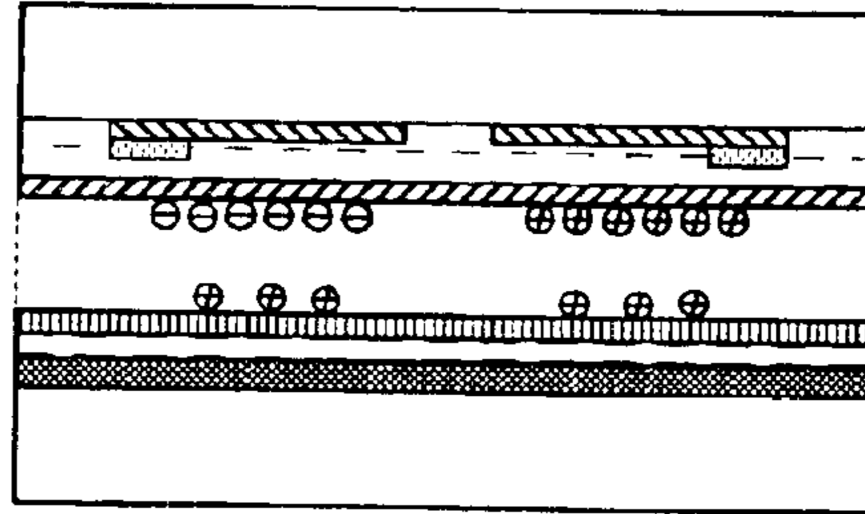
FIG. 20C (PRIOR ART)
