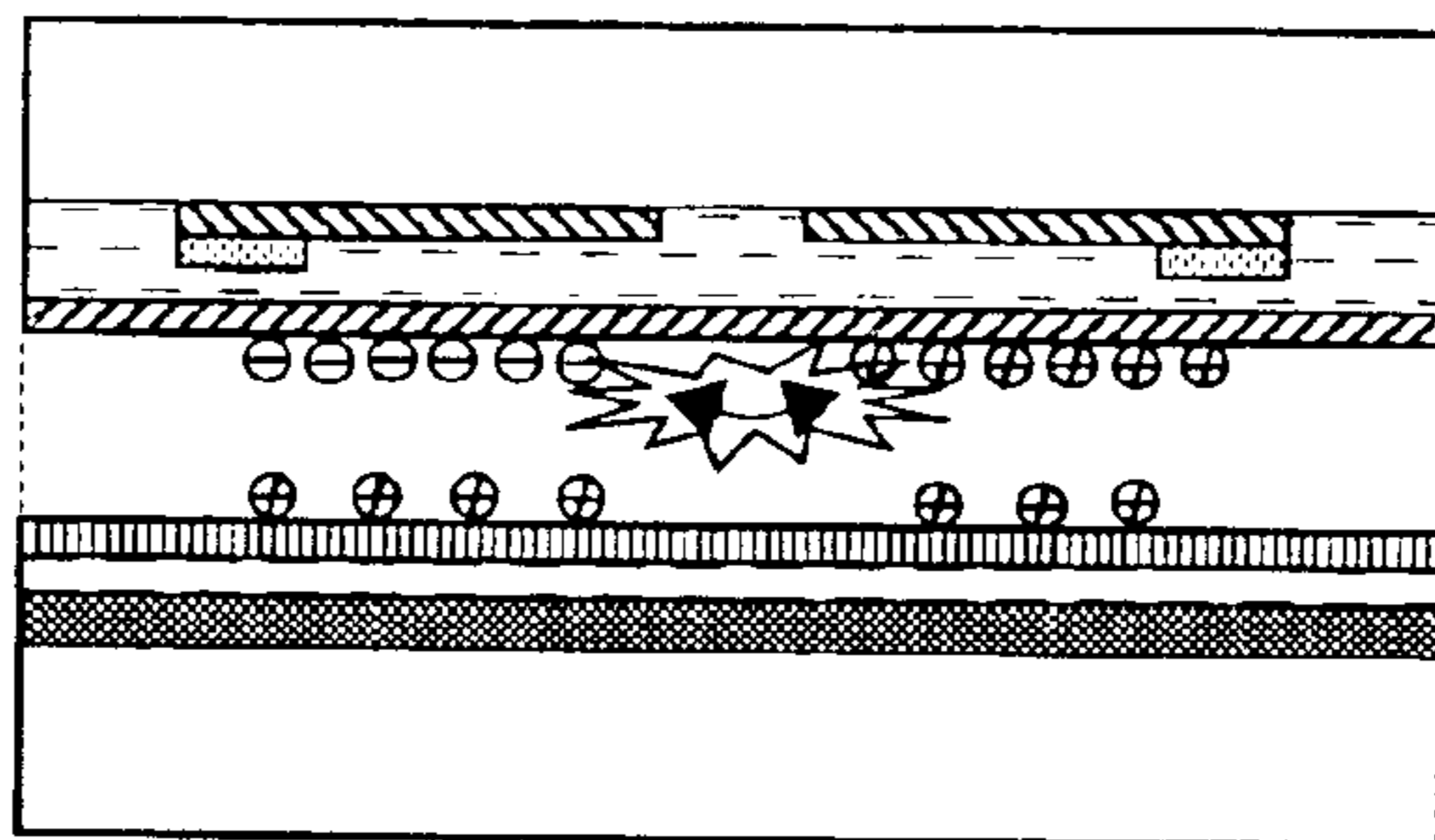
FIG. 22C (PRIOR ART)
