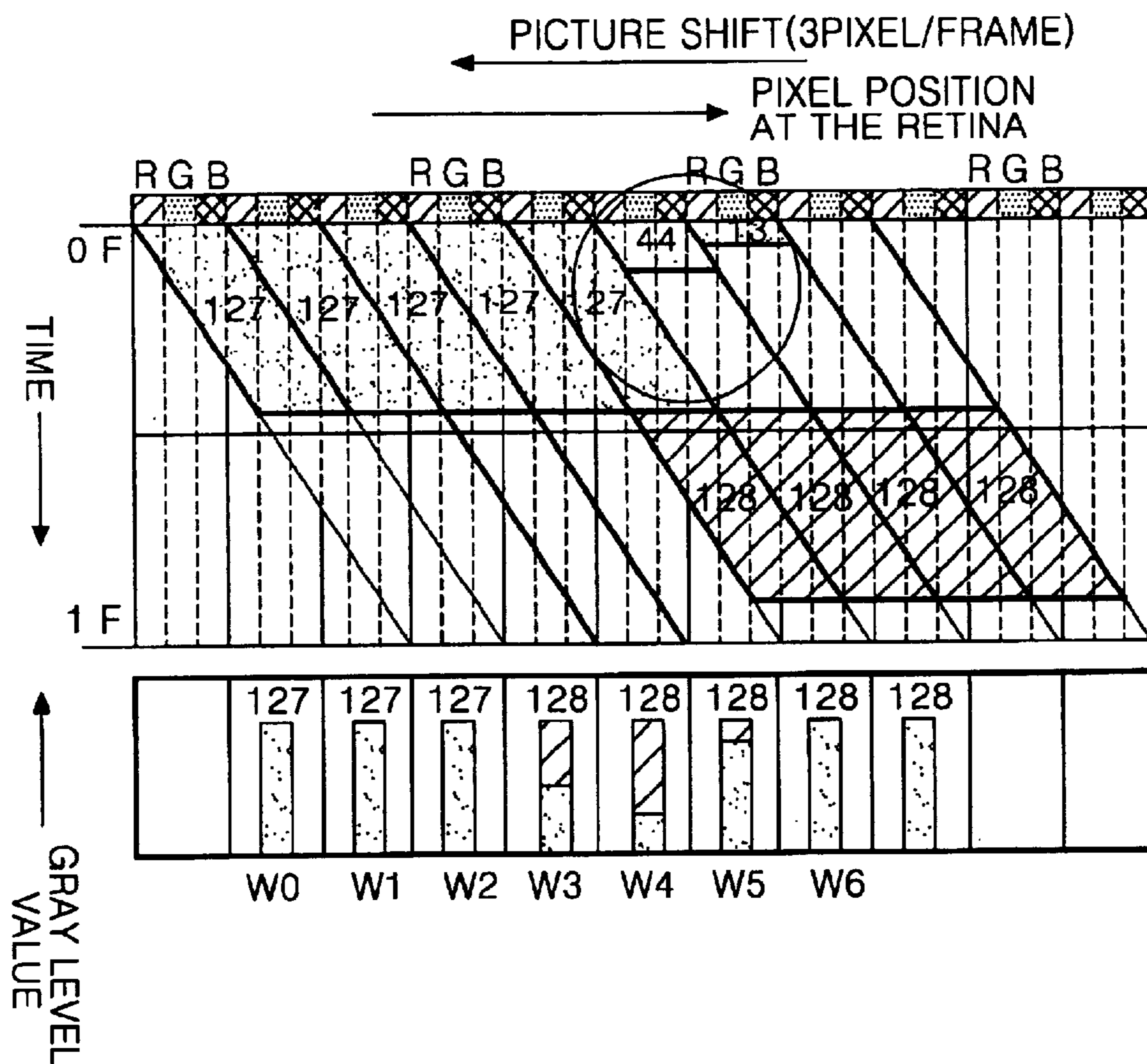
FIG. 3 RELATED ART
