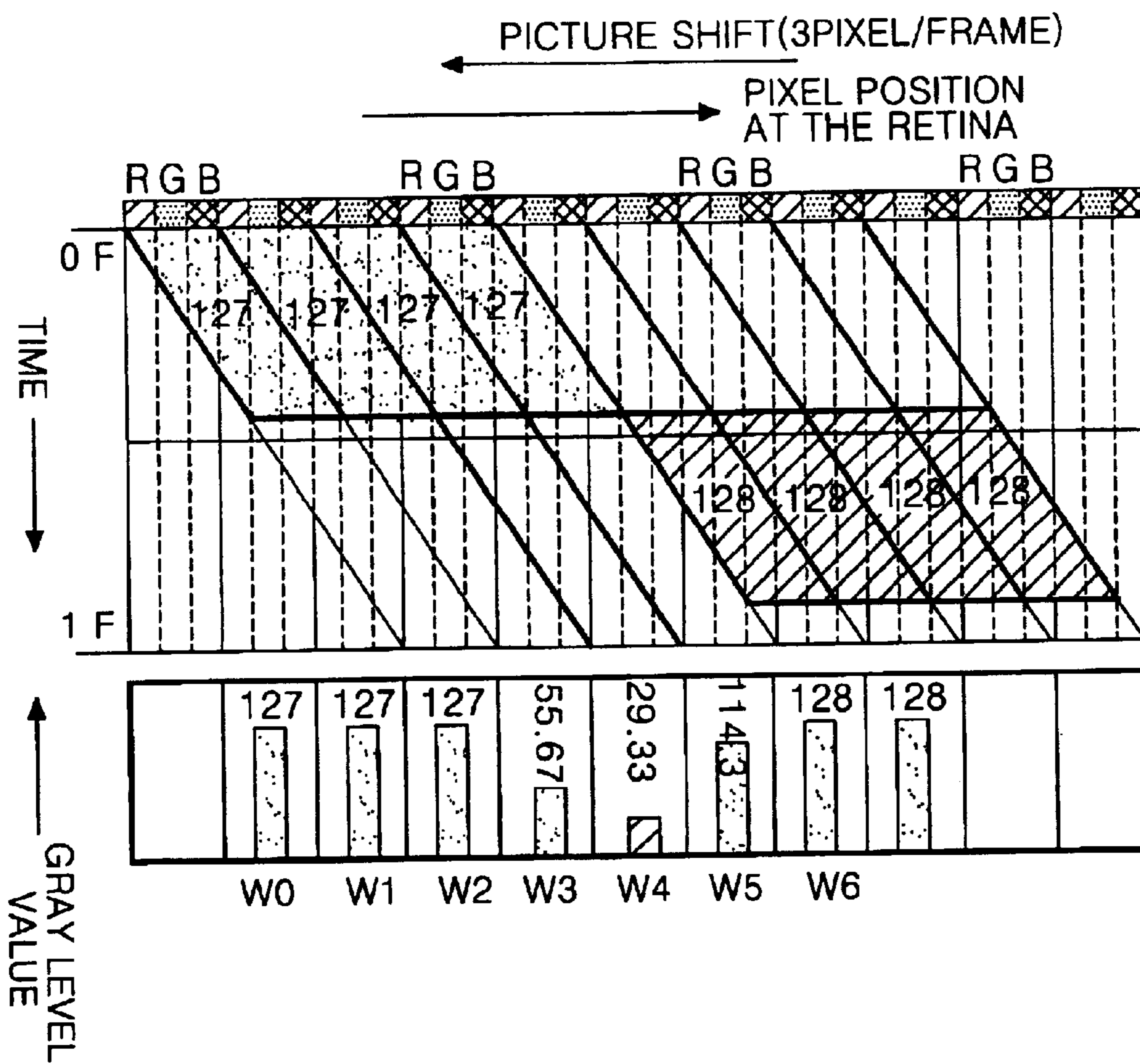
FIG. 2 RELATED ART
