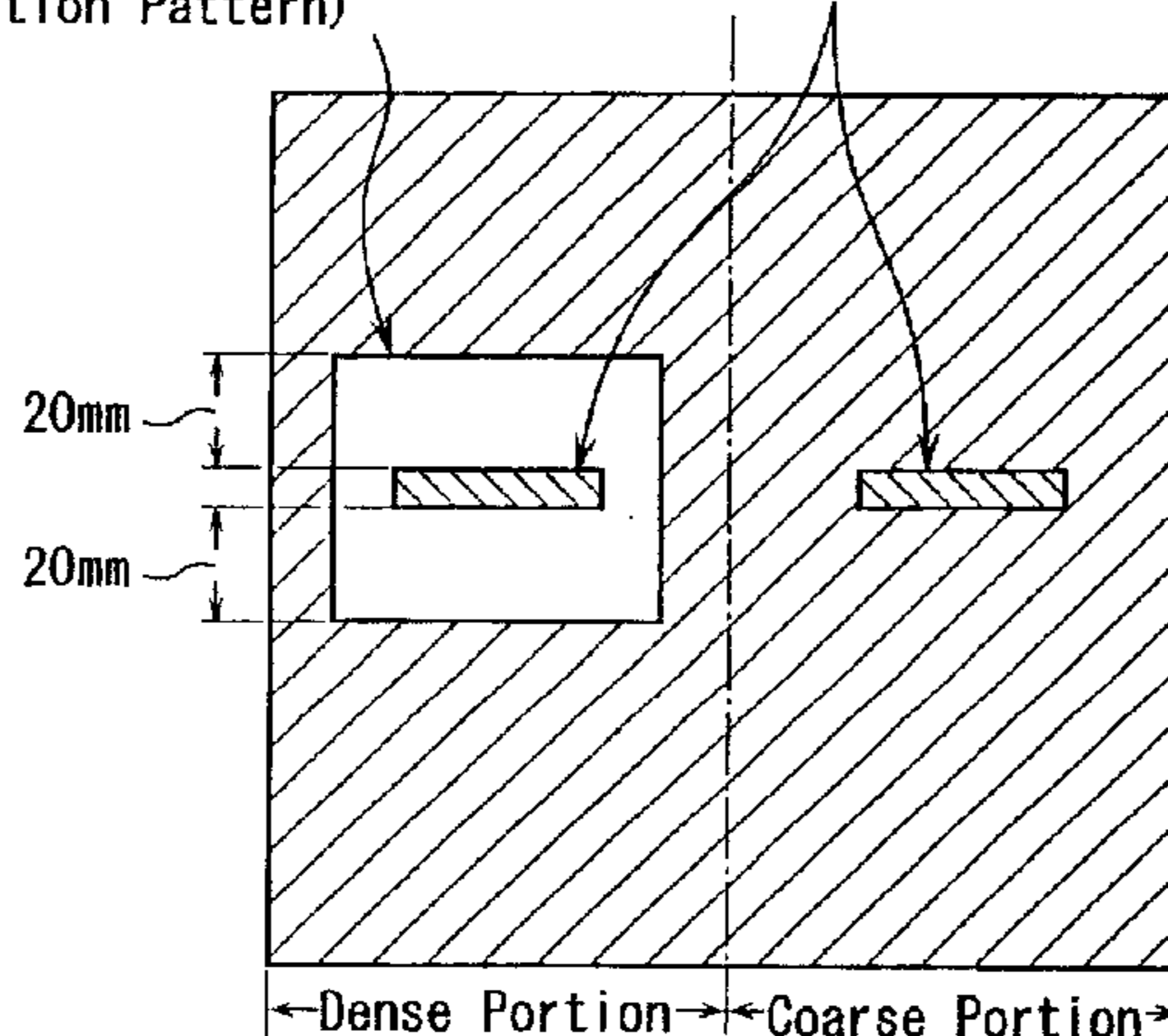
Completely Removed Pattern Dimension-Evaluation Pattern (Periphery of the Dimension-Evaluation Pattern) (L/S, Isolated L, Isolated S)
