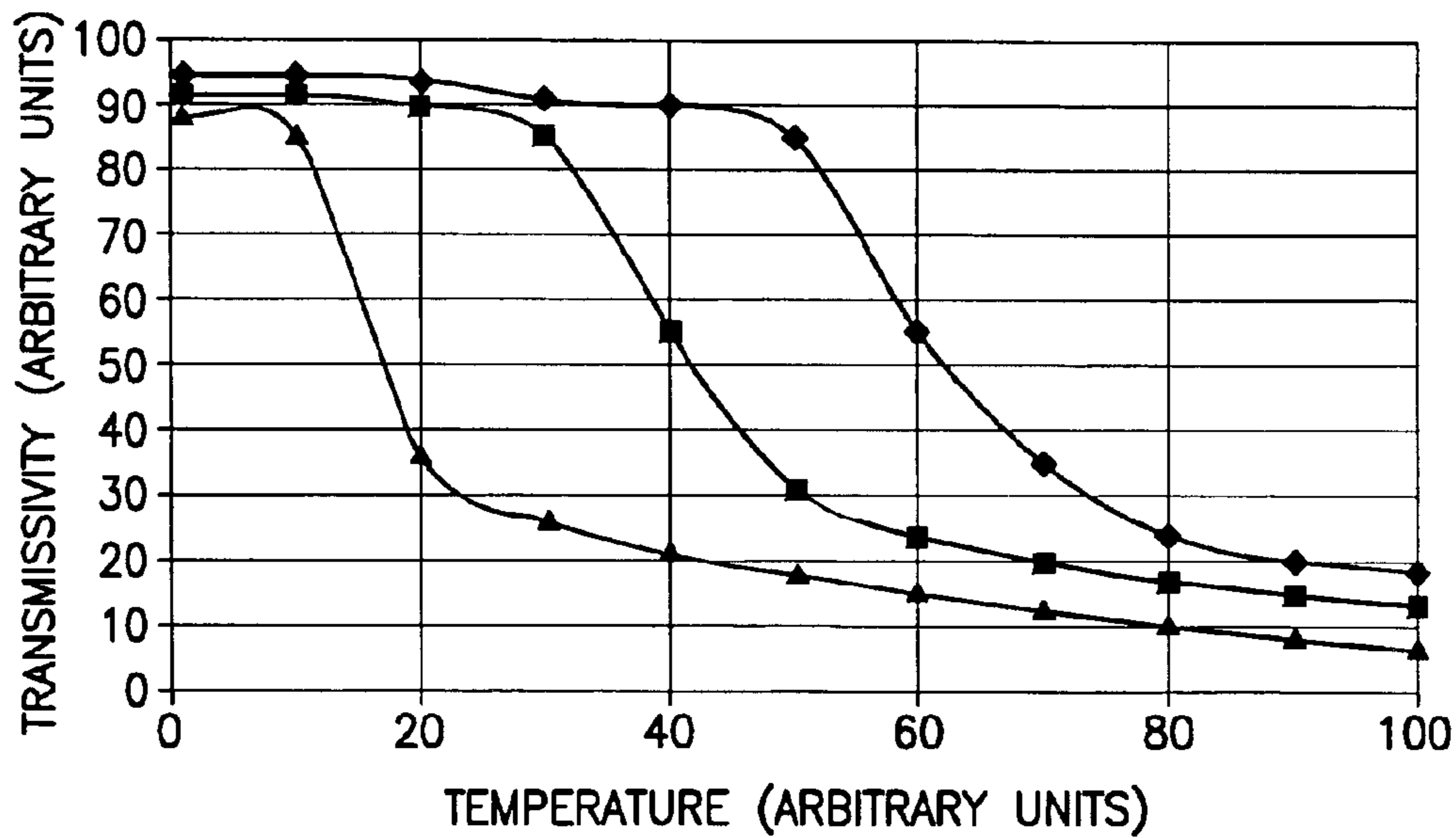
RESPONSE FUNCTION FOR THREE THERMOCHROMIC MATERIALS
