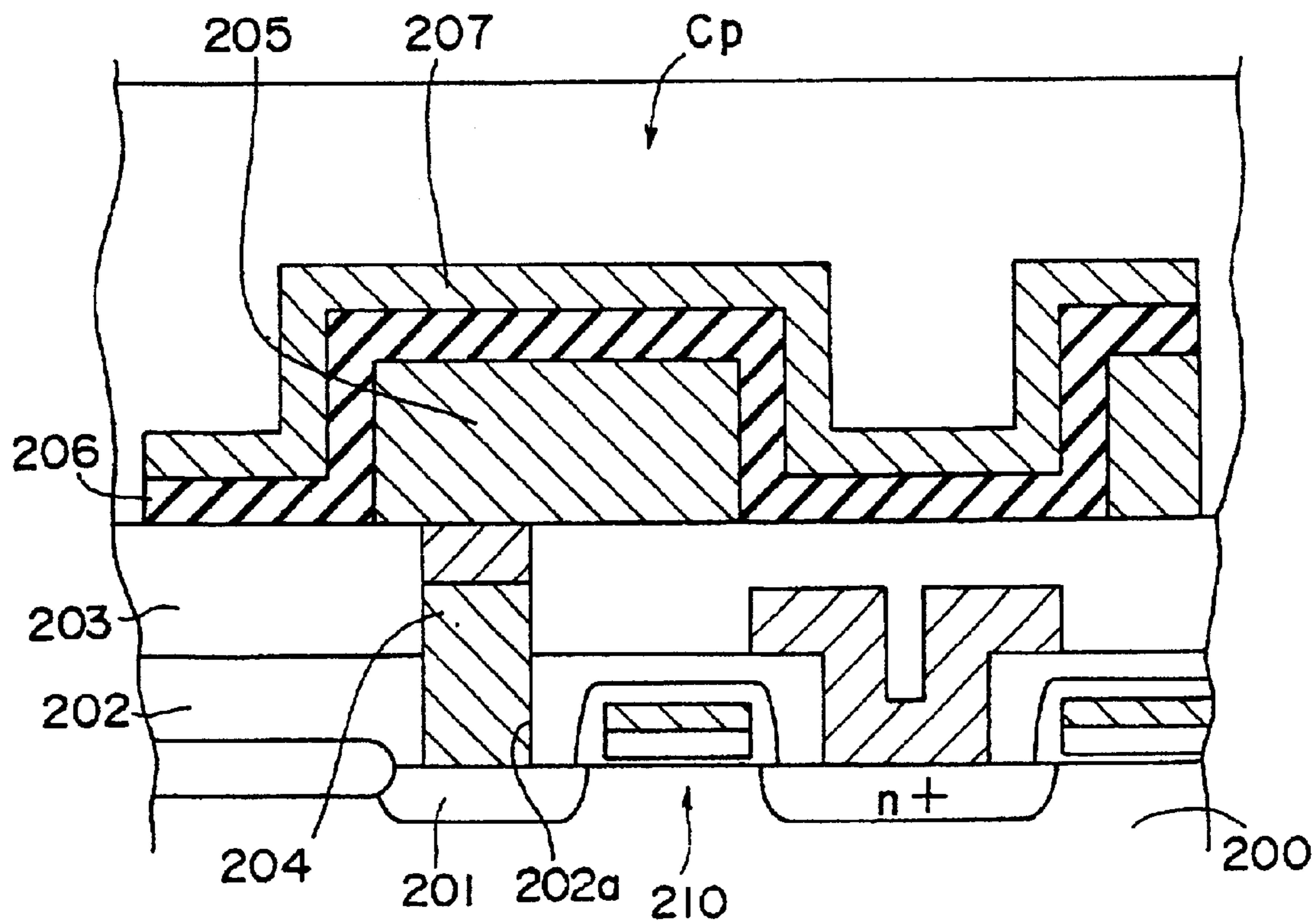
Fig. 4 PRIOR ART
