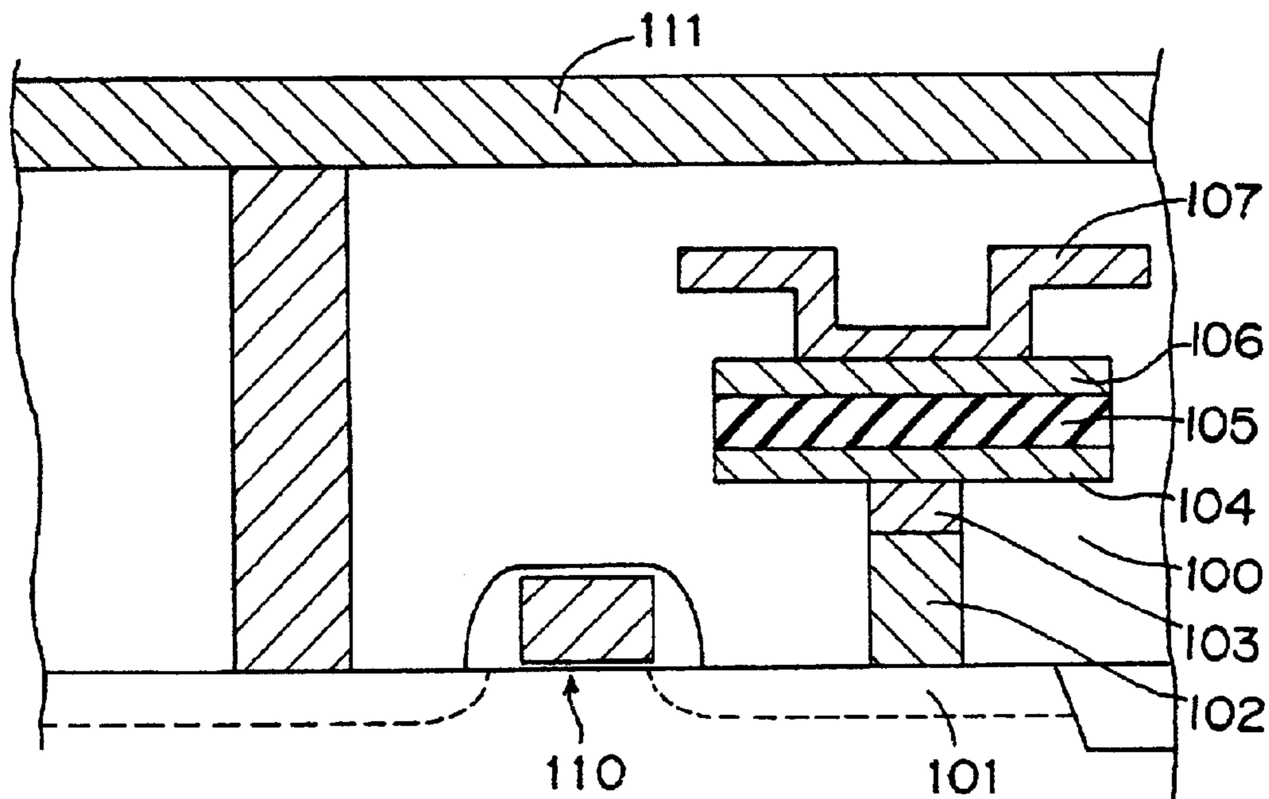
Fig. 4 PRIOR ART
