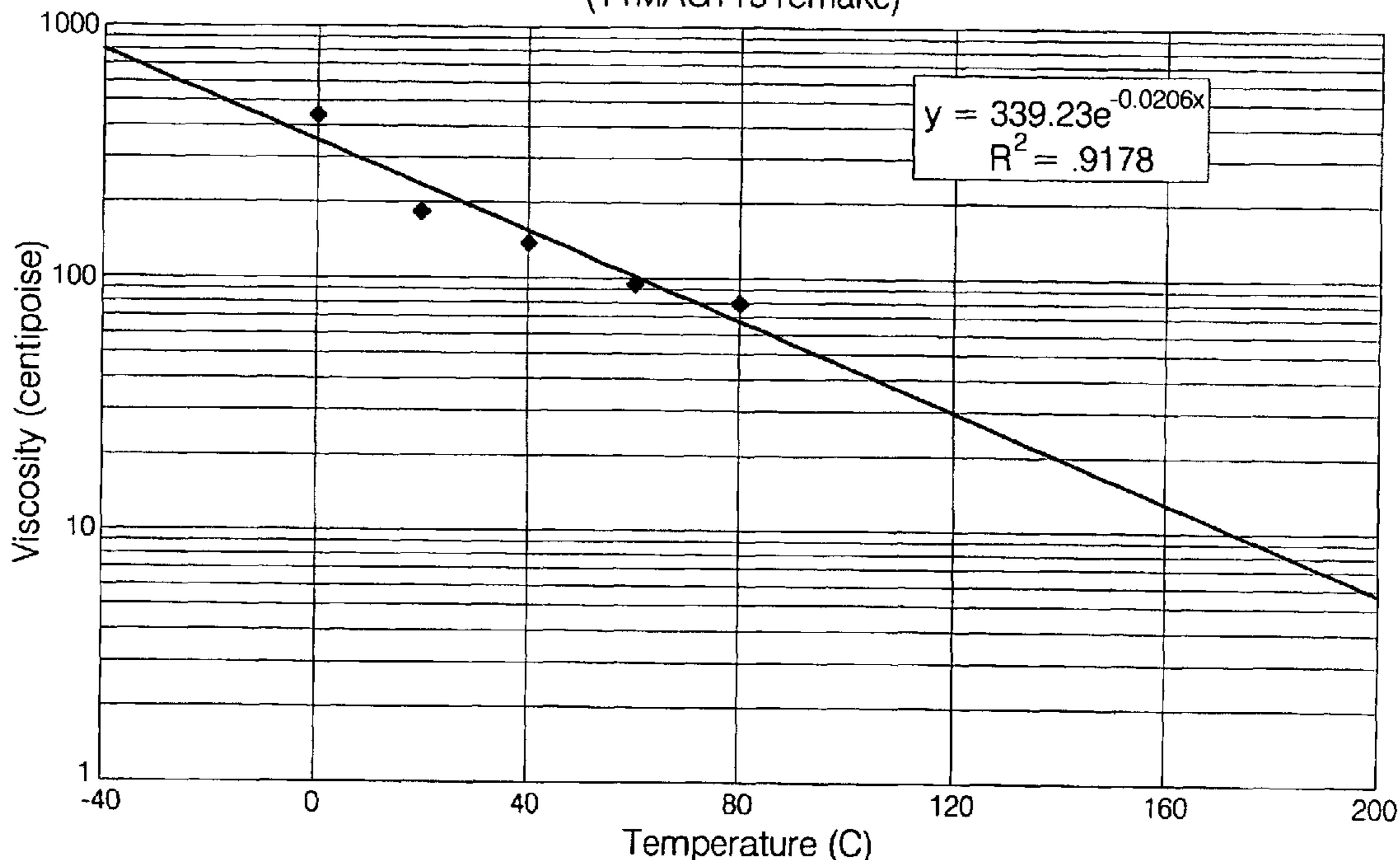
Viscosity versus Temperature for 12MAG001 (11MAG115 remake)
