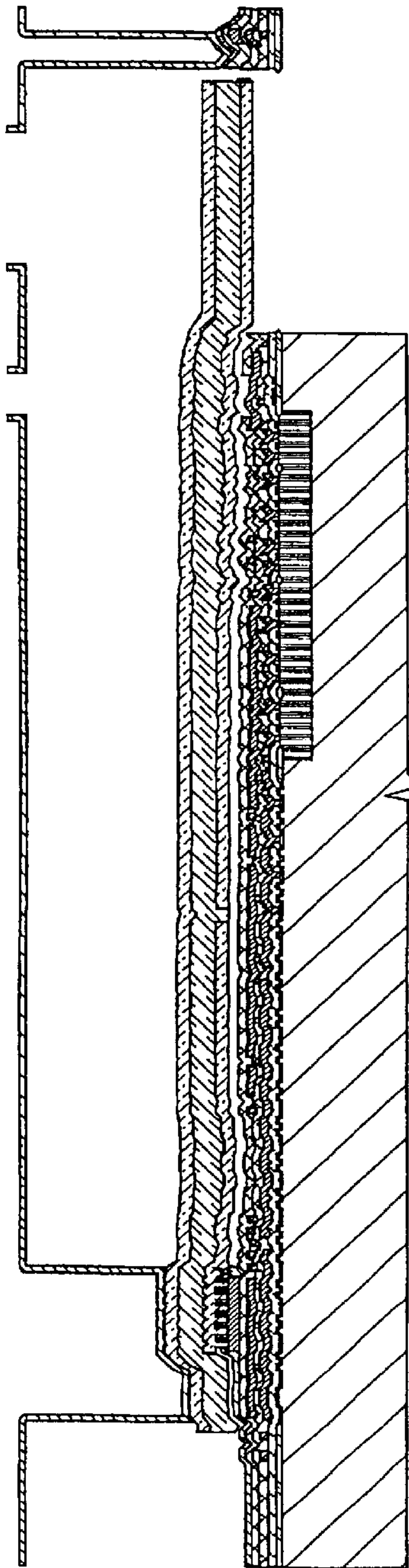
Detach from wafer blank, etch sacrificial material
