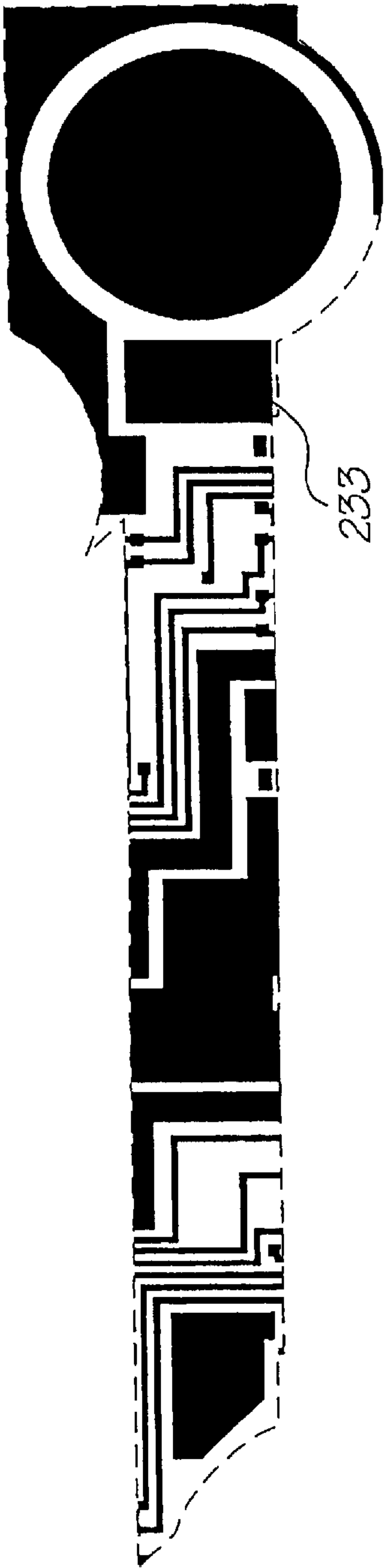
Metal 2 mask
