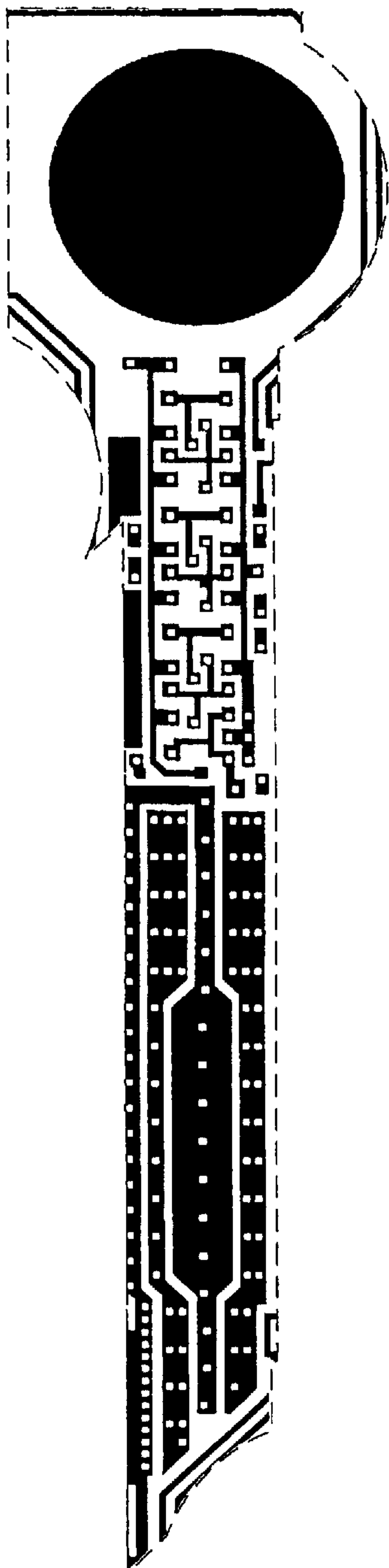
Metal 1 mask
