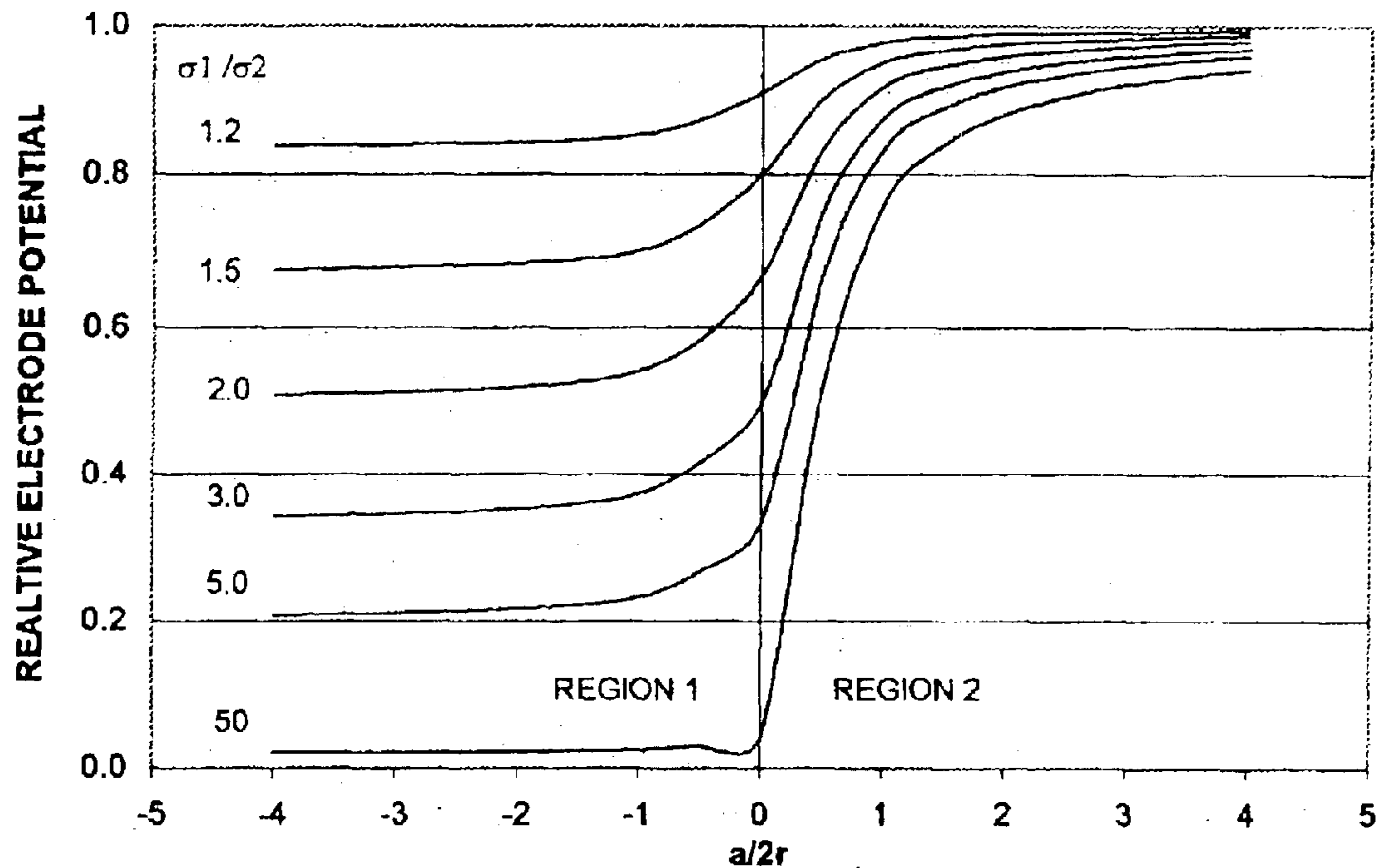
FIG.7A SPHERICAL ELECTRODE
