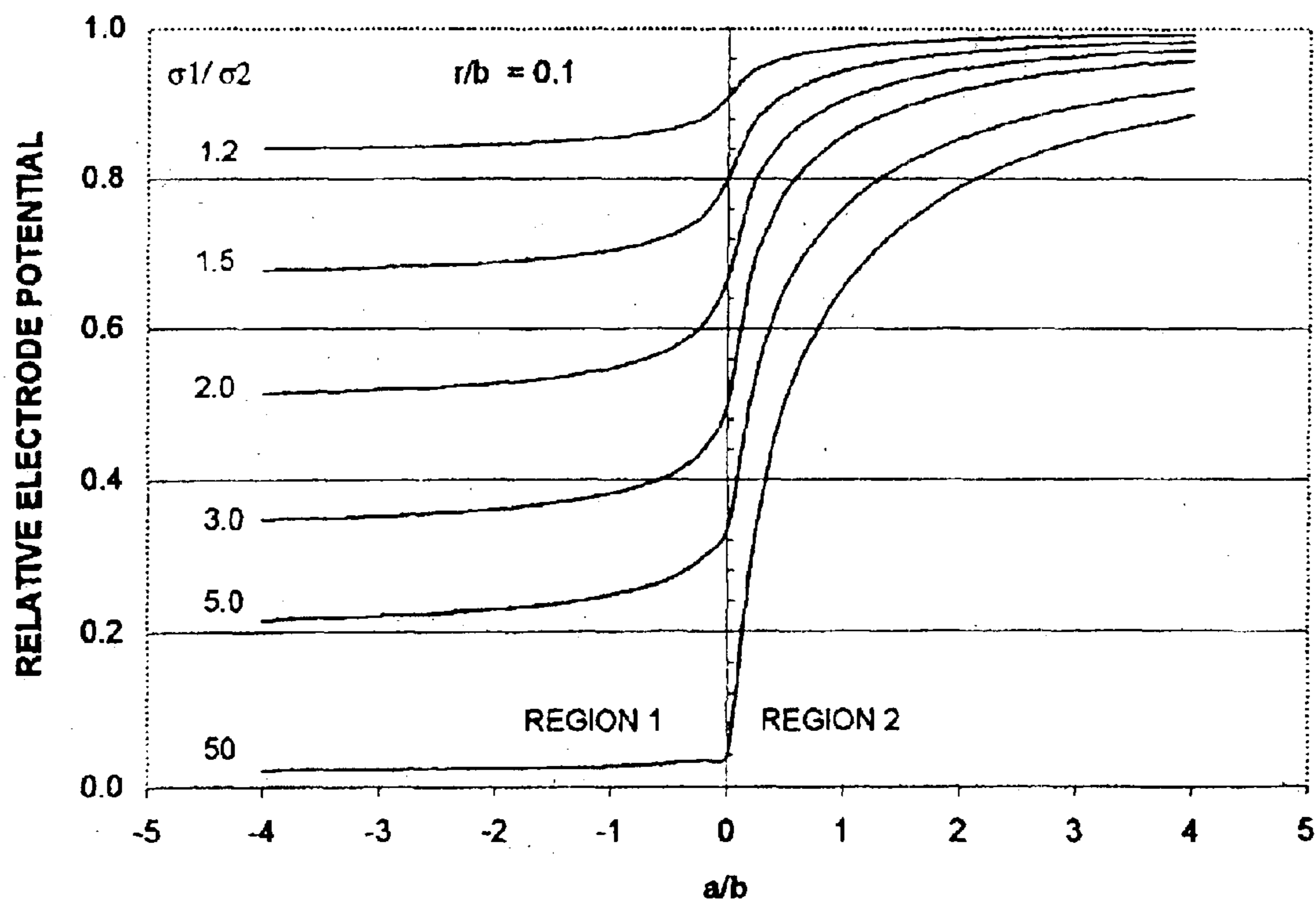
FIG.7B RING ELECTRODE
