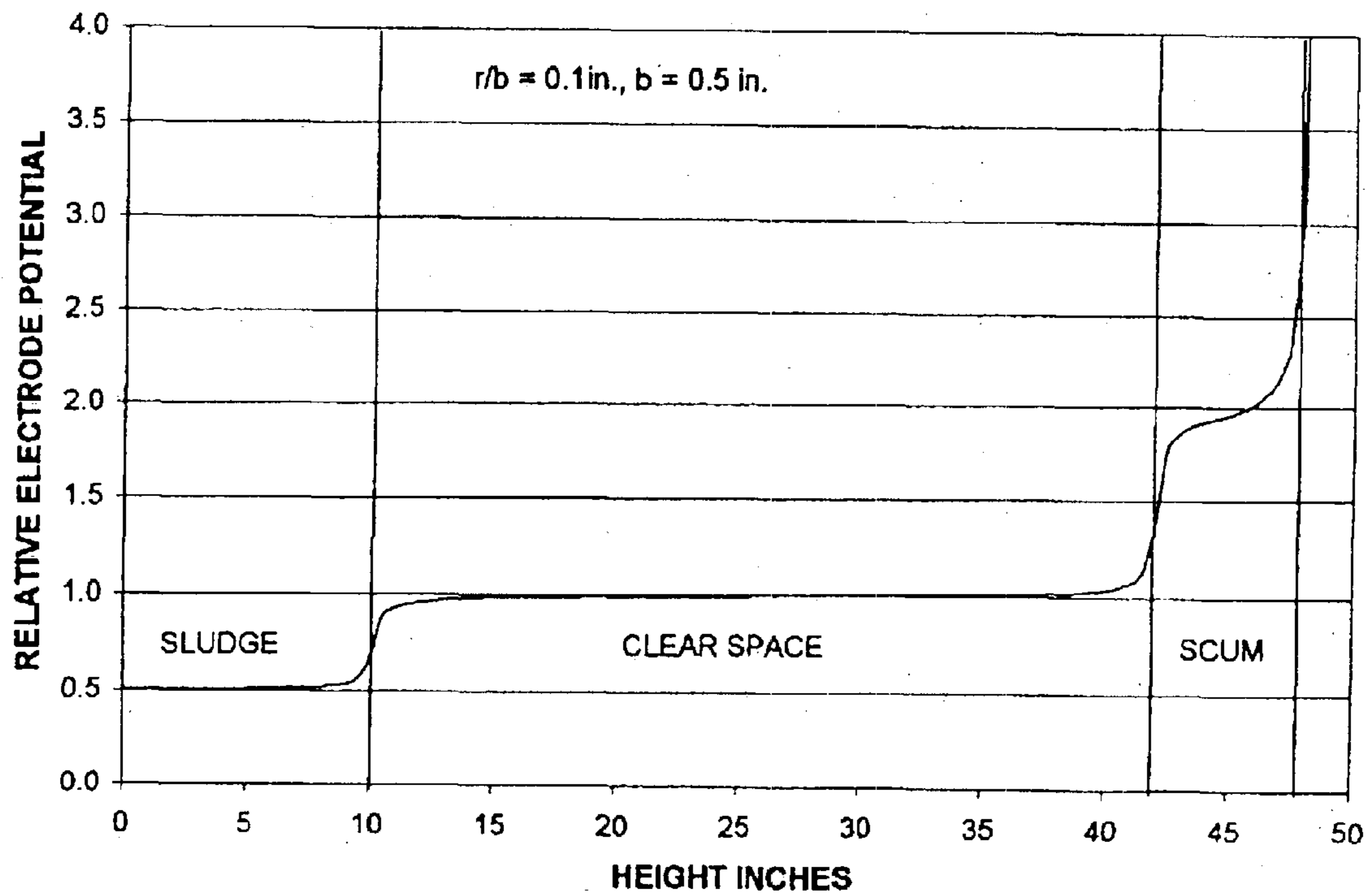
FIG. 8B RING ELECTRODE
