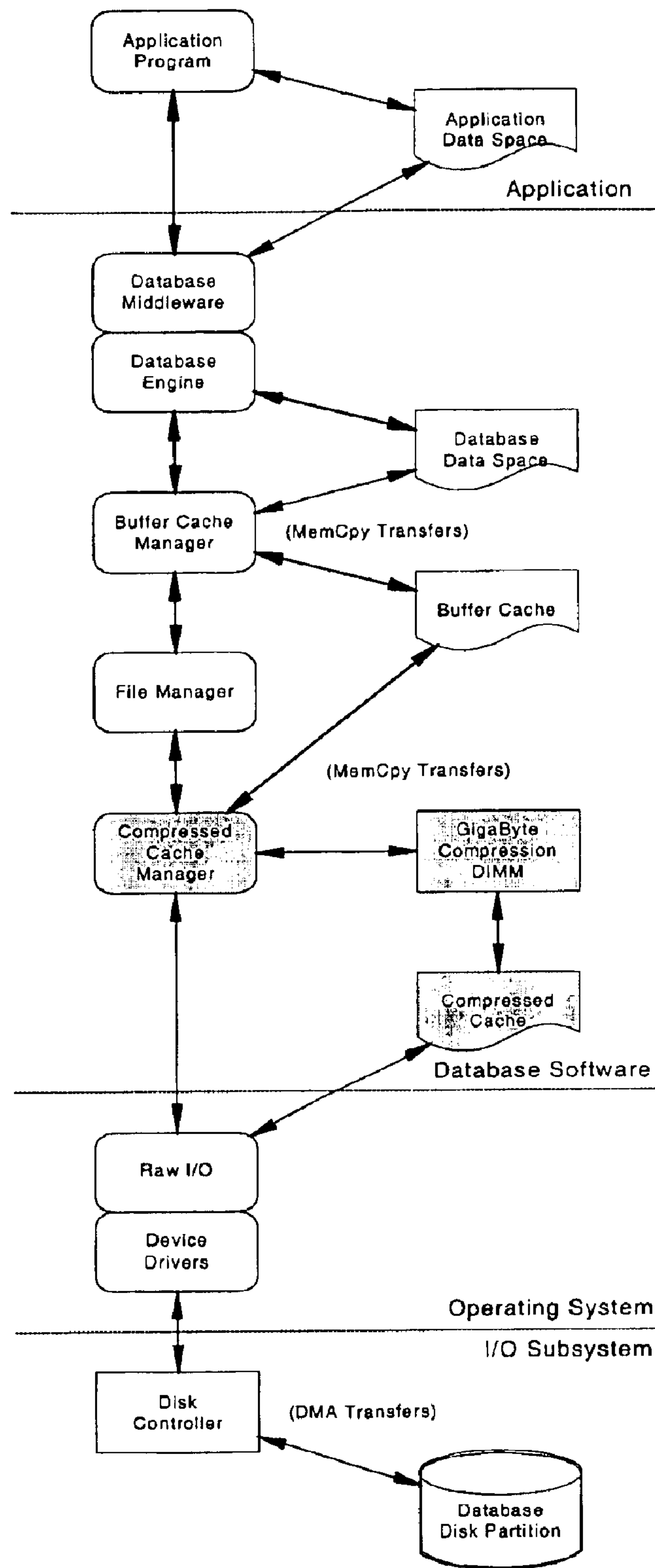
Fig 47 File System Filter Example
