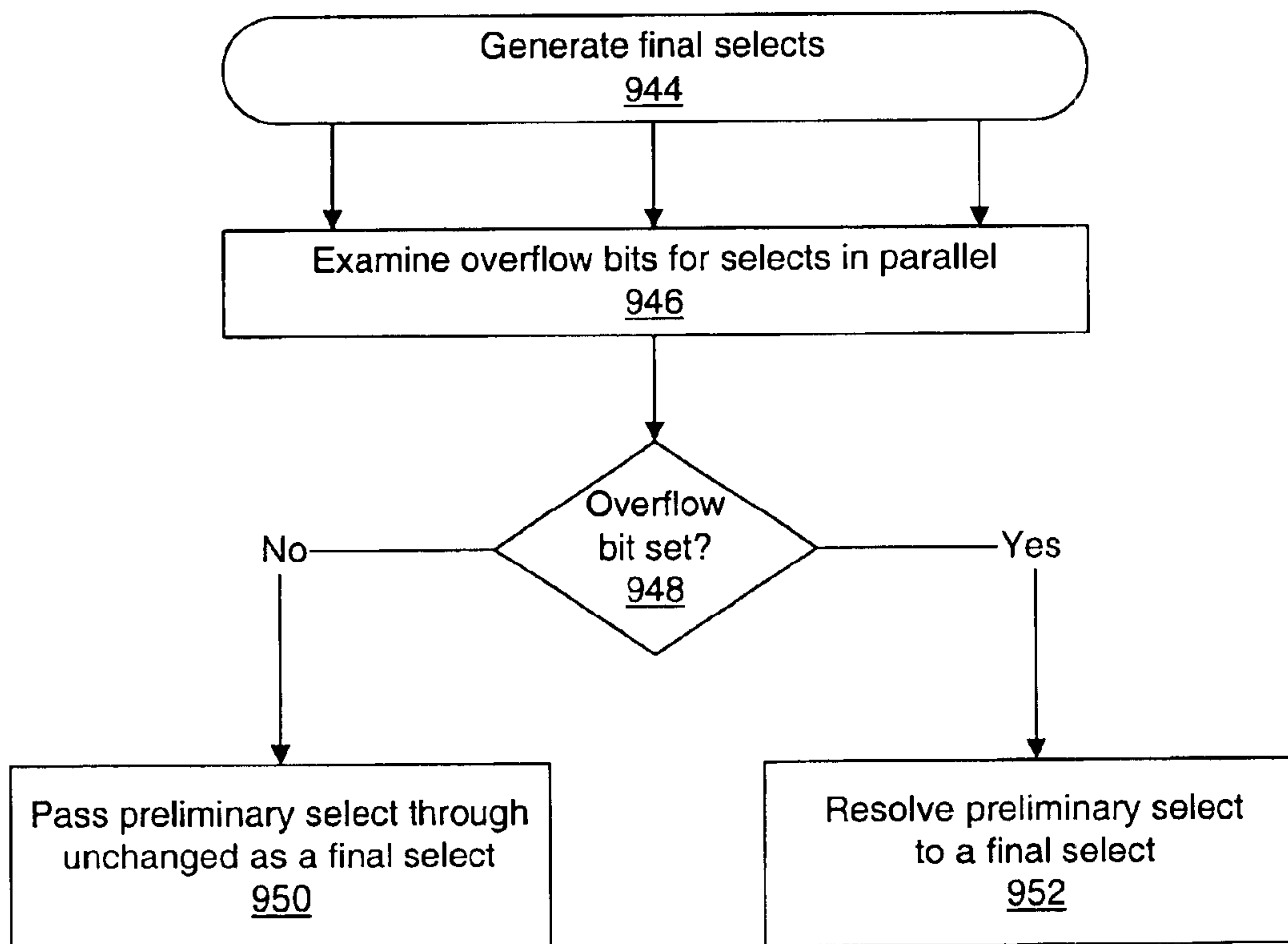
Figure 43h Decompression flowchart
