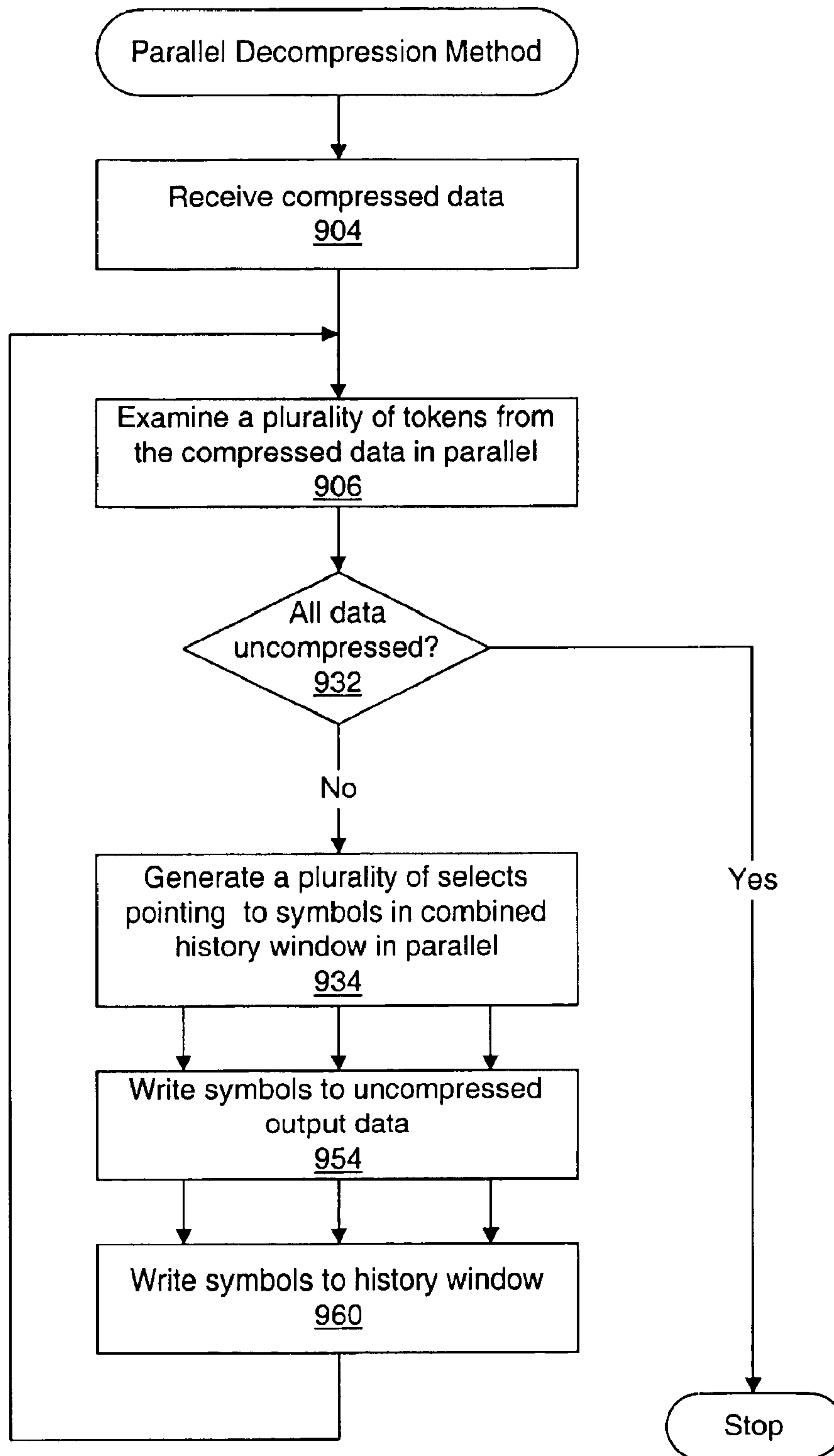
Figure 43b Decompression flowchart
