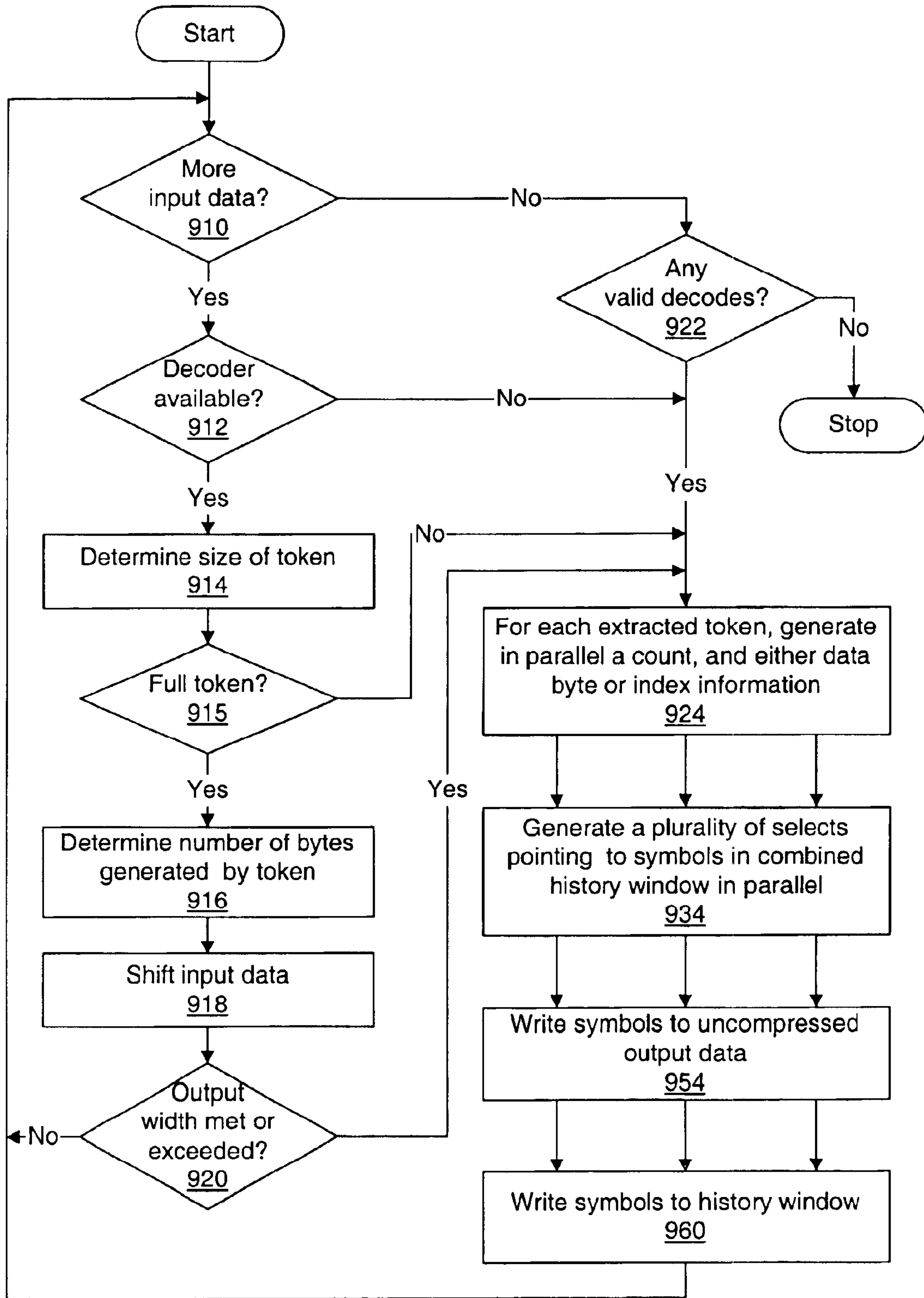
Figure 43k Decompression flowchart
