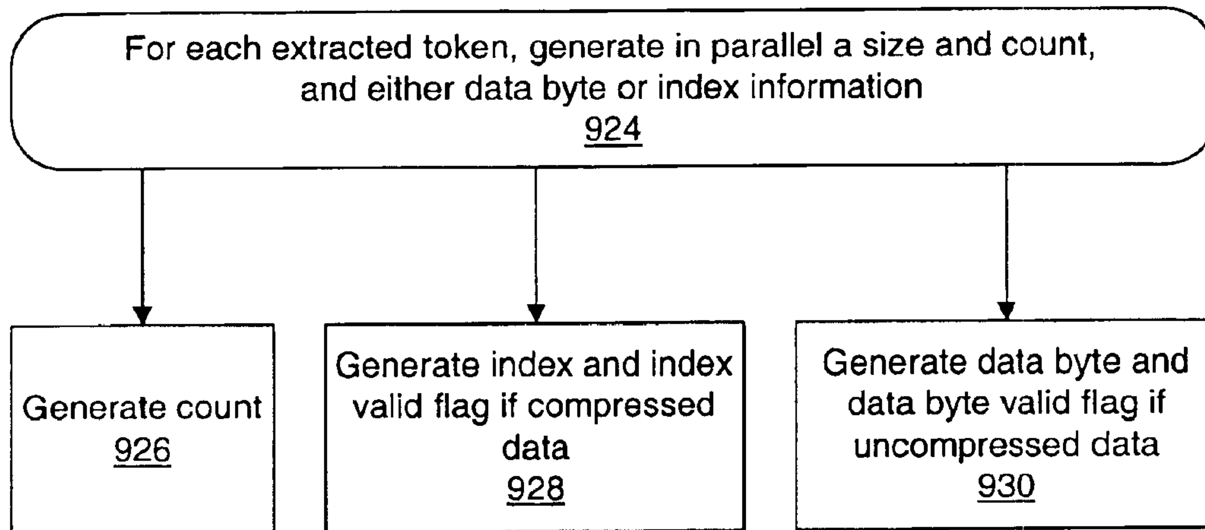
Figure 43e Decompression flowchart
