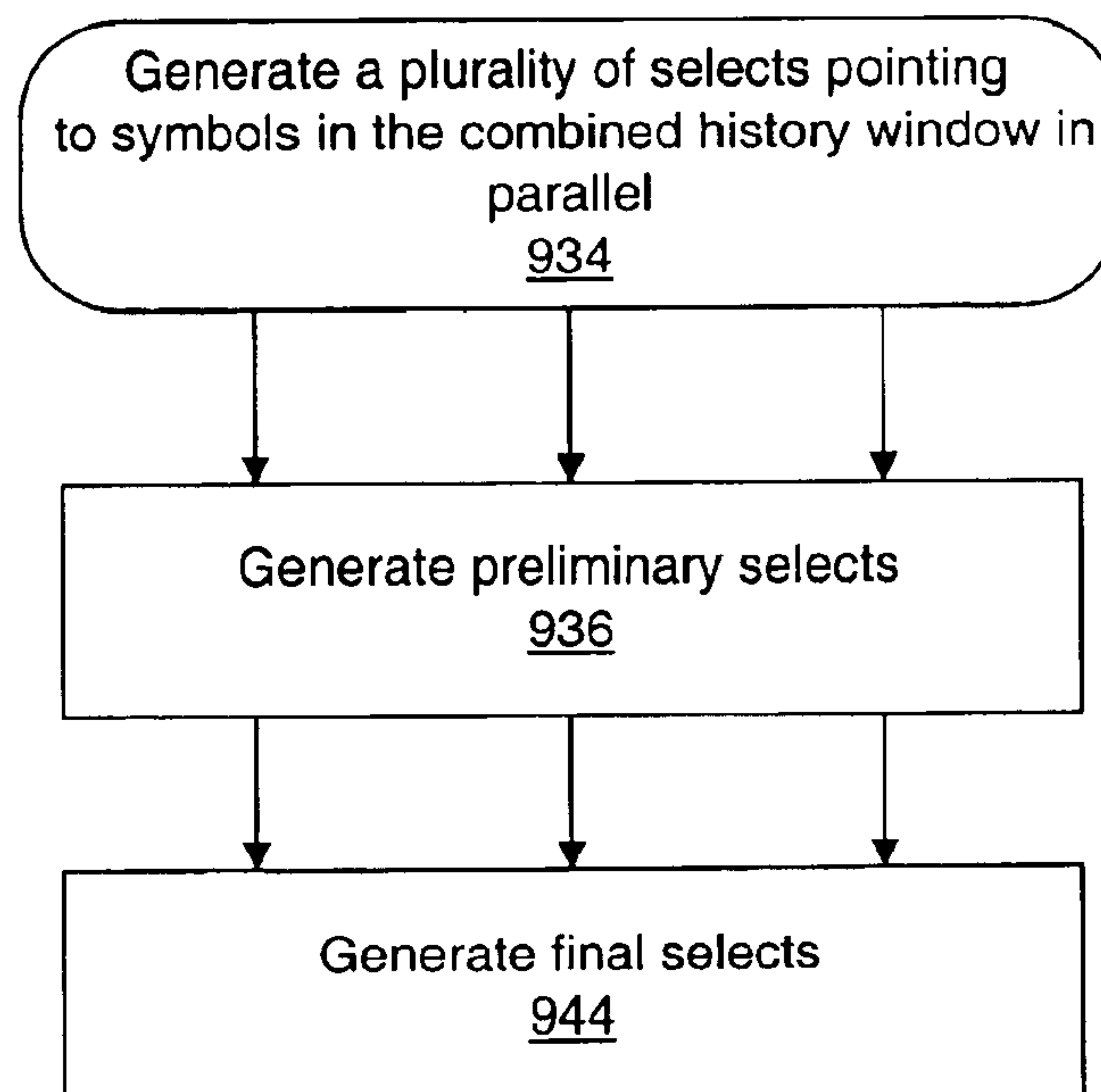
Figure 43f Decompression flowchart
