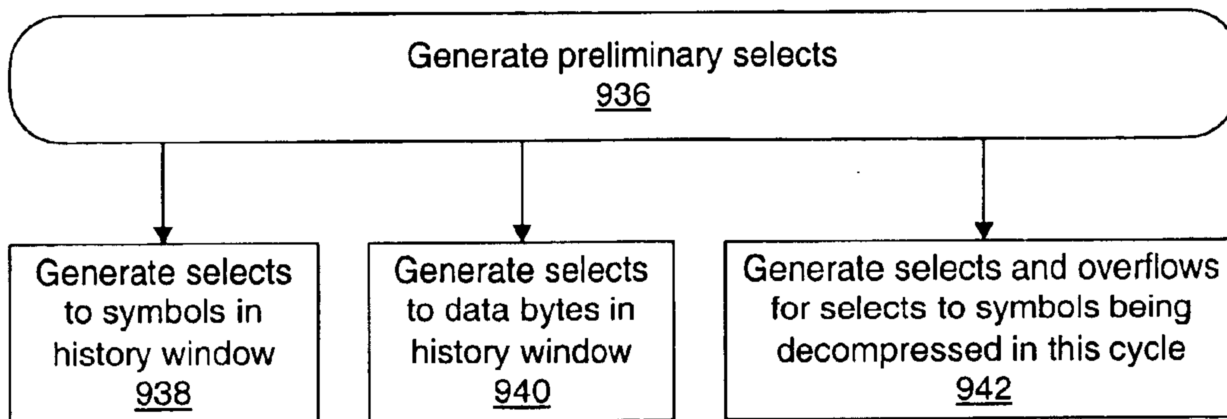
Figure 43g Decompression flowchart
