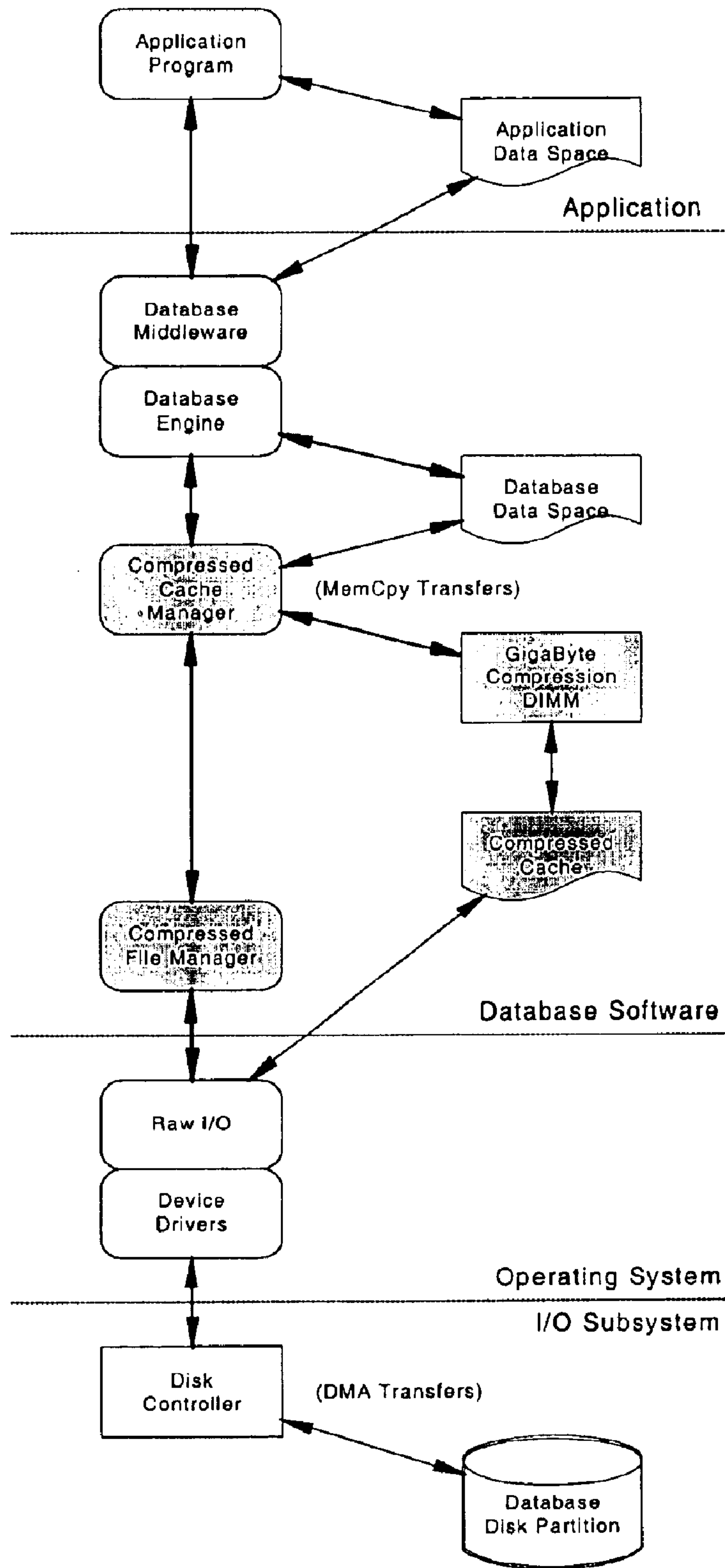
Fig. 48 Compressed Buffer Cache Example
