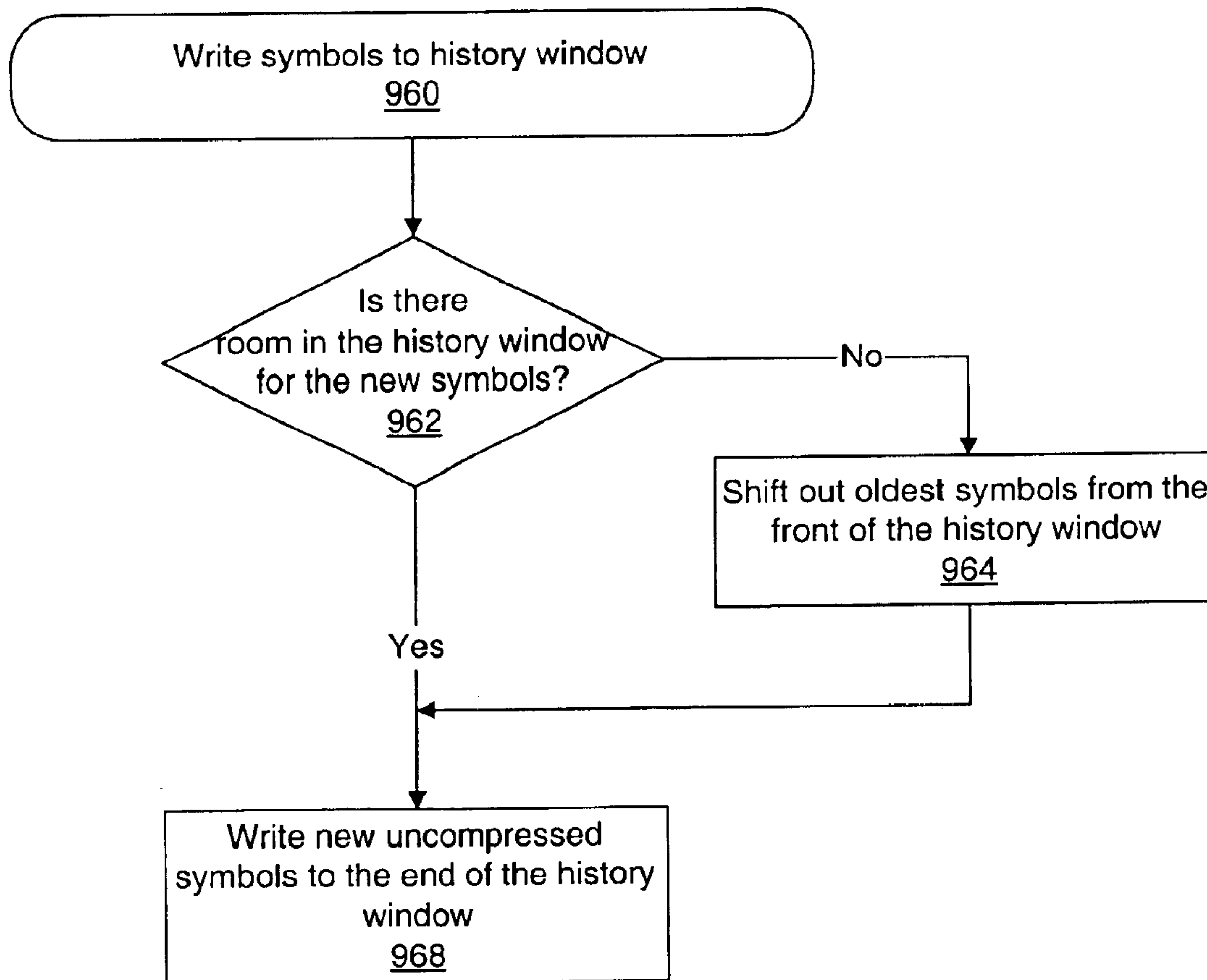
Figure 43j Decompression flowchart
