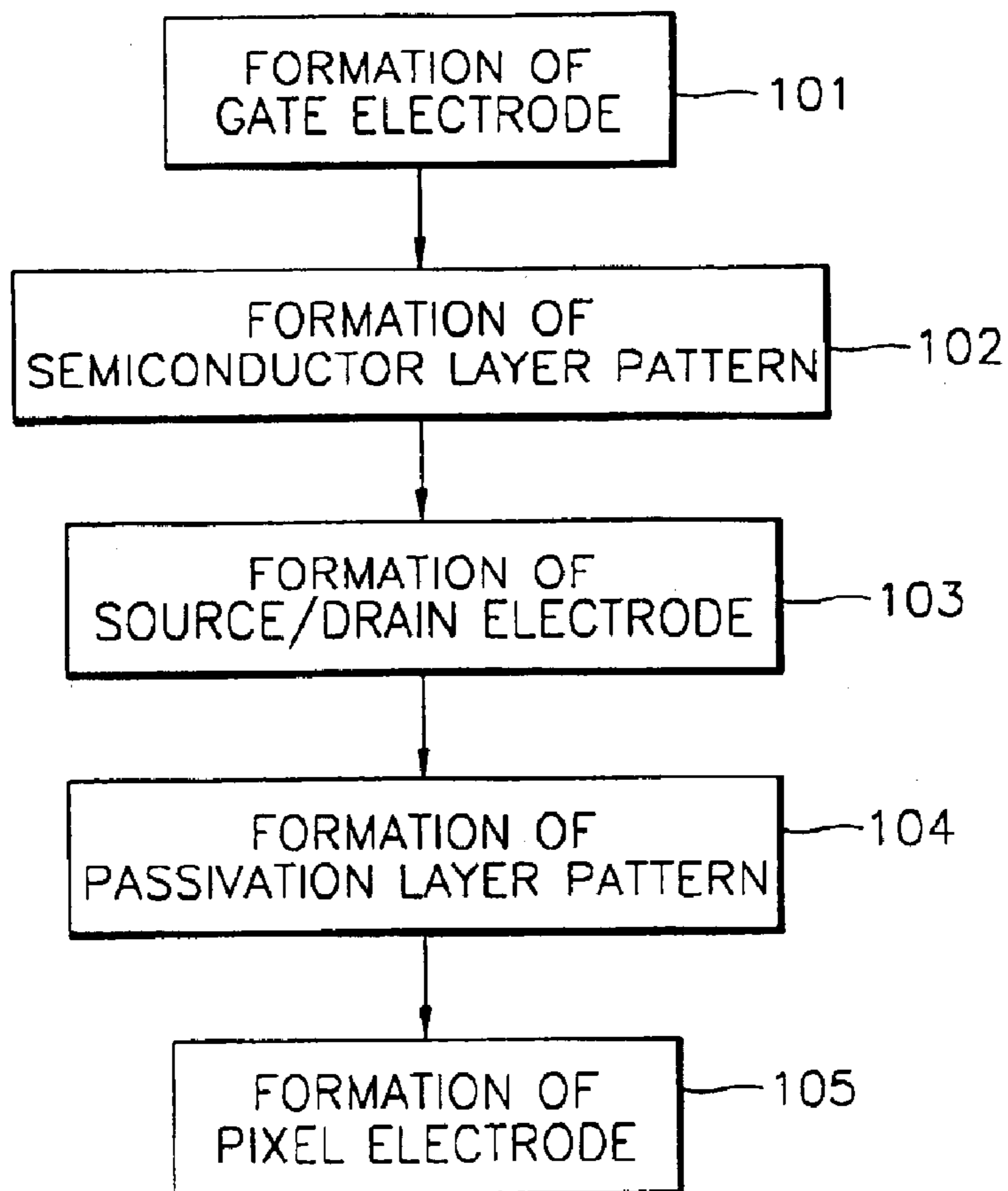
FIG. 2 (PRIOR ART)
