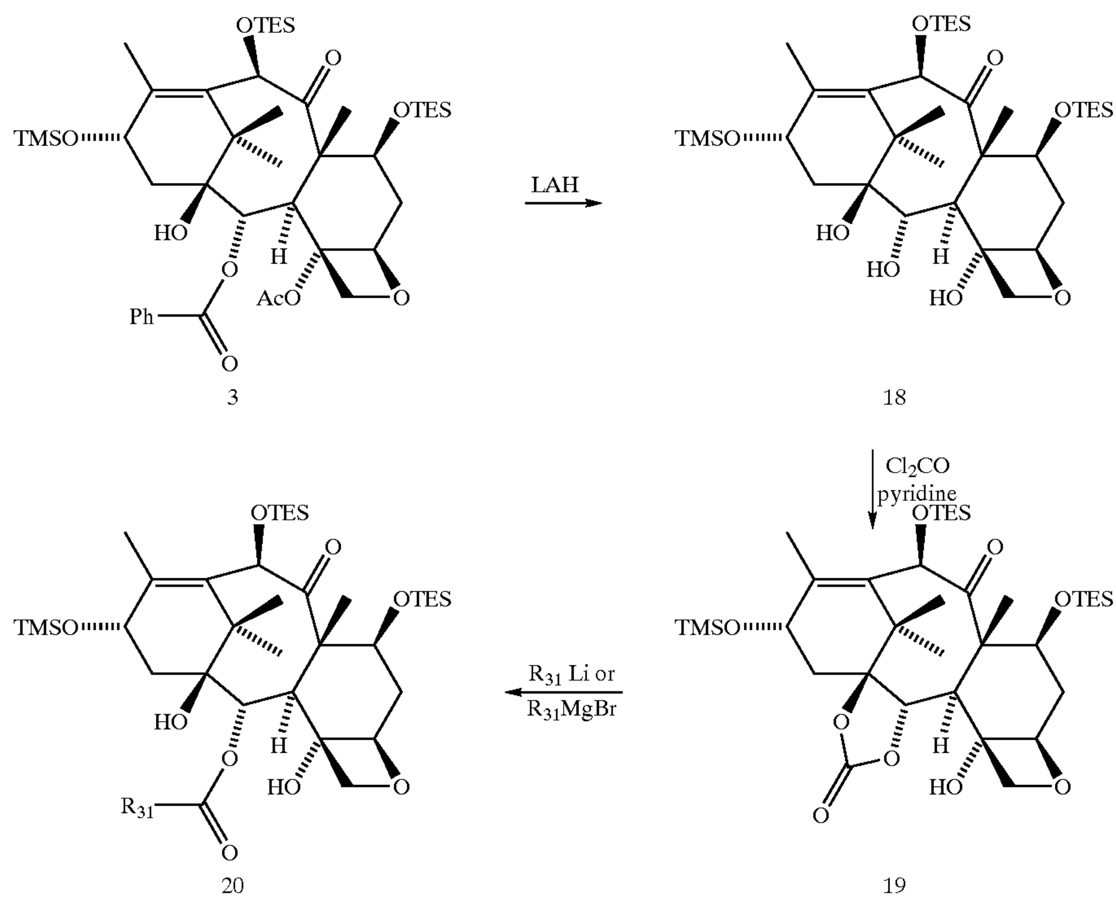
Scheme 6
