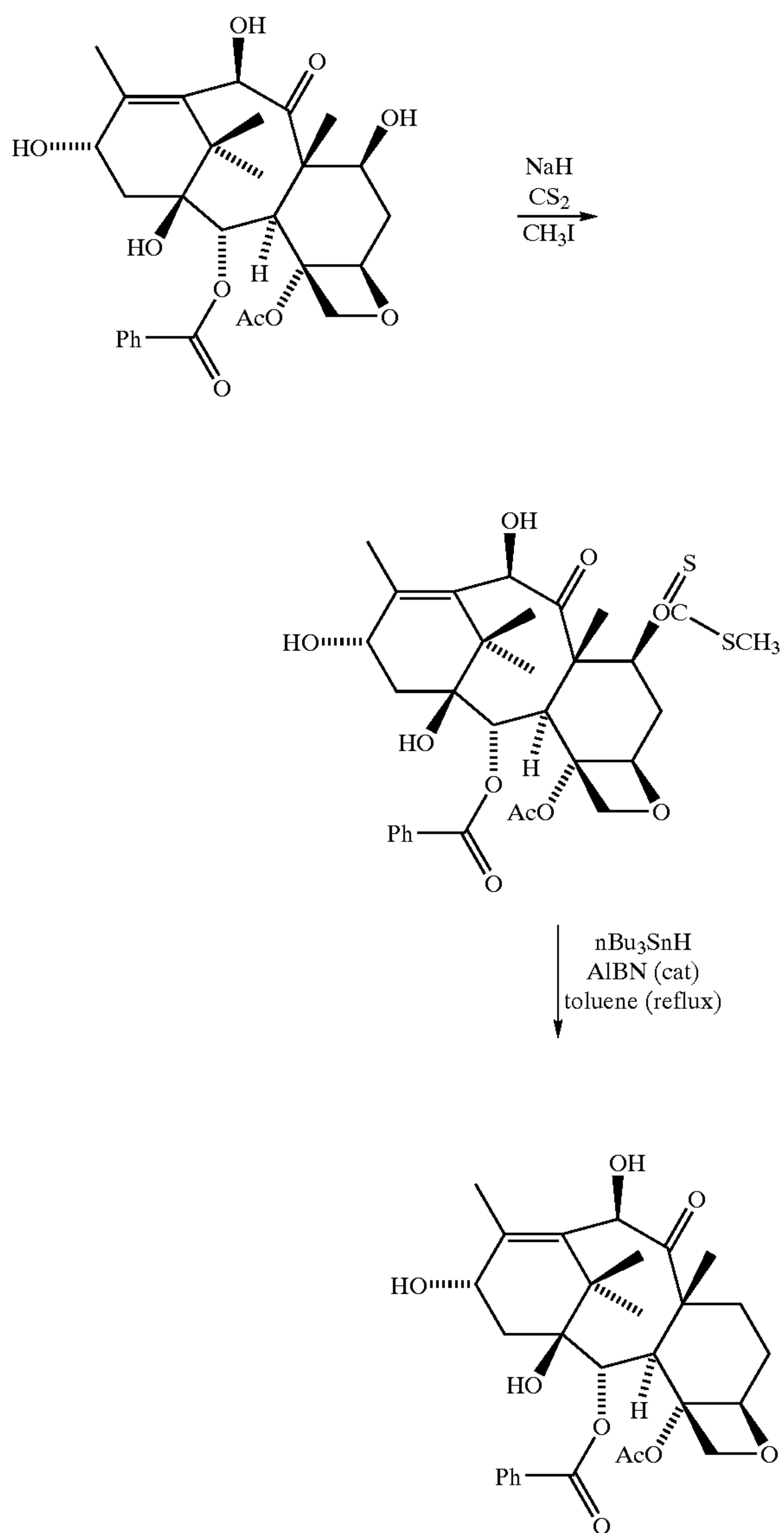
REACTION SCHEME 11
