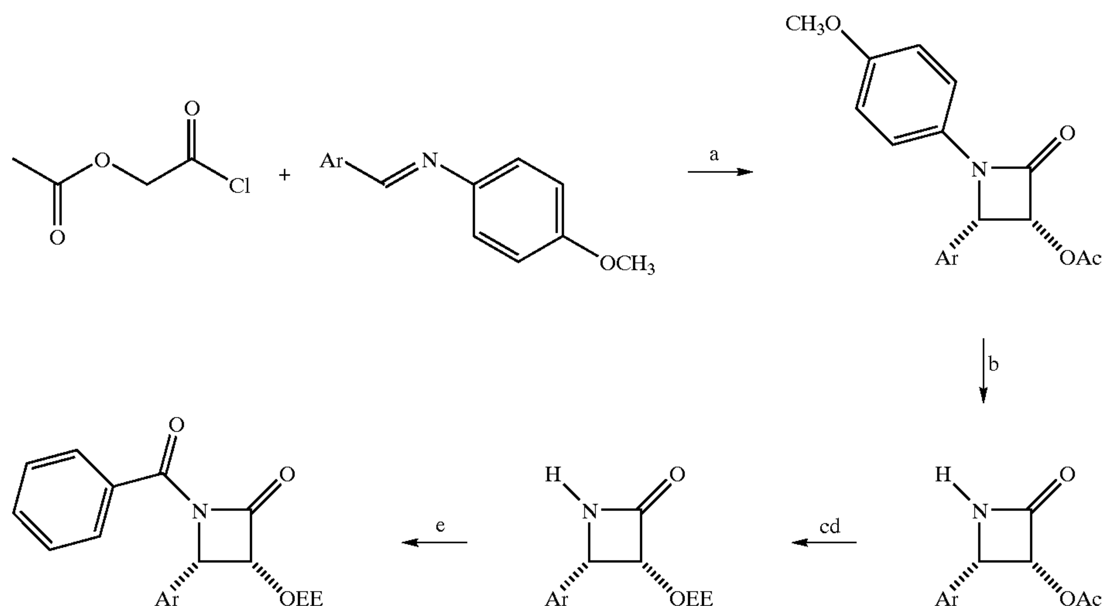
Scheme A
