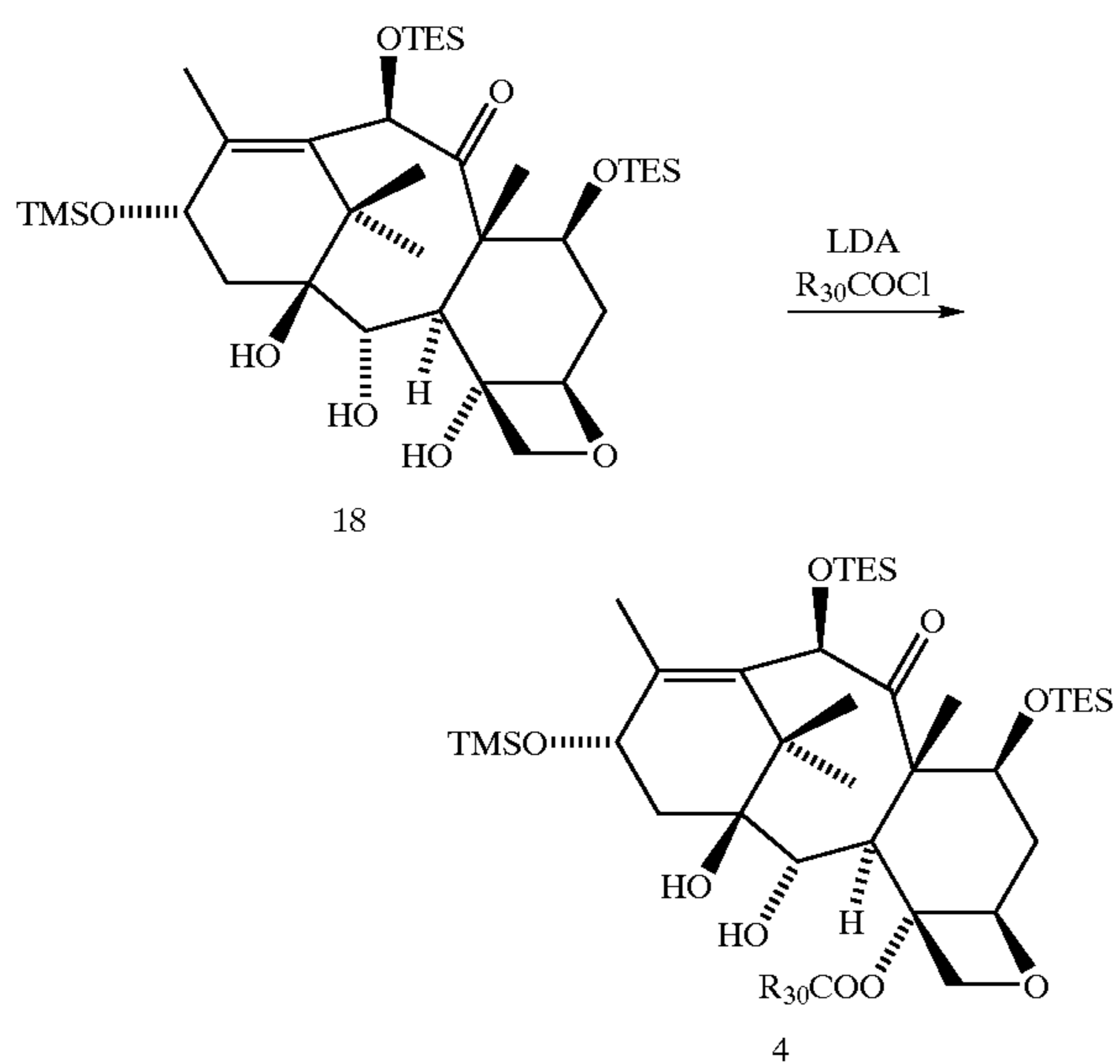
Scheme 7
