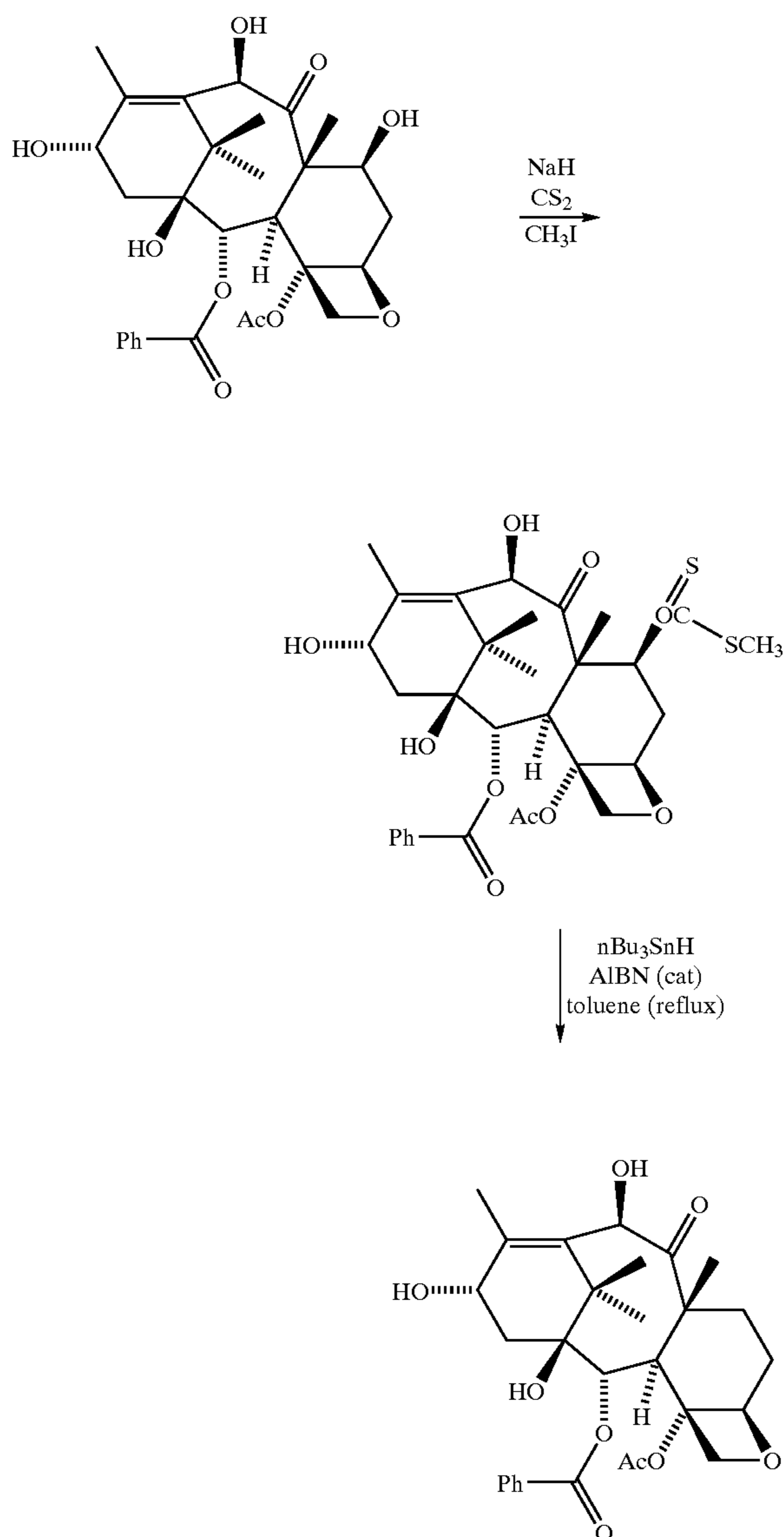
REACTION SCHEME 11
