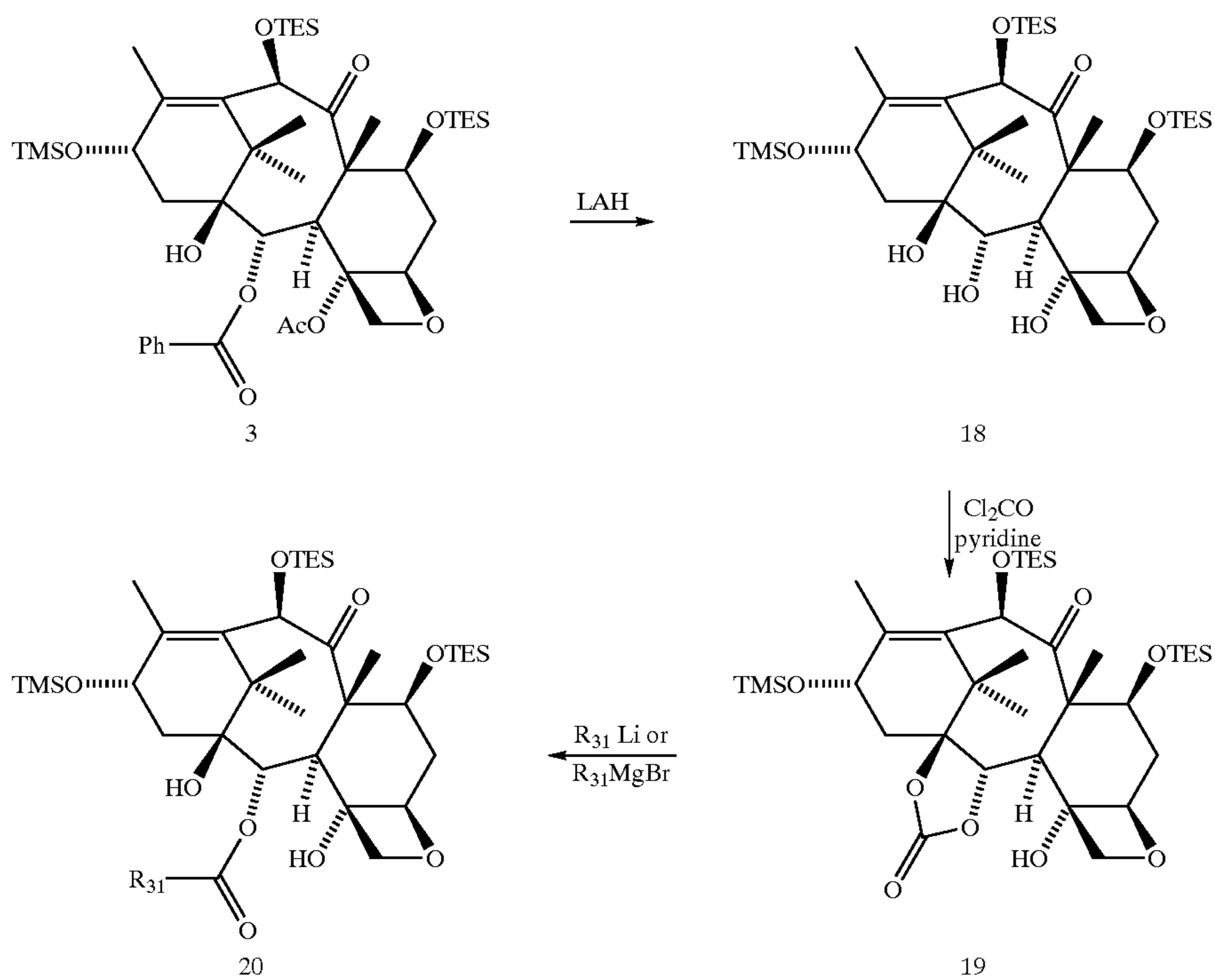
Scheme 6
