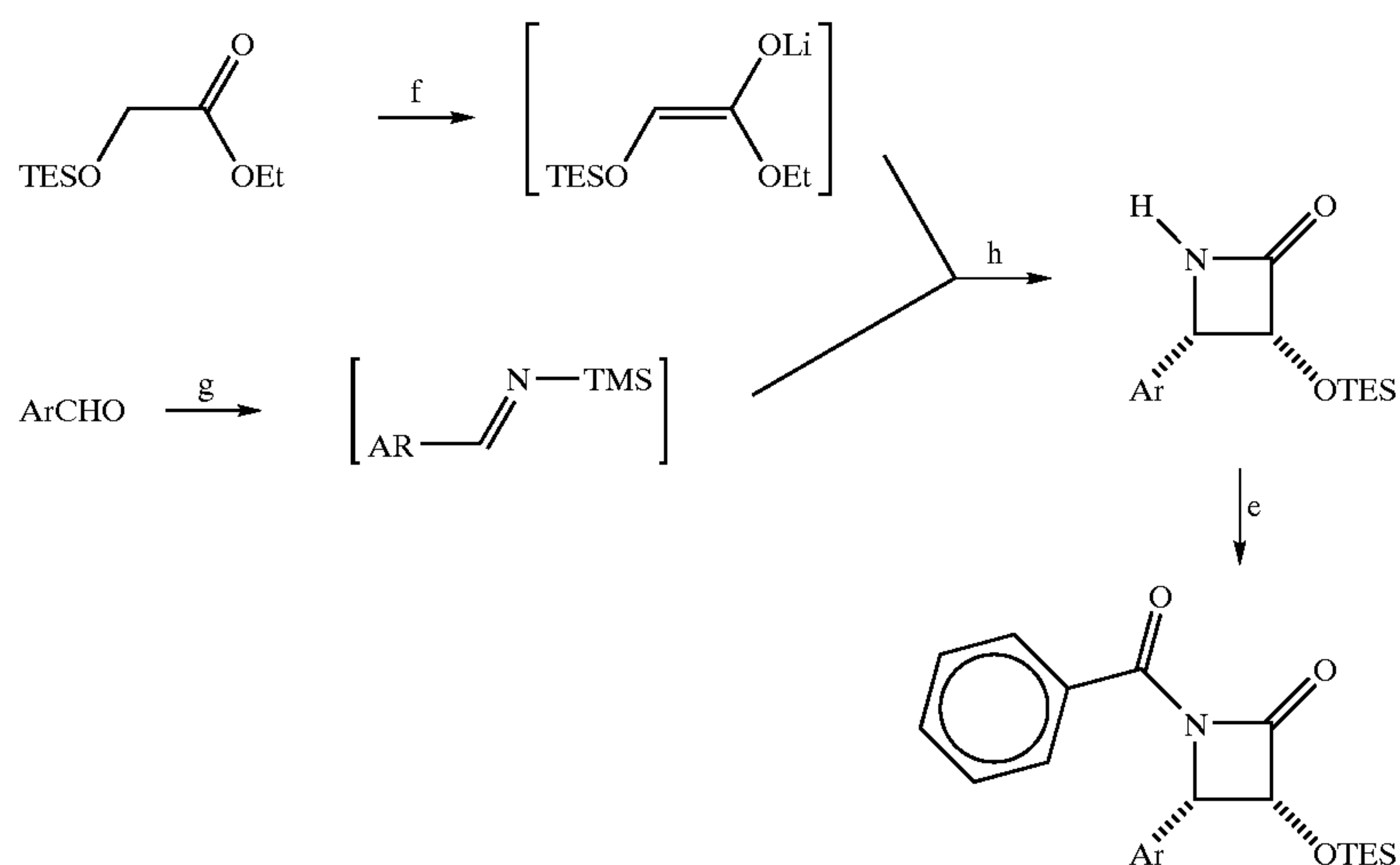
Scheme B
