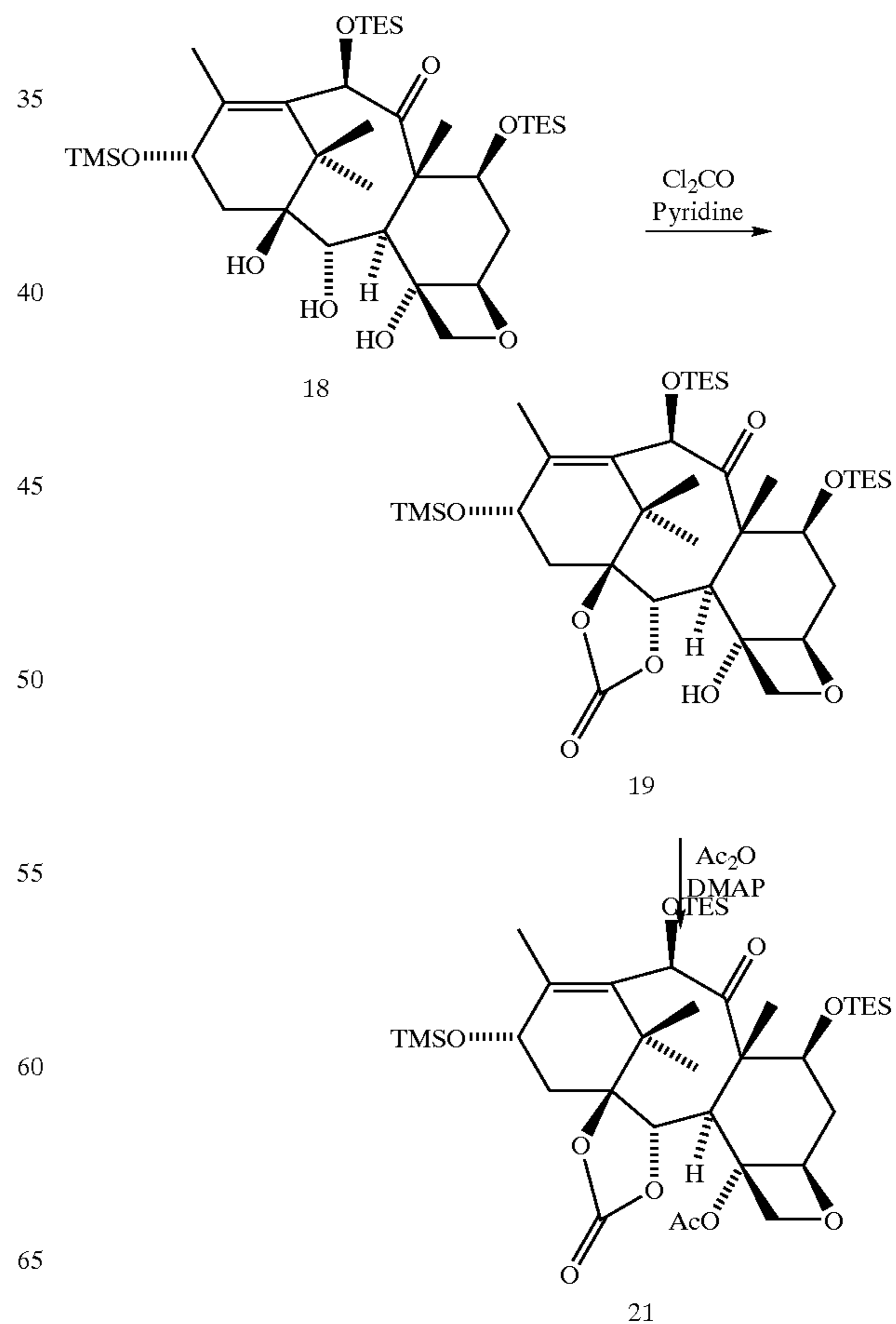
Scheme 8
