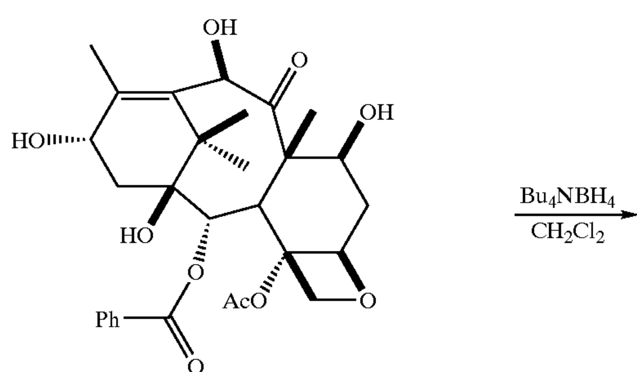
REACTION SCHEME 4
