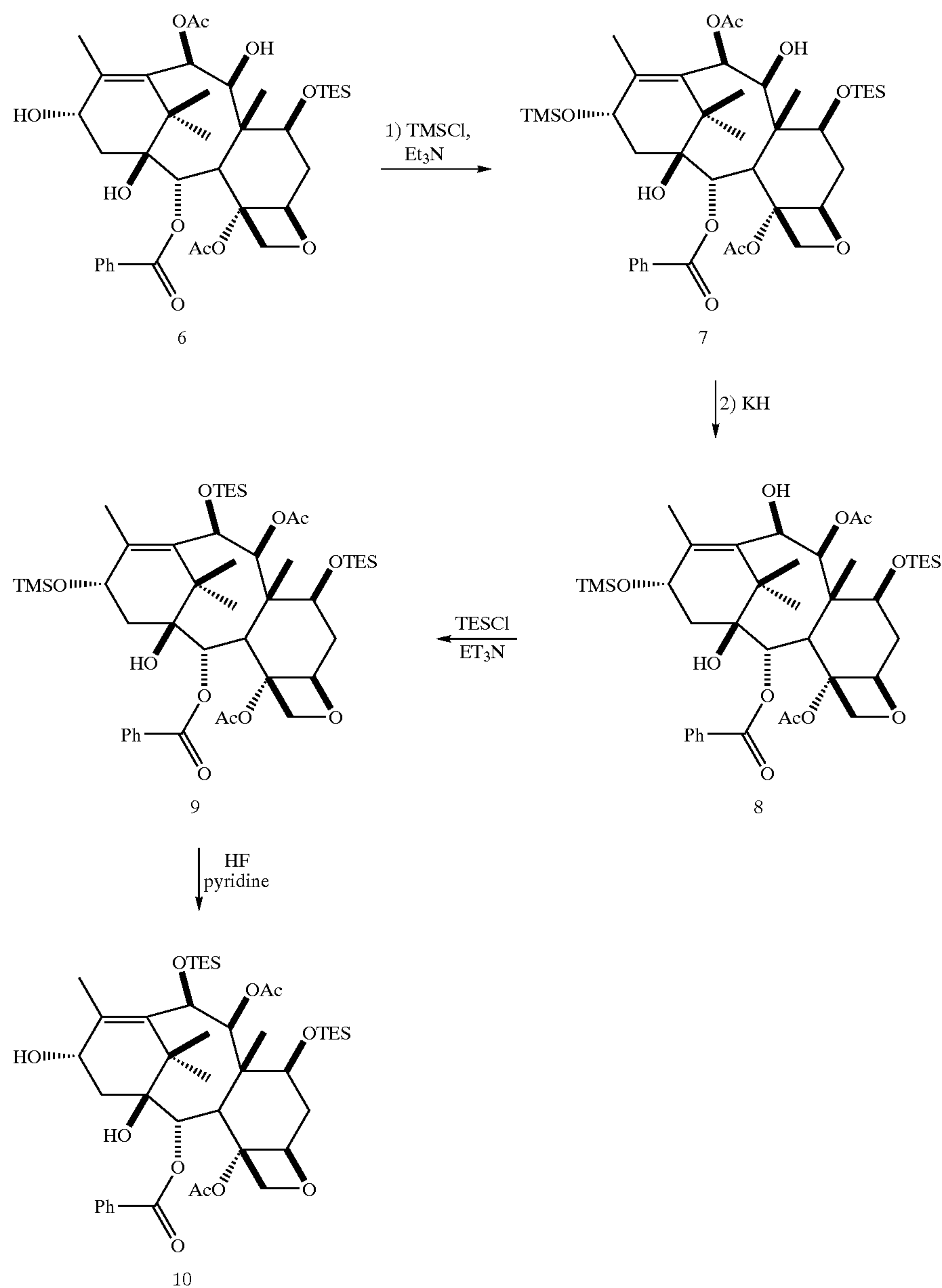
REACTION SCHEME 2
