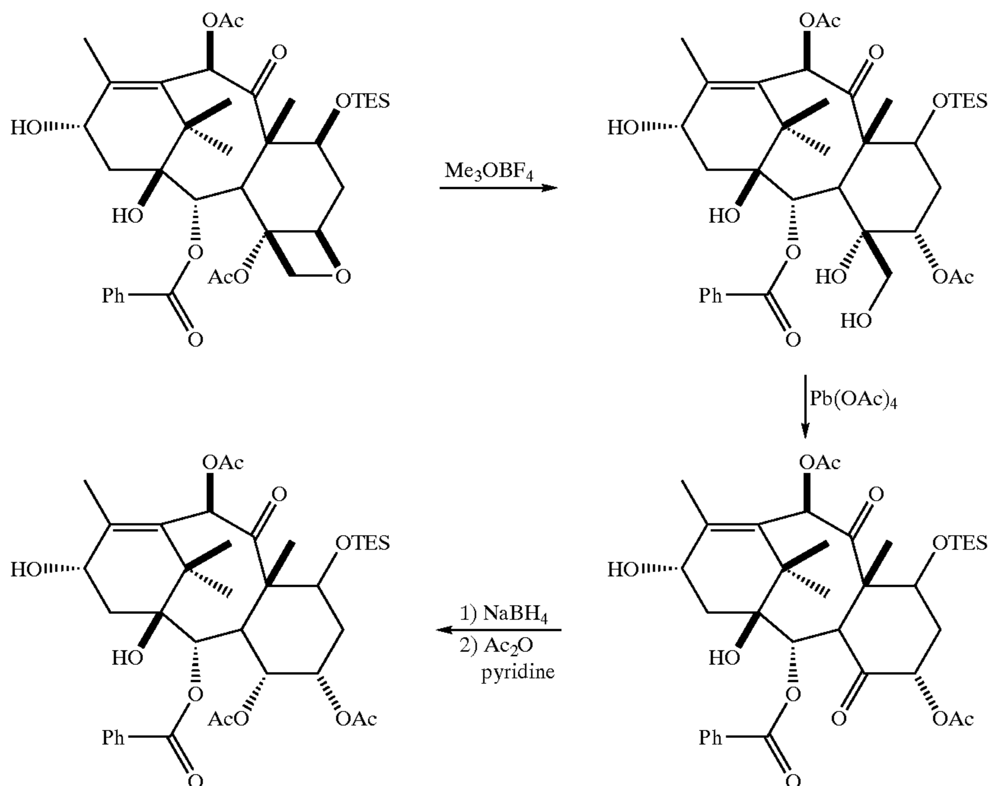
REACTION SCHEME 13
