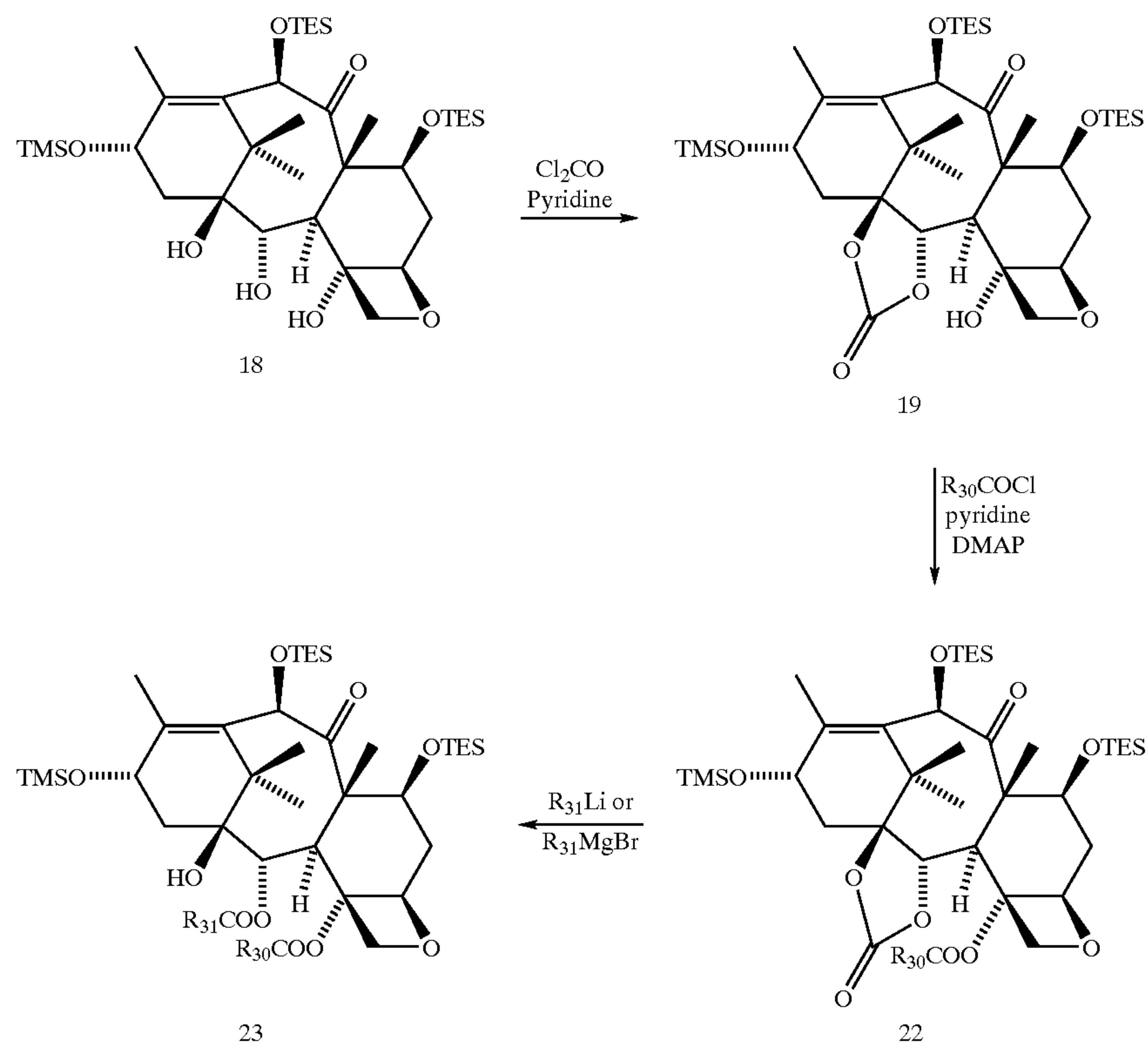
Scheme 9
