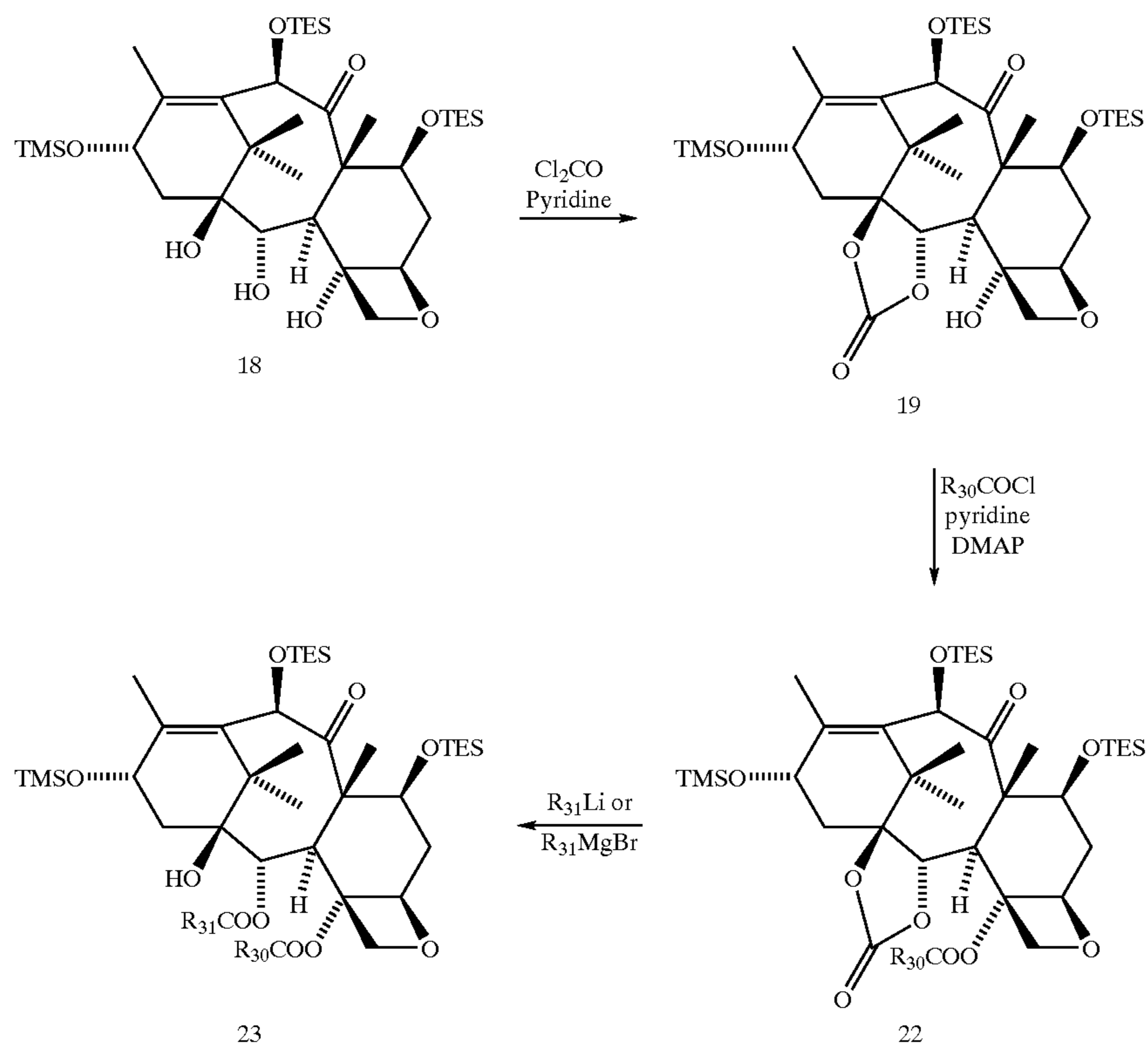
Scheme 9
