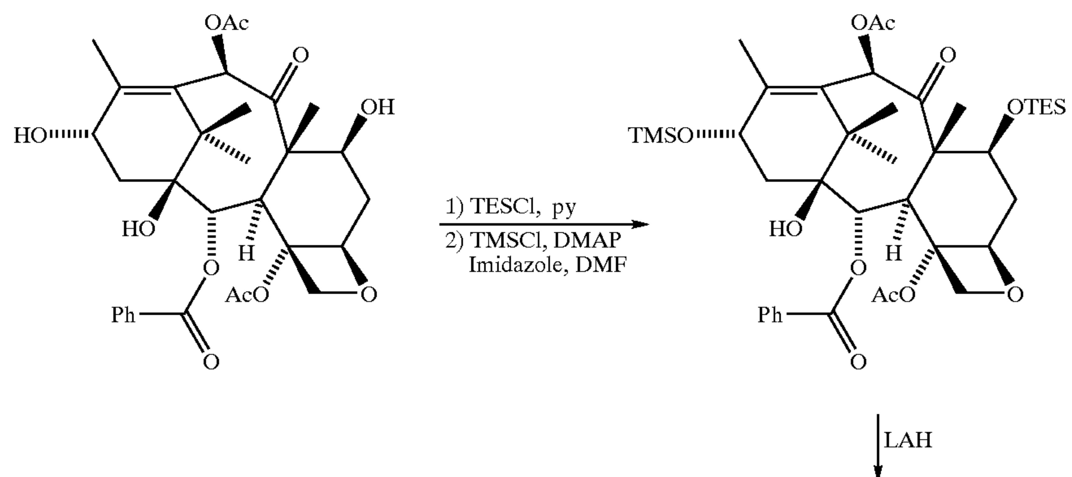
Scheme 10
