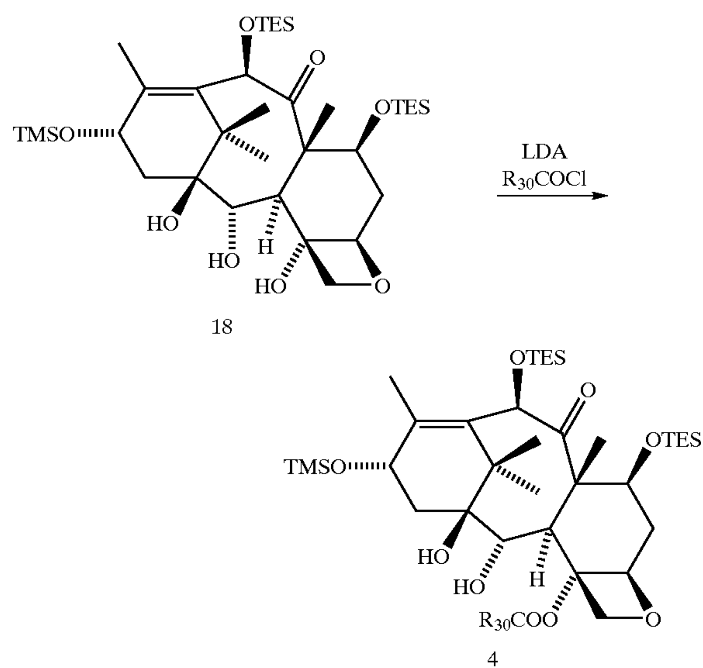
Scheme 7
