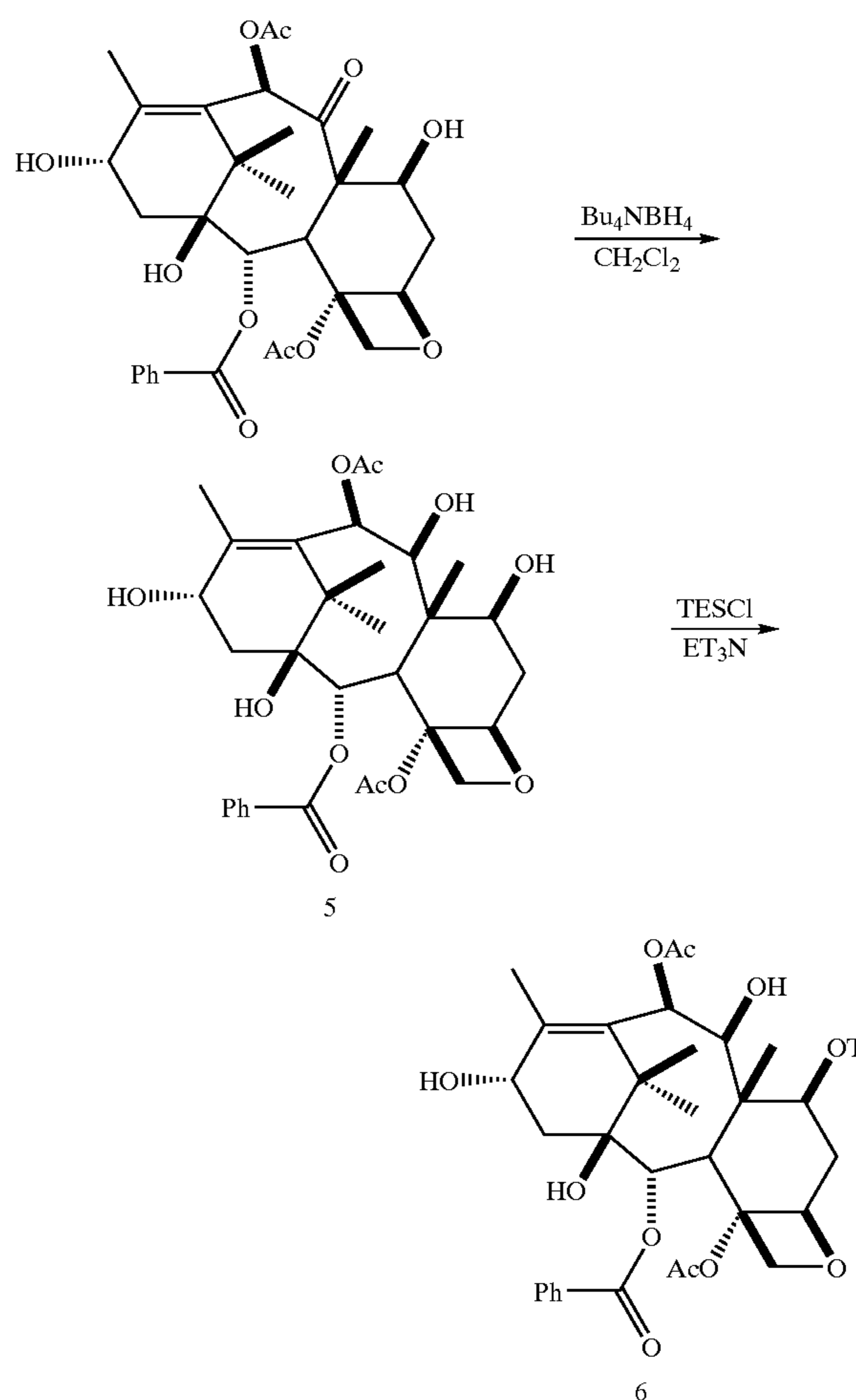
REACTION SCHEME 1
