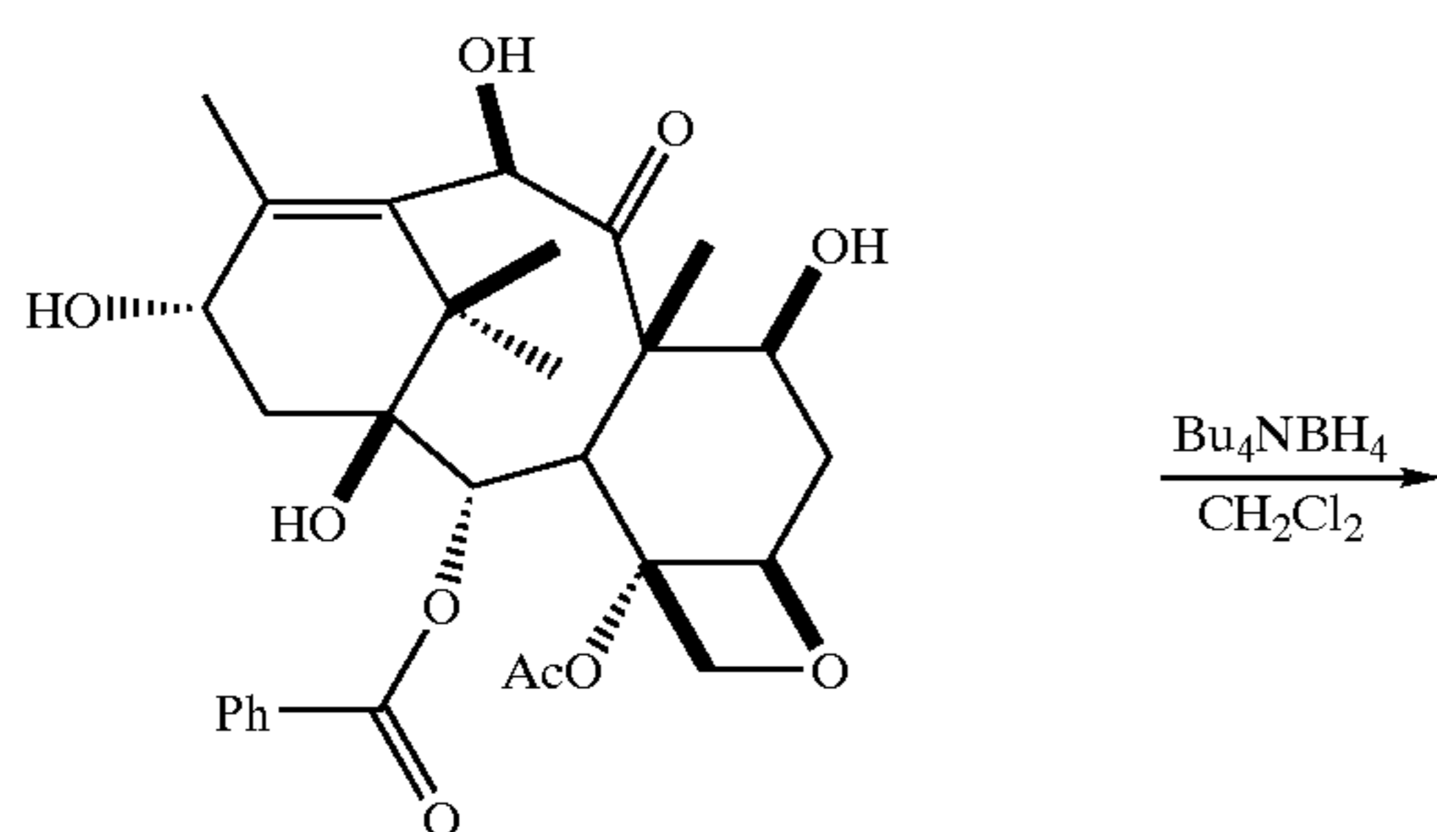
REACTION SCHEME 4
