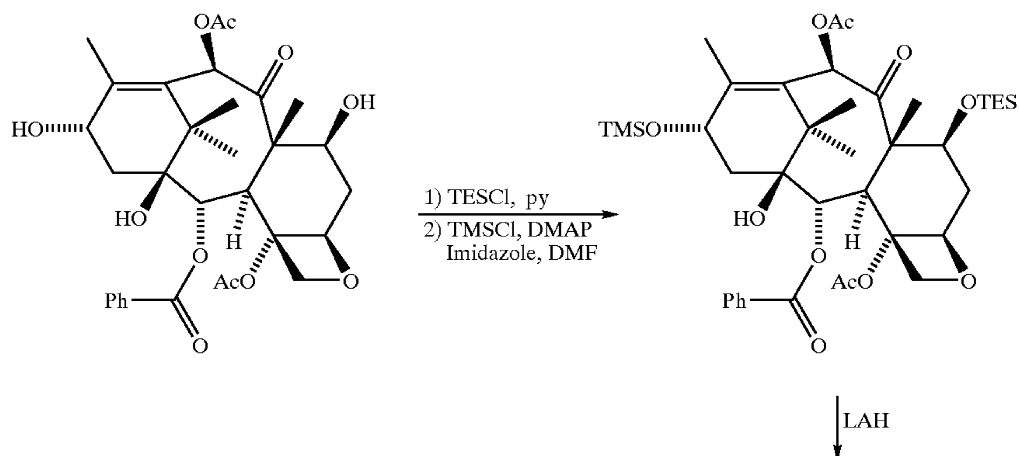
Scheme 10
