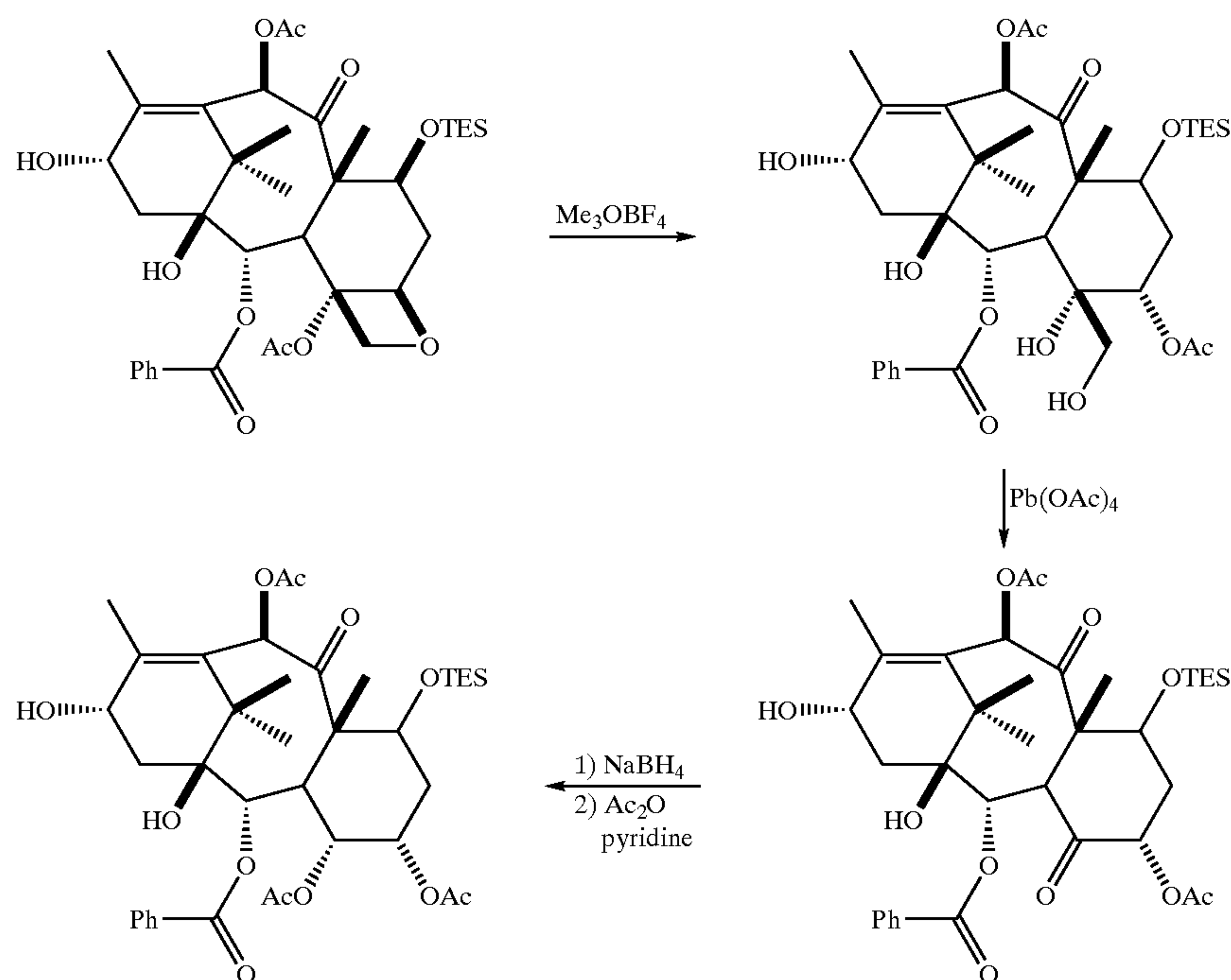
REACTION SCHEME 13
