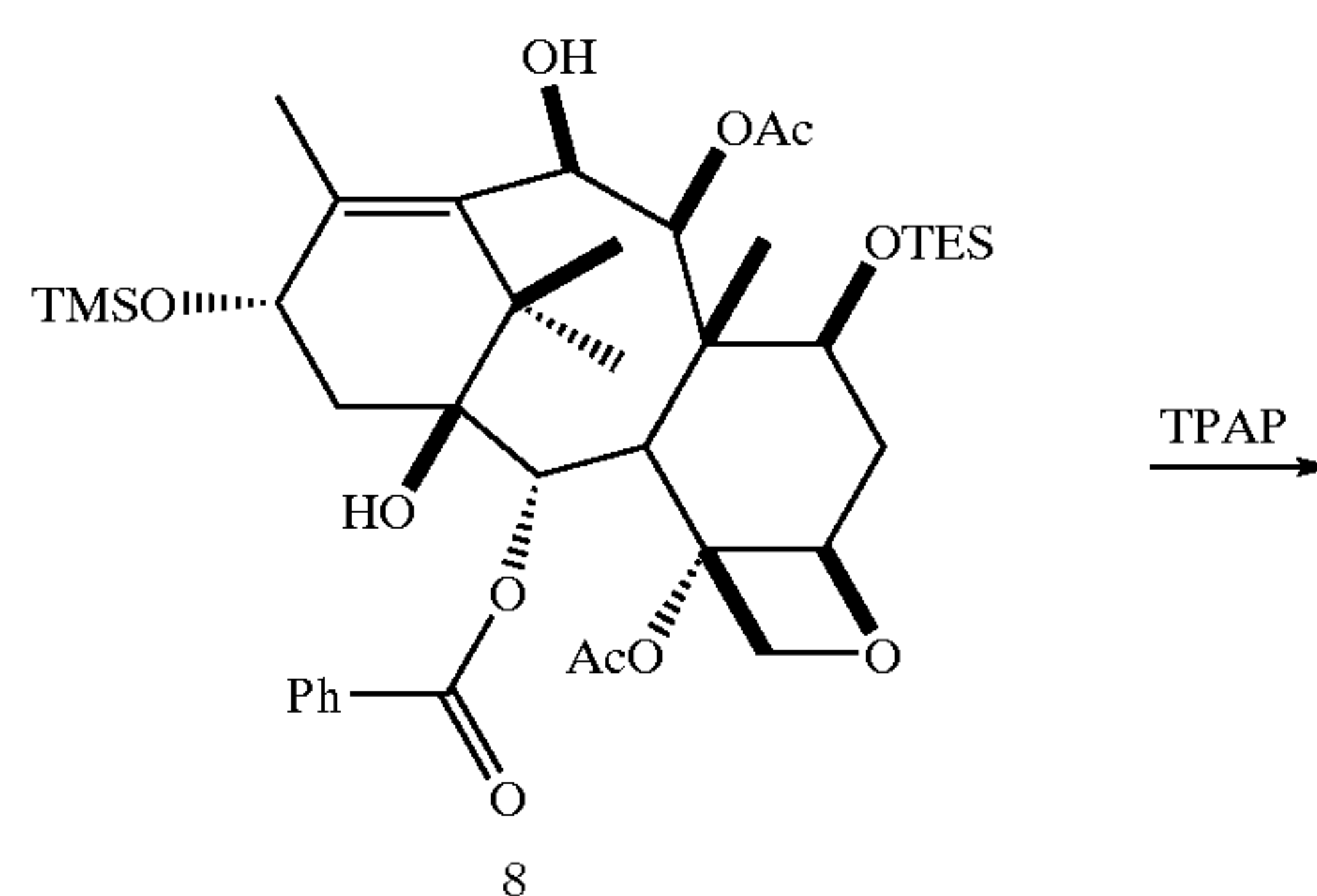
REACTION SCHEME 3
