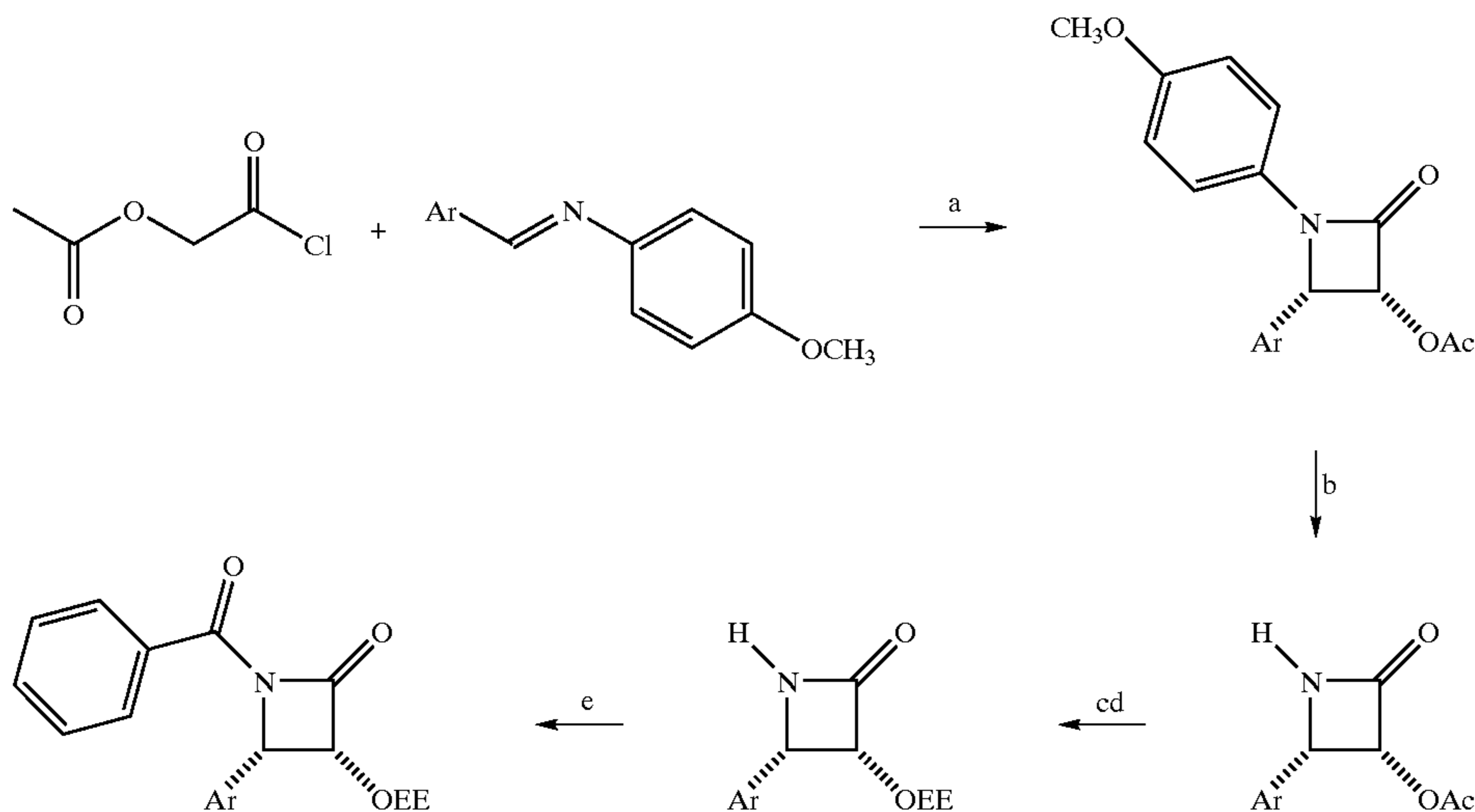
Scheme A
