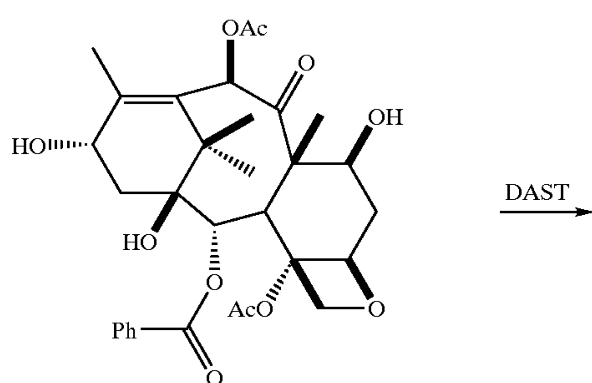
REACTION SCHEME 12
