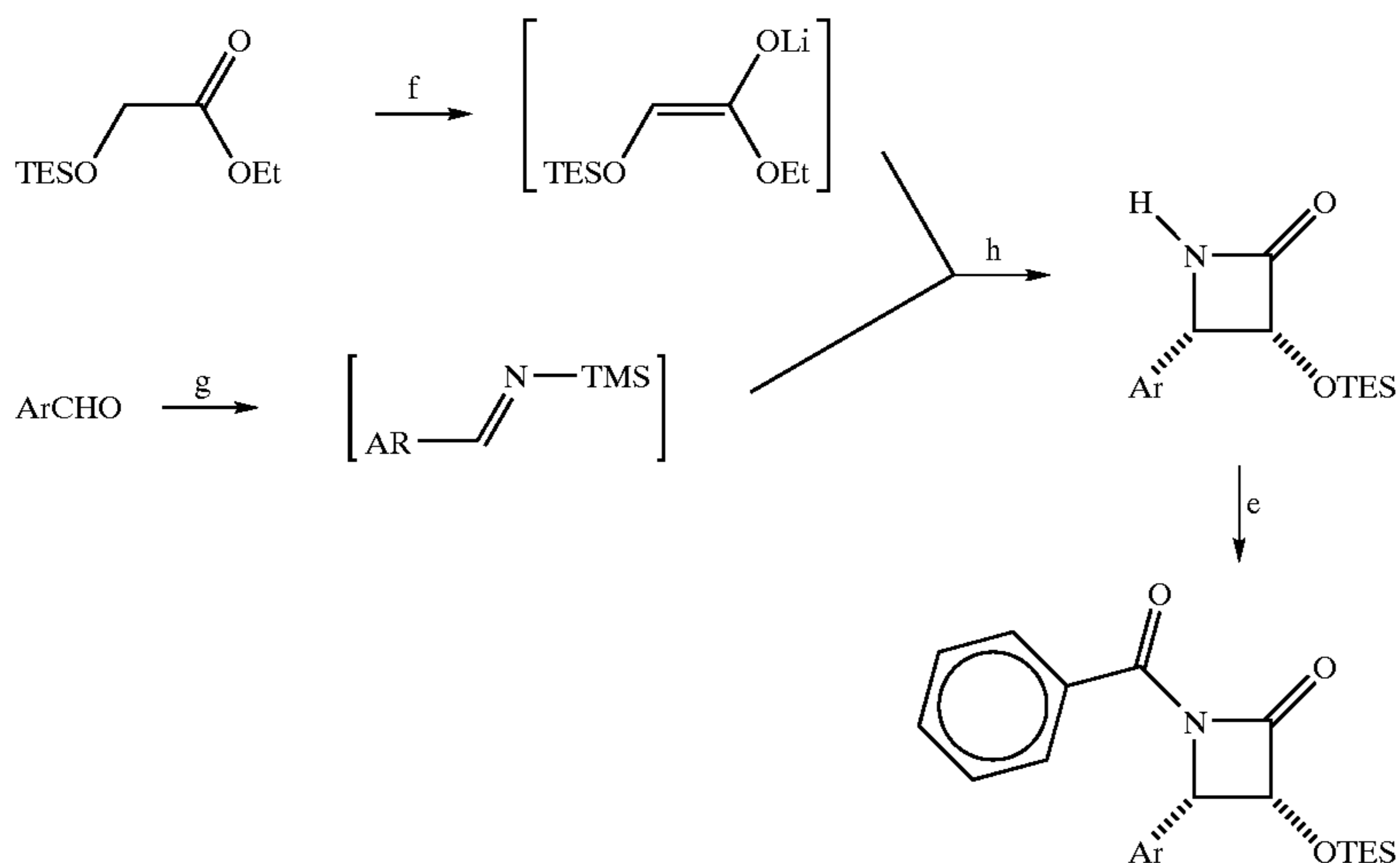
Scheme B
