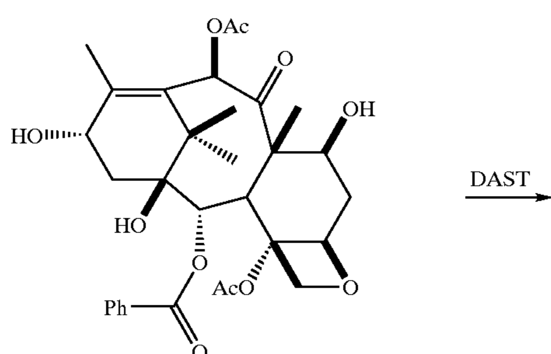
REACTION SCHEME 12
