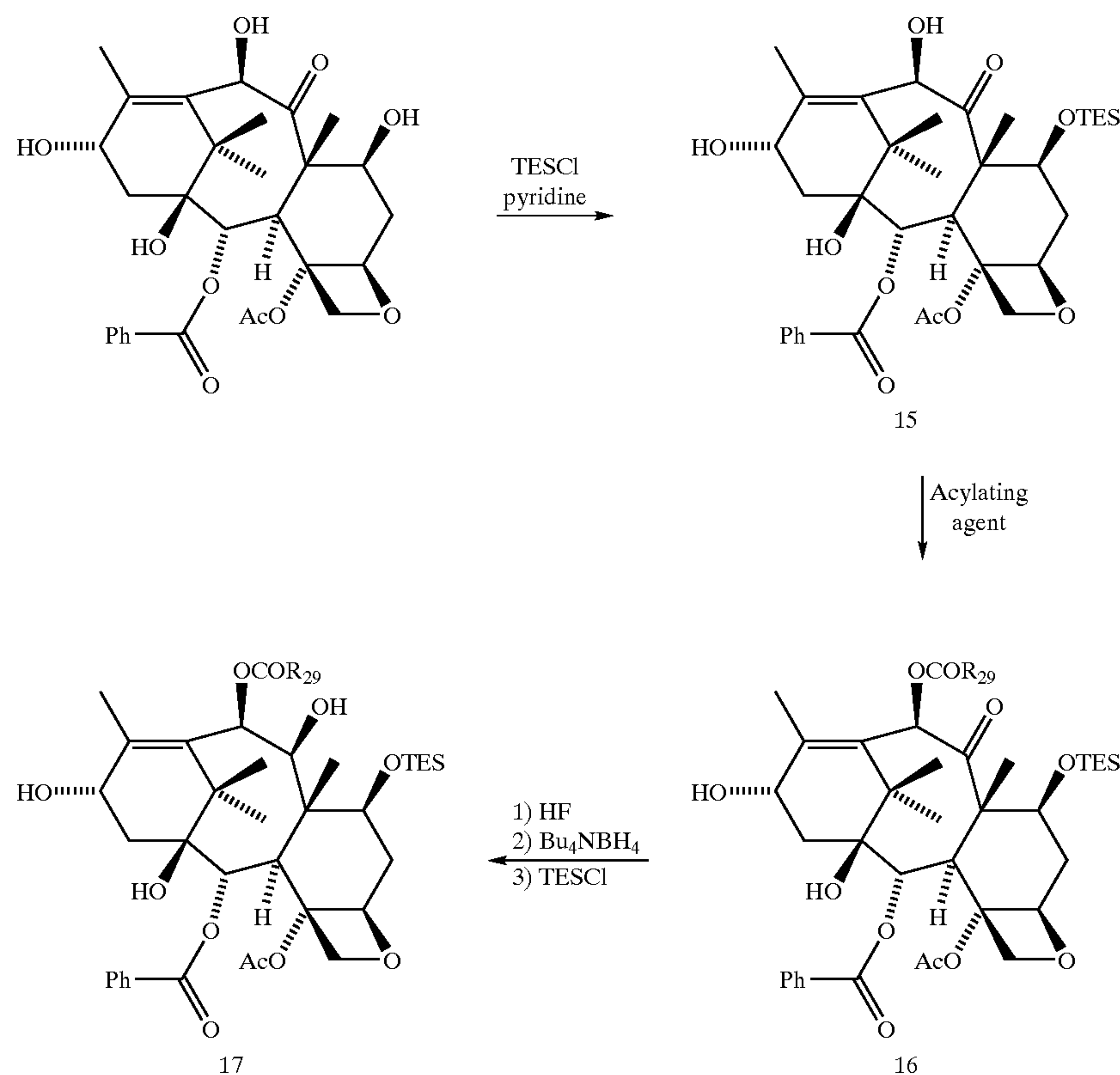
REACTION SCHEME 5
