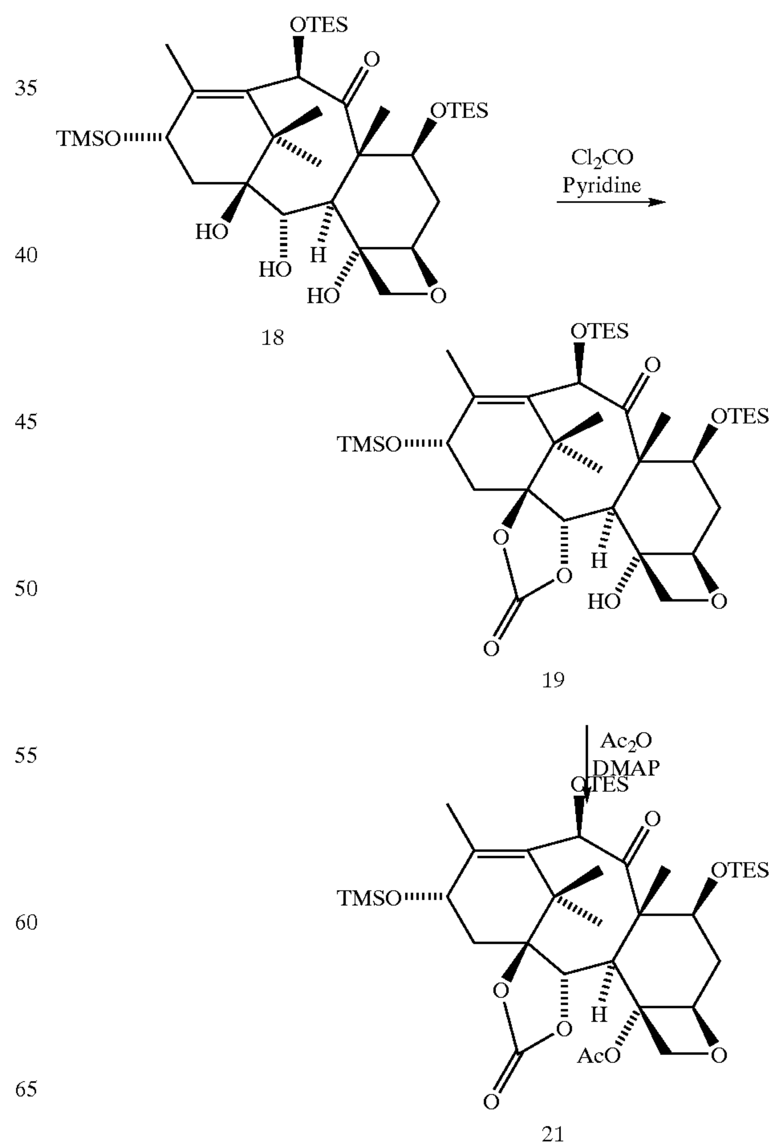
Scheme 8
