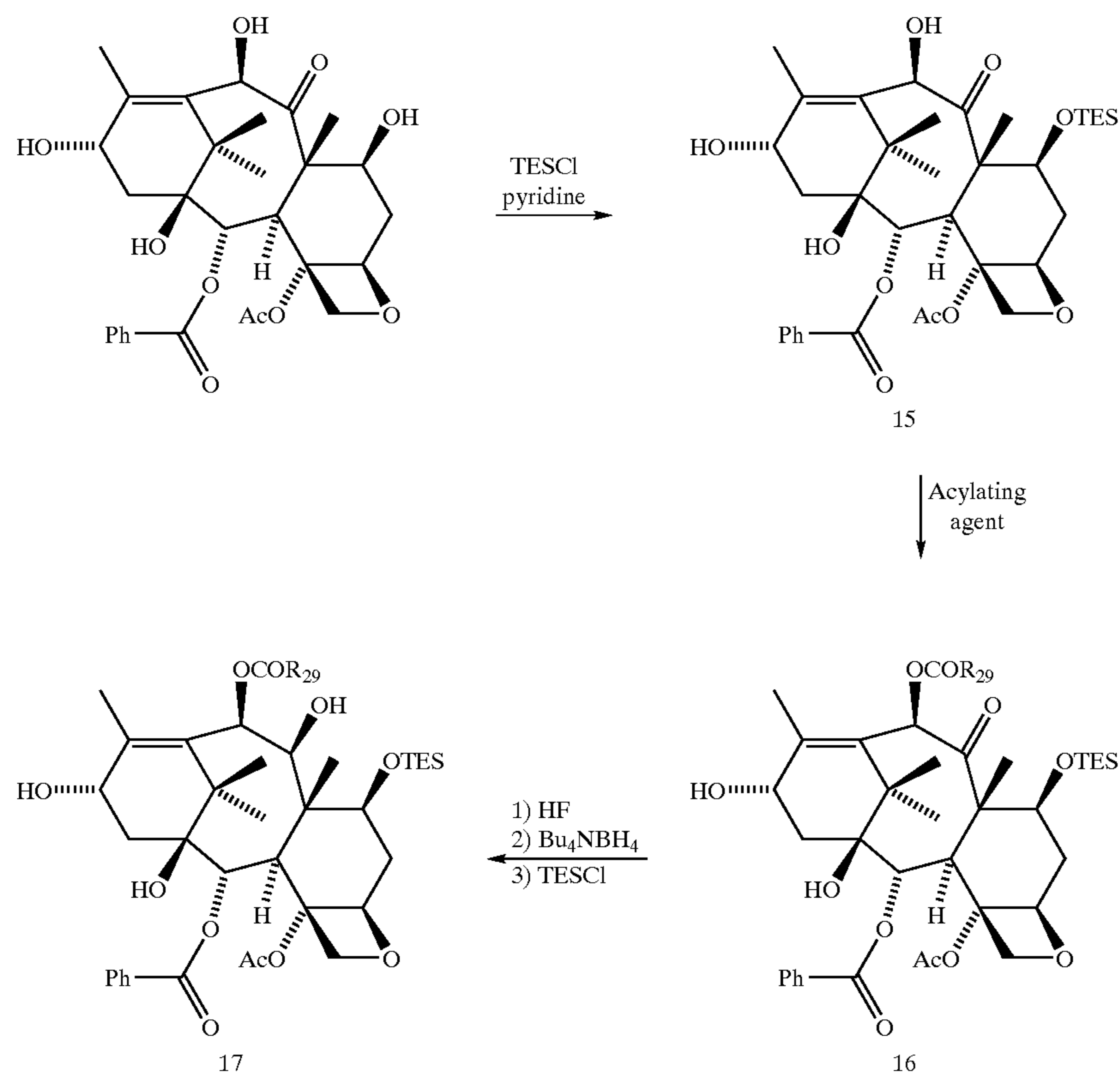
REACTION SCHEME 5
