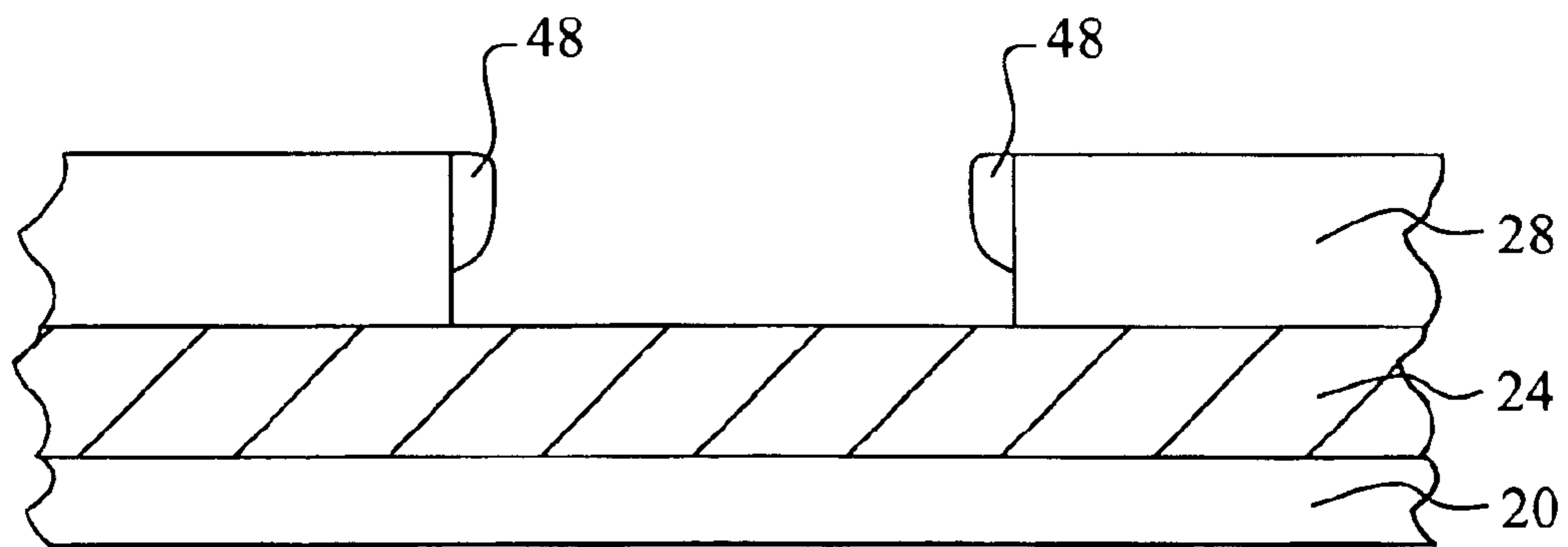
FIG. 4 Prior Art
