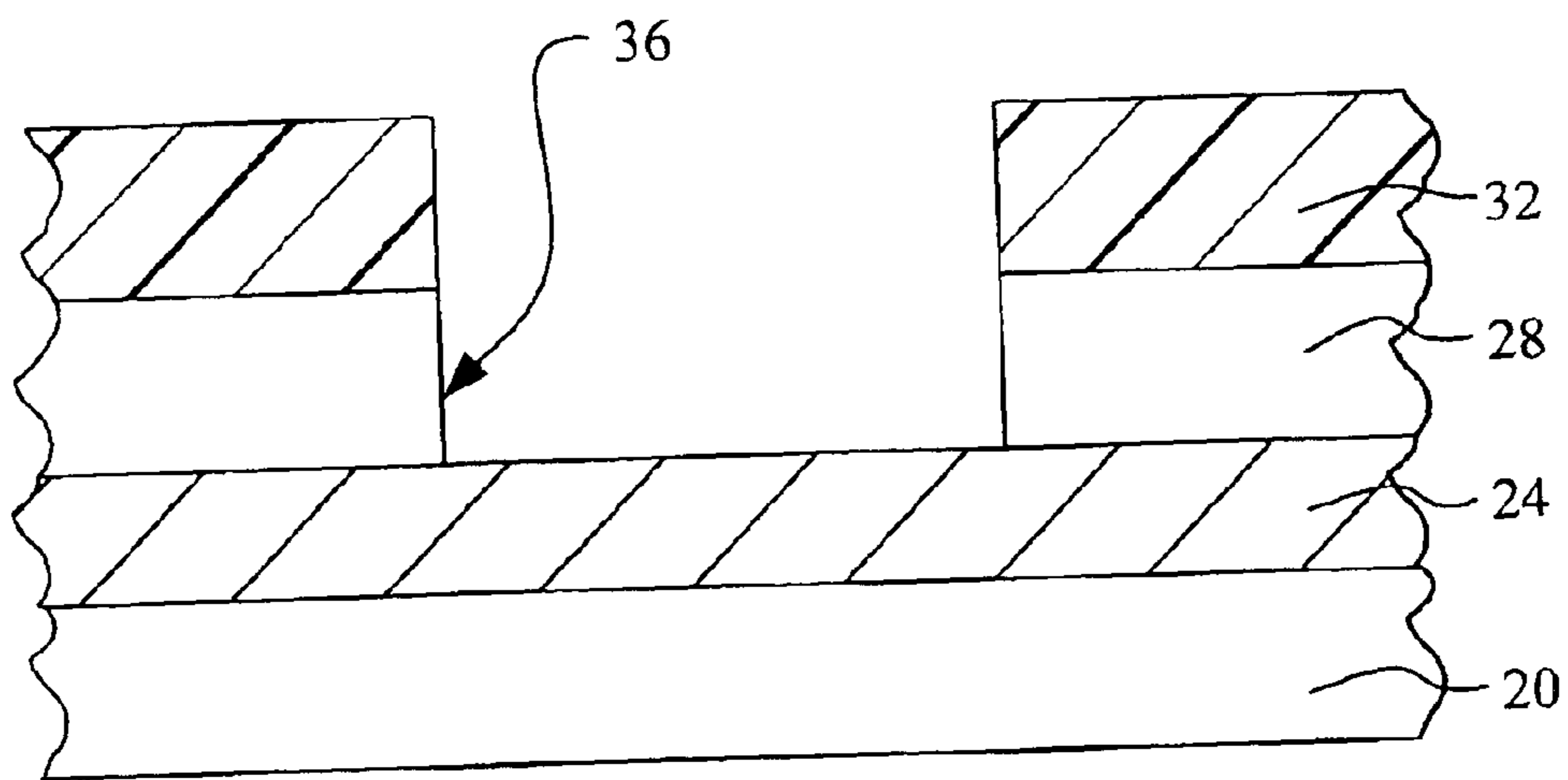
FIG. 2 Prior Art
