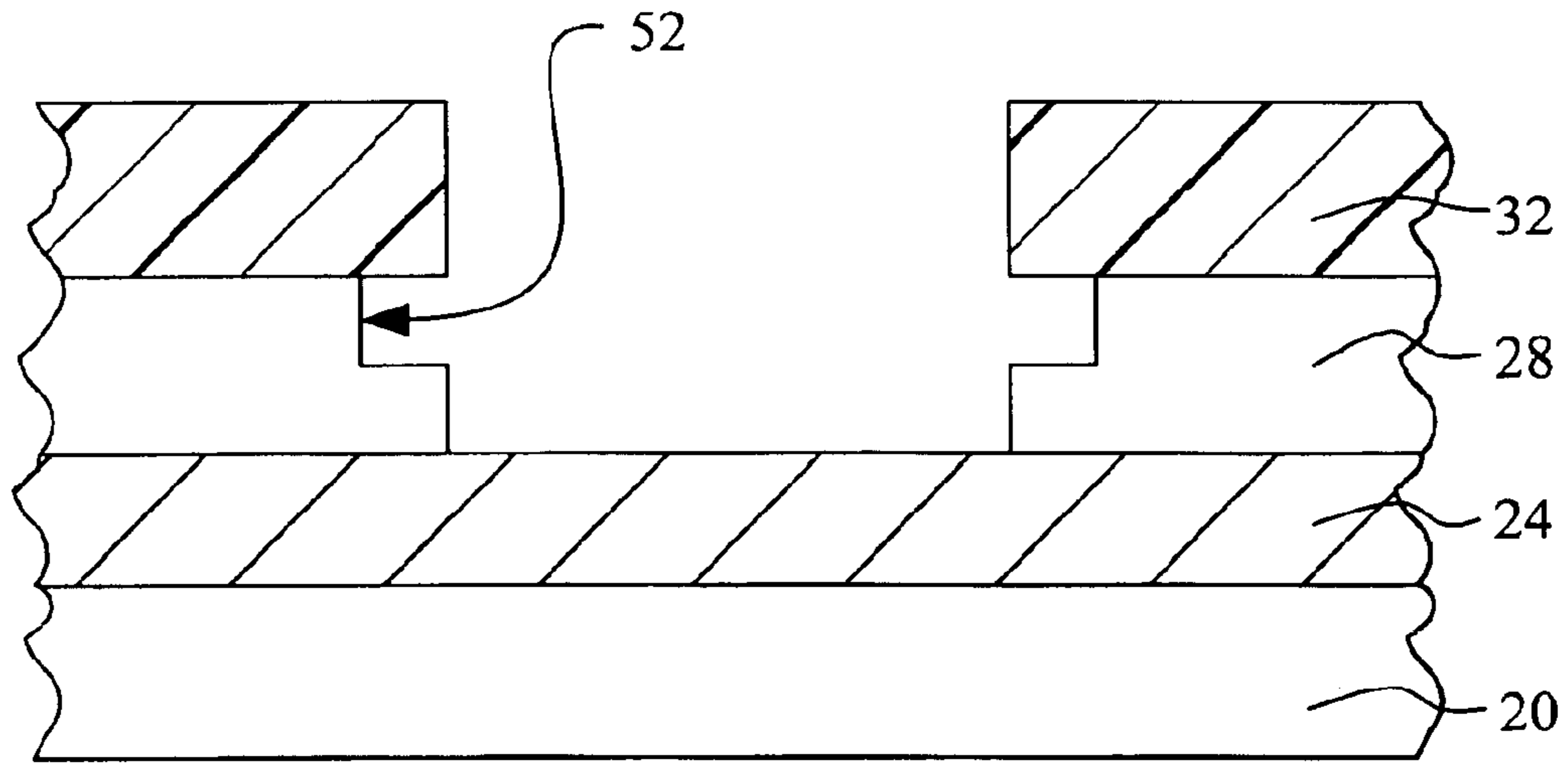
FIG. 5 Prior Art
