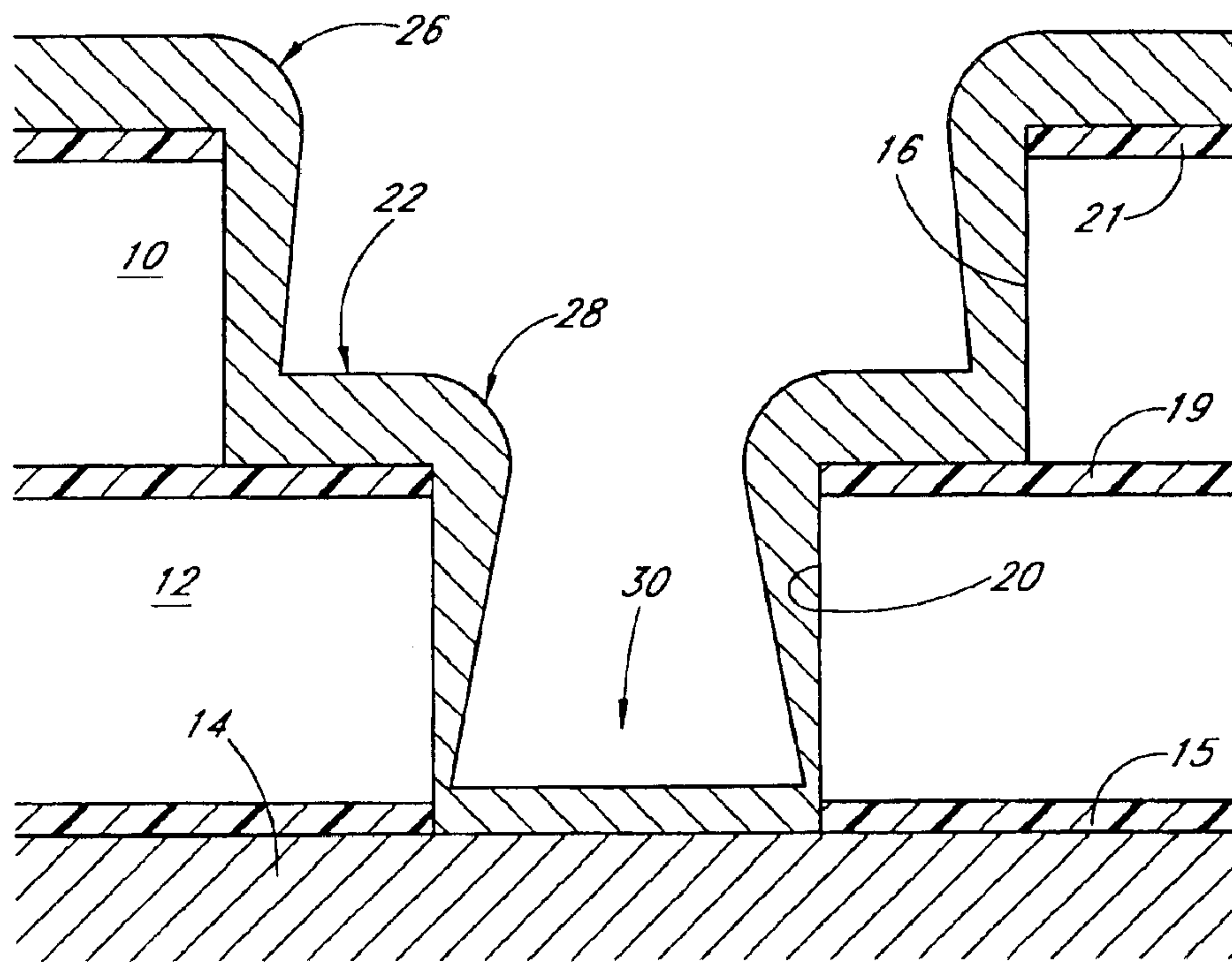
FIG. 1 (PRIOR ART)
