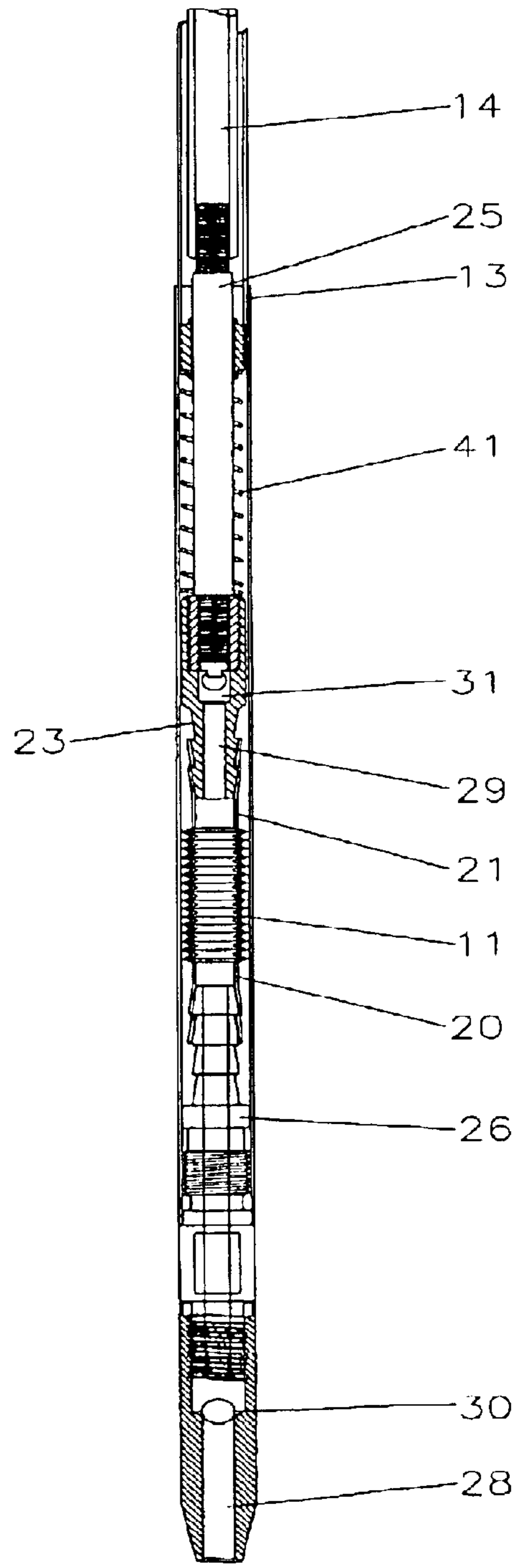
(b) DOWNSTROKE BLADDER COMPRESSING
