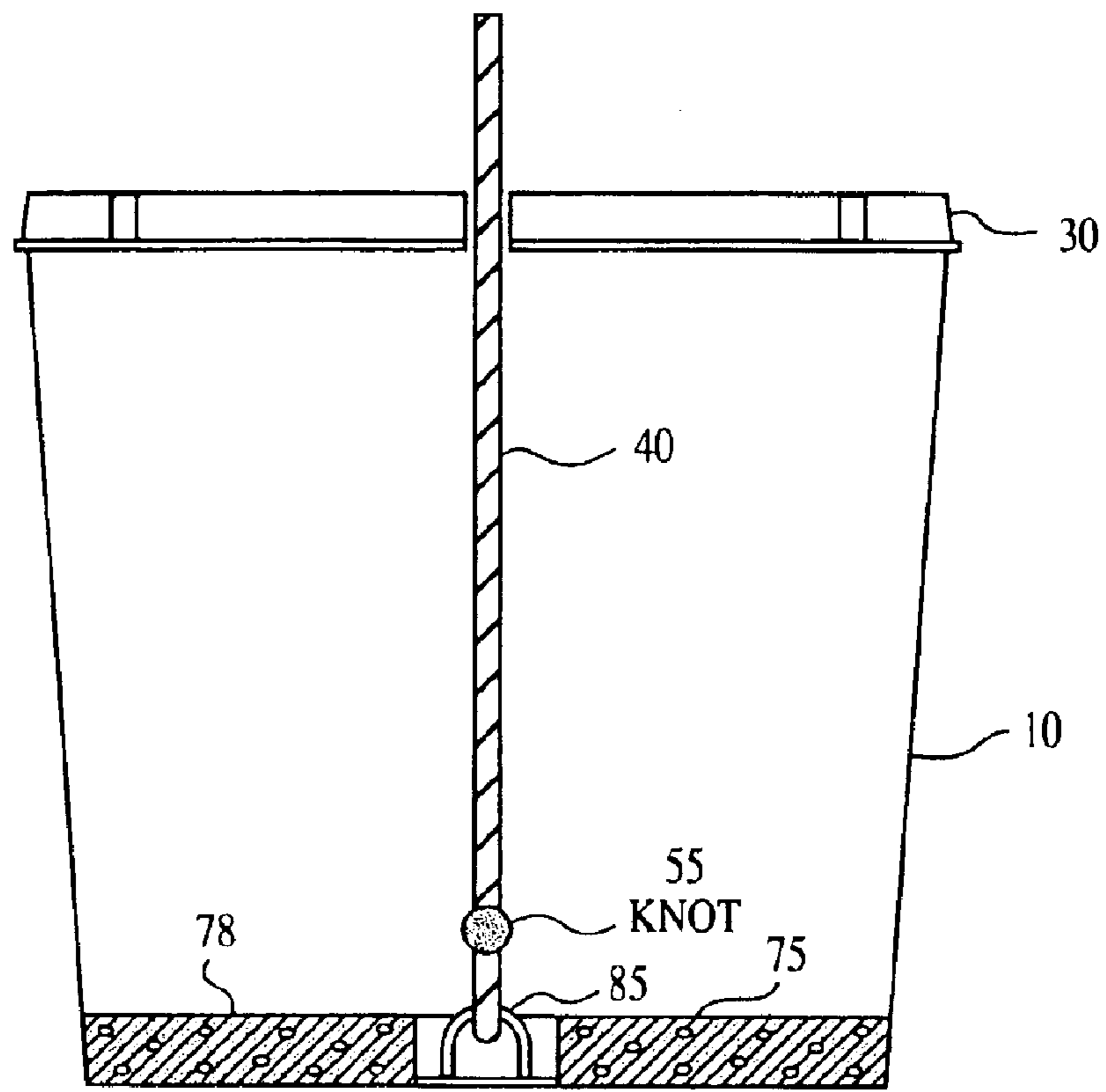
SECTION OF BUCKET
