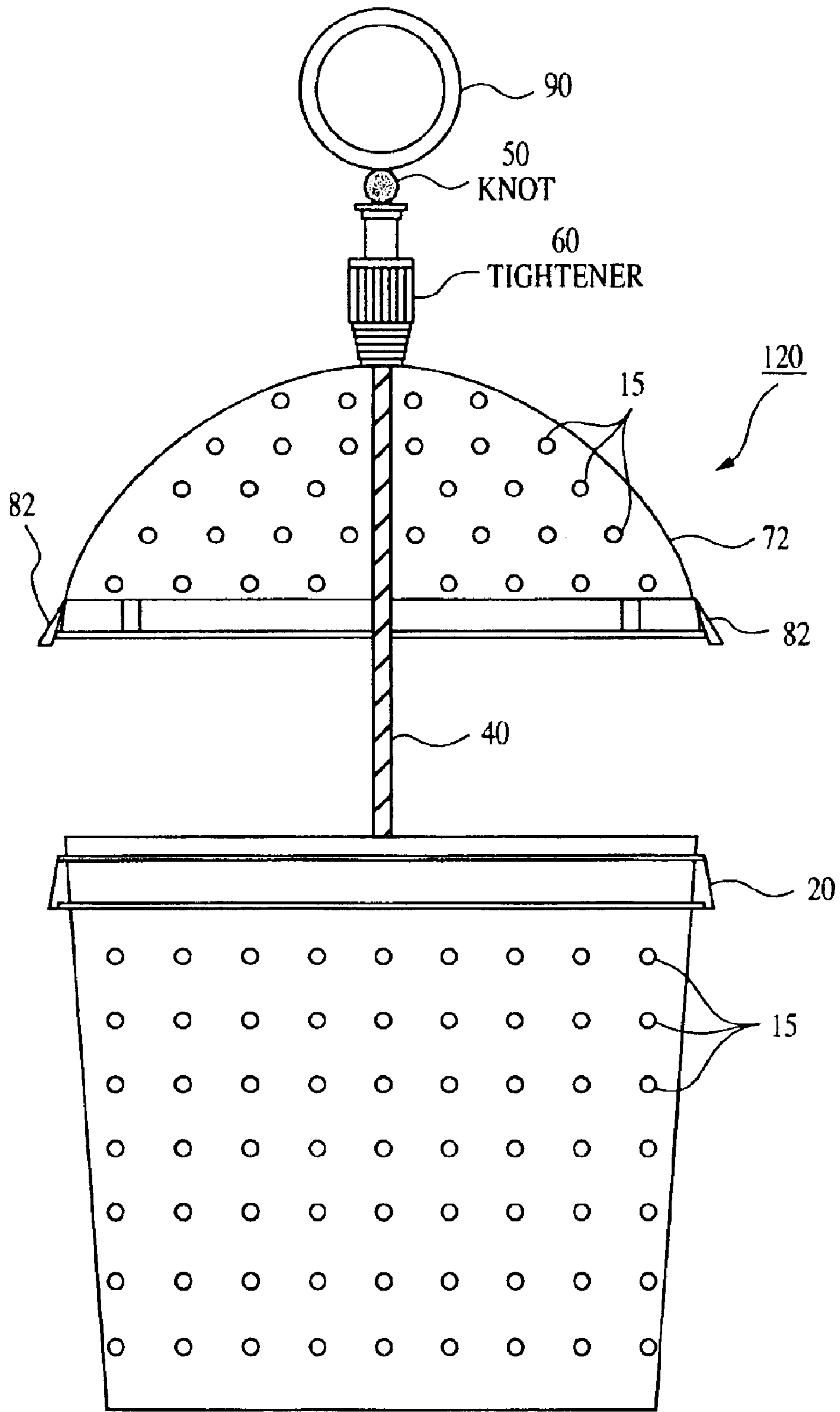
OPEN BUCKET ELEVATION
