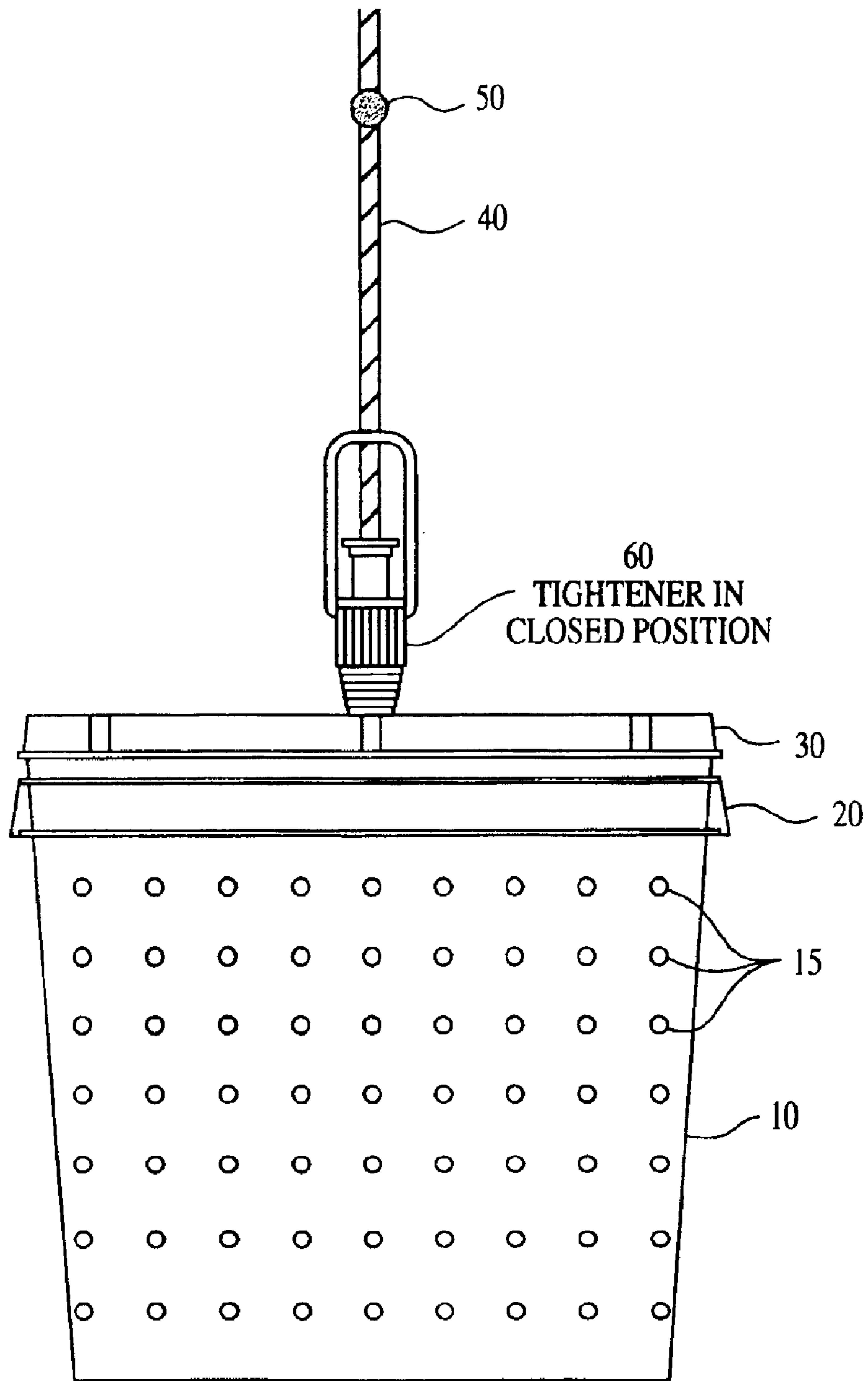
CLOSED BUCKET ELEVATION
