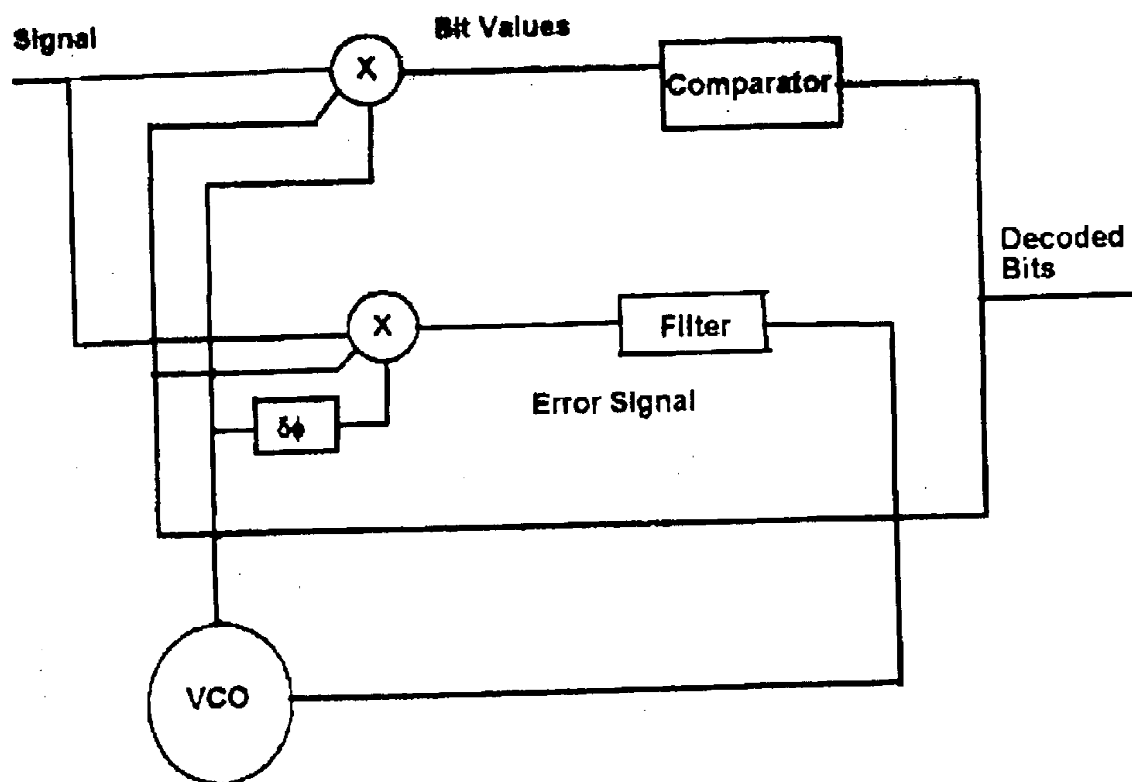
Fig. 4 (Prior Art)
