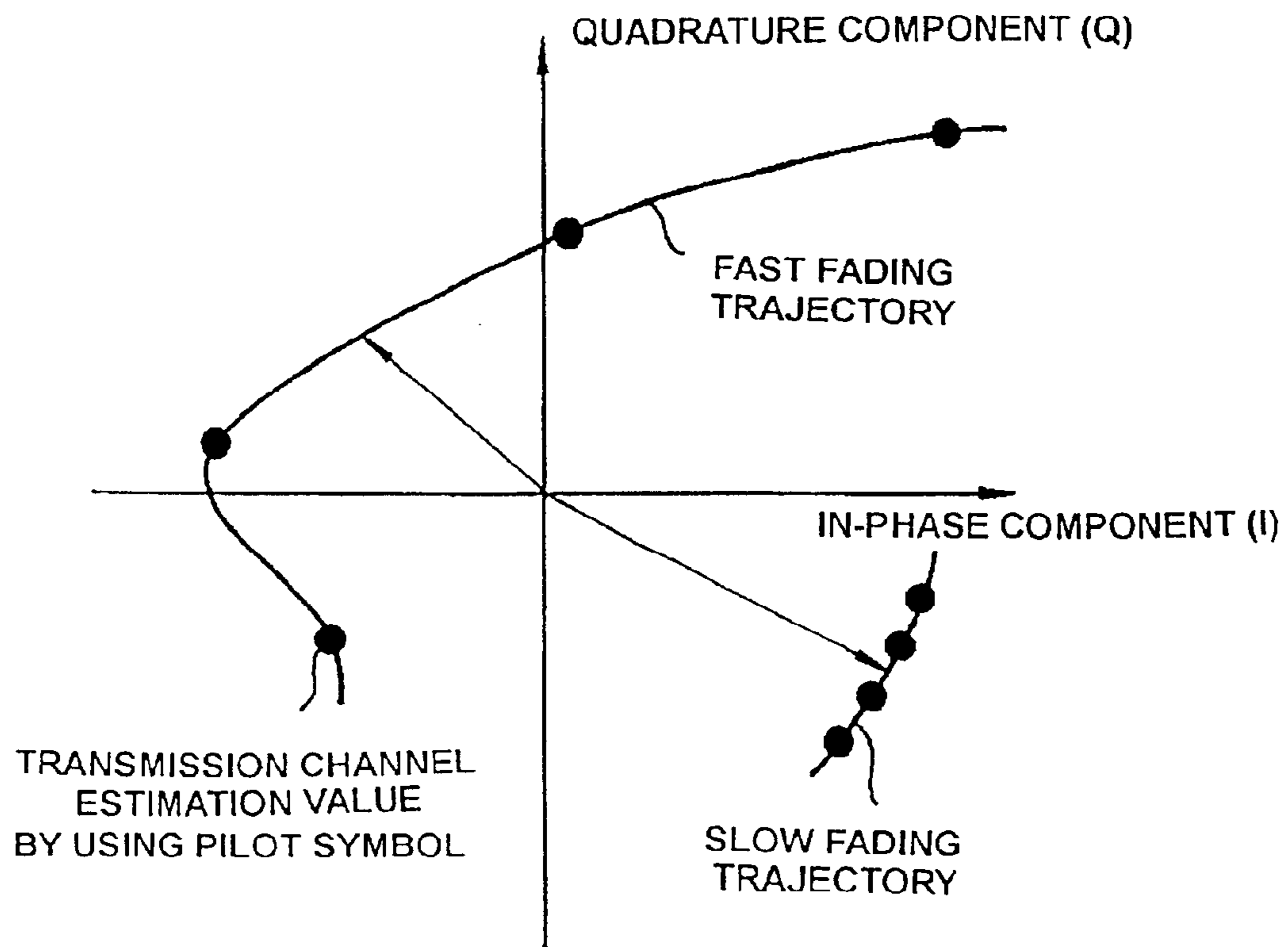
FIG. 6 (PRIOR ART)
