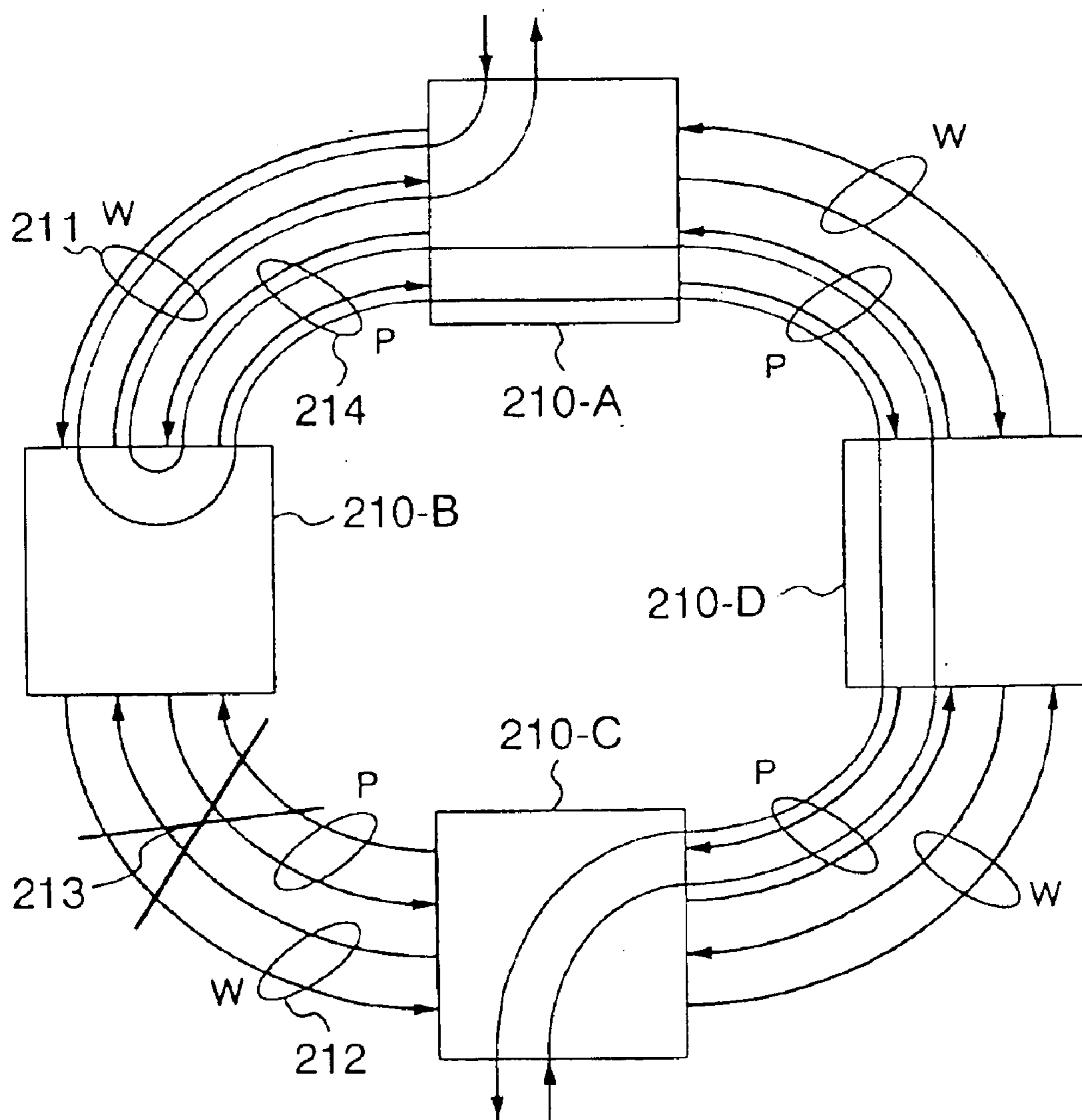
LINE SWITCH FUNCTION (SWITCHED AT 4-FIBER BLSR FAULT TIME)
