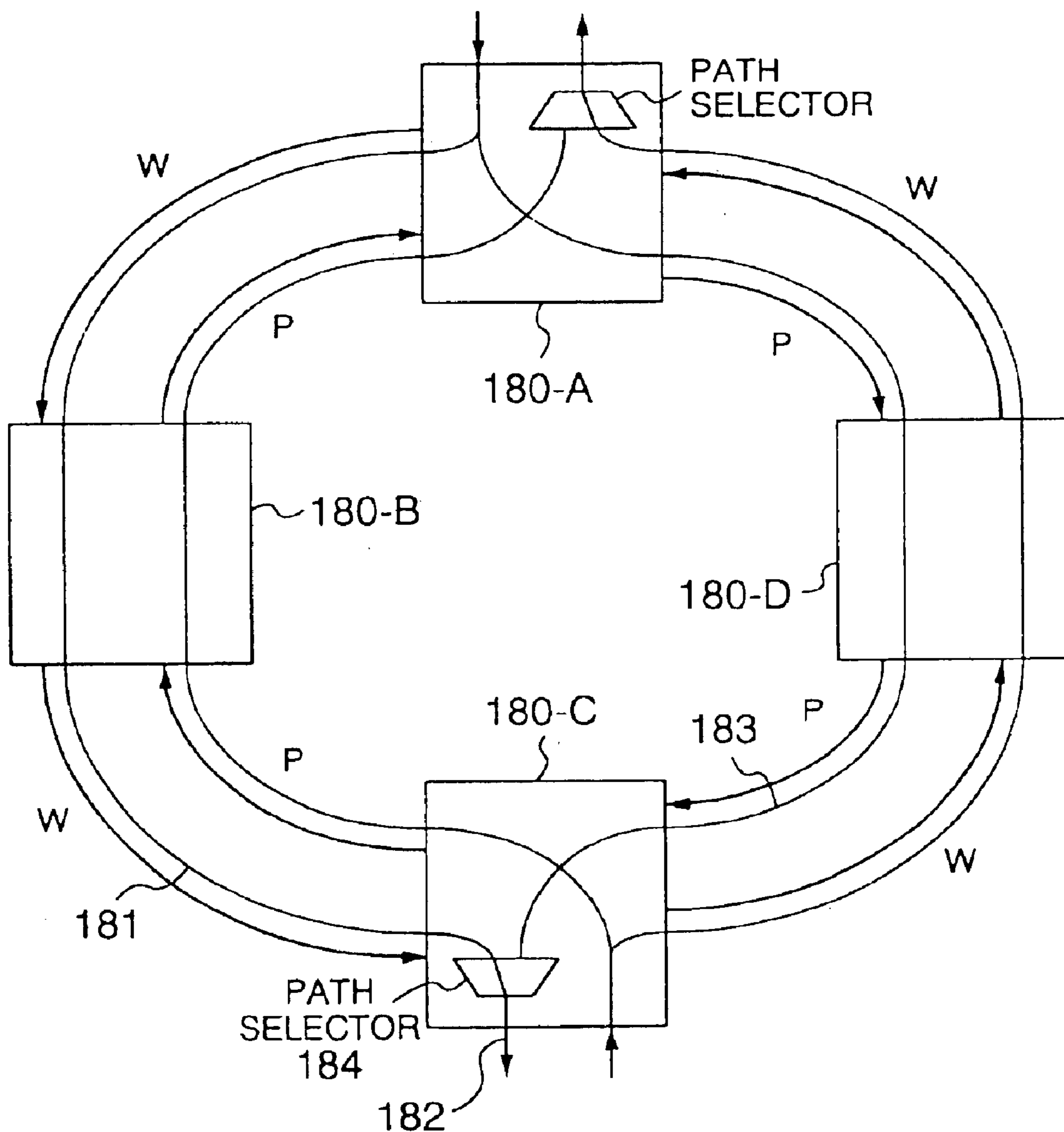
PATH SWITCH FUNCTION (UPSR UNDER NORMAL CONDITION)
