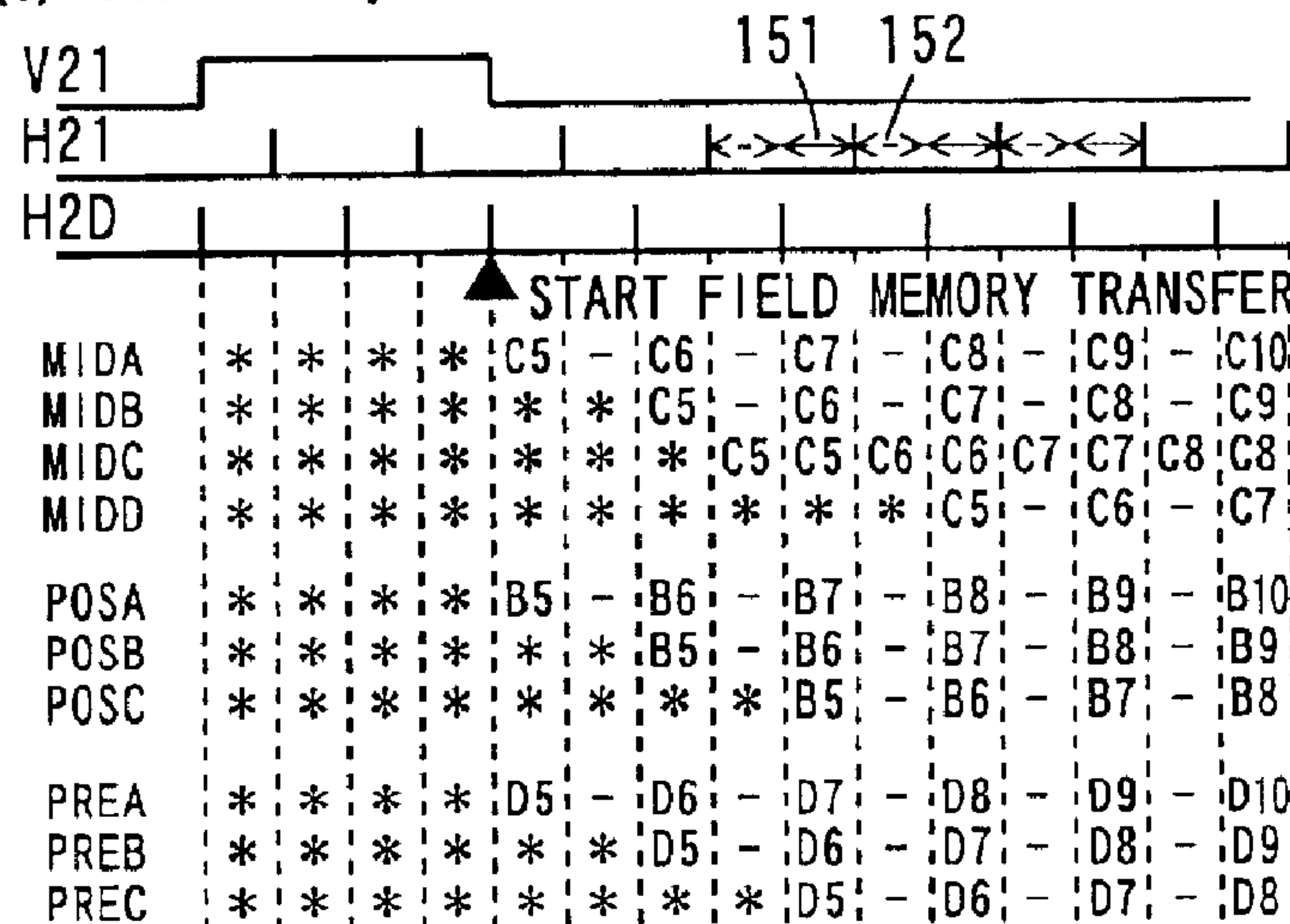
(c) OUTPUT SEQUENCE FROM FIELD MEMORY (EVEN FIELD)
