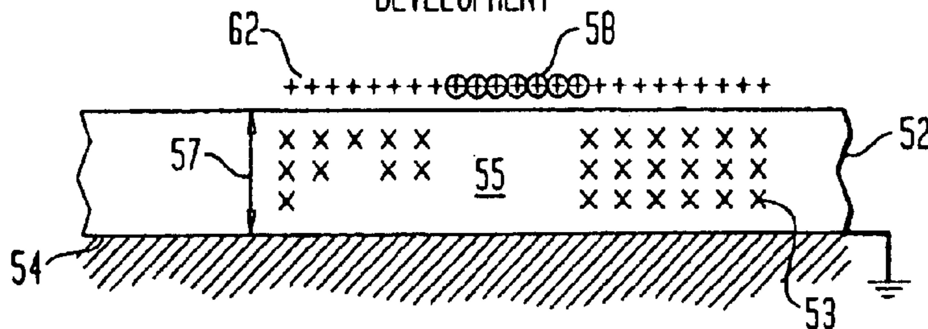
FIG. 3D LIQUID TONER DEVELOPMENT
