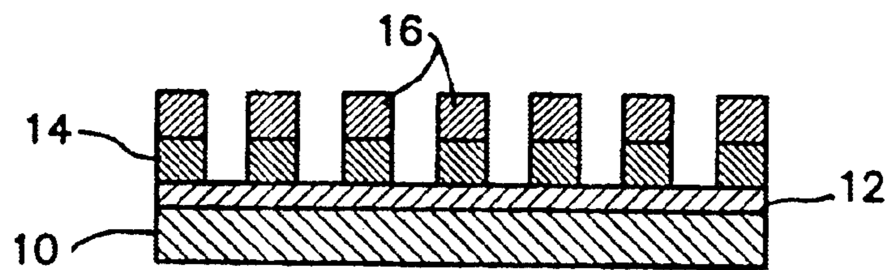
FIG. 2 PRIOR ART
