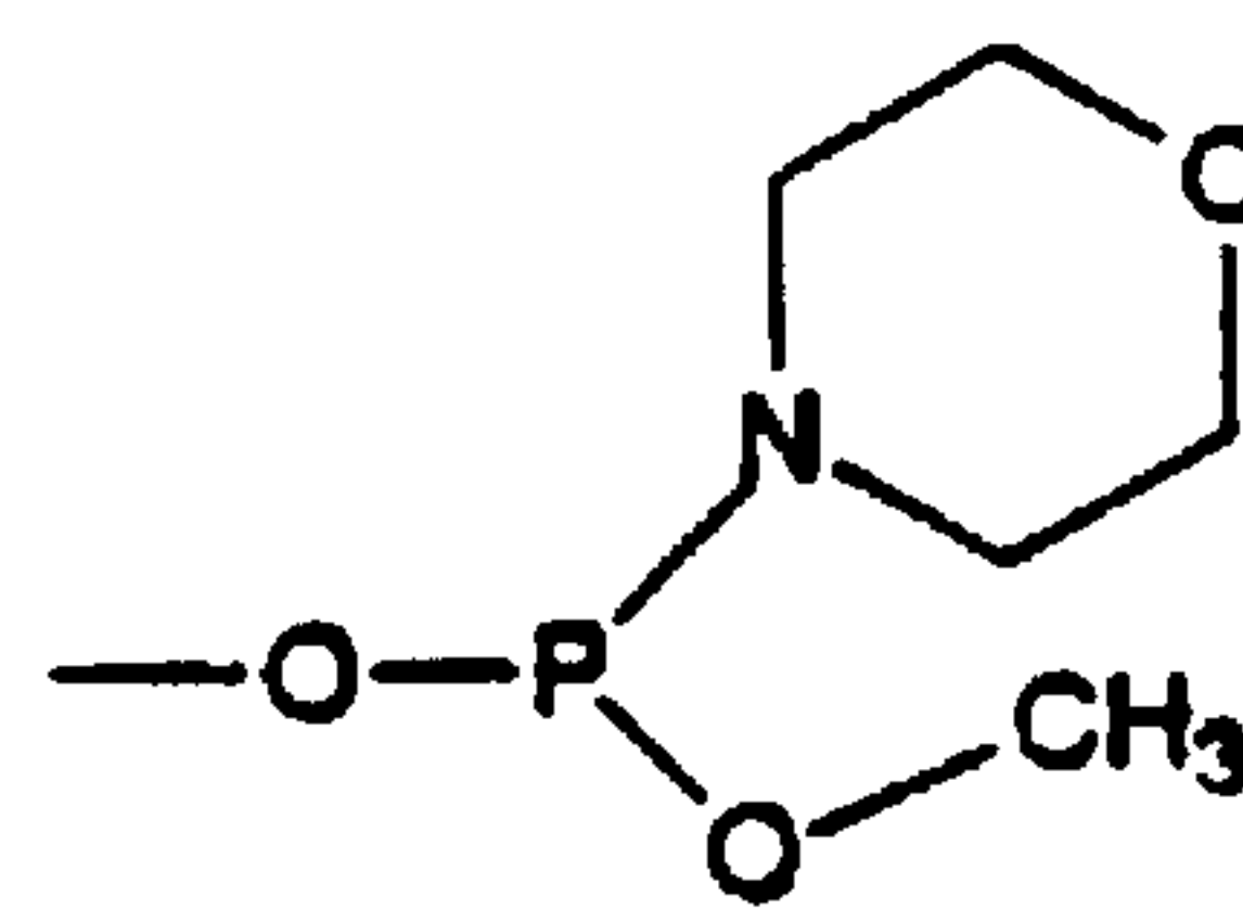
N-morpholino methoxyphosphine
