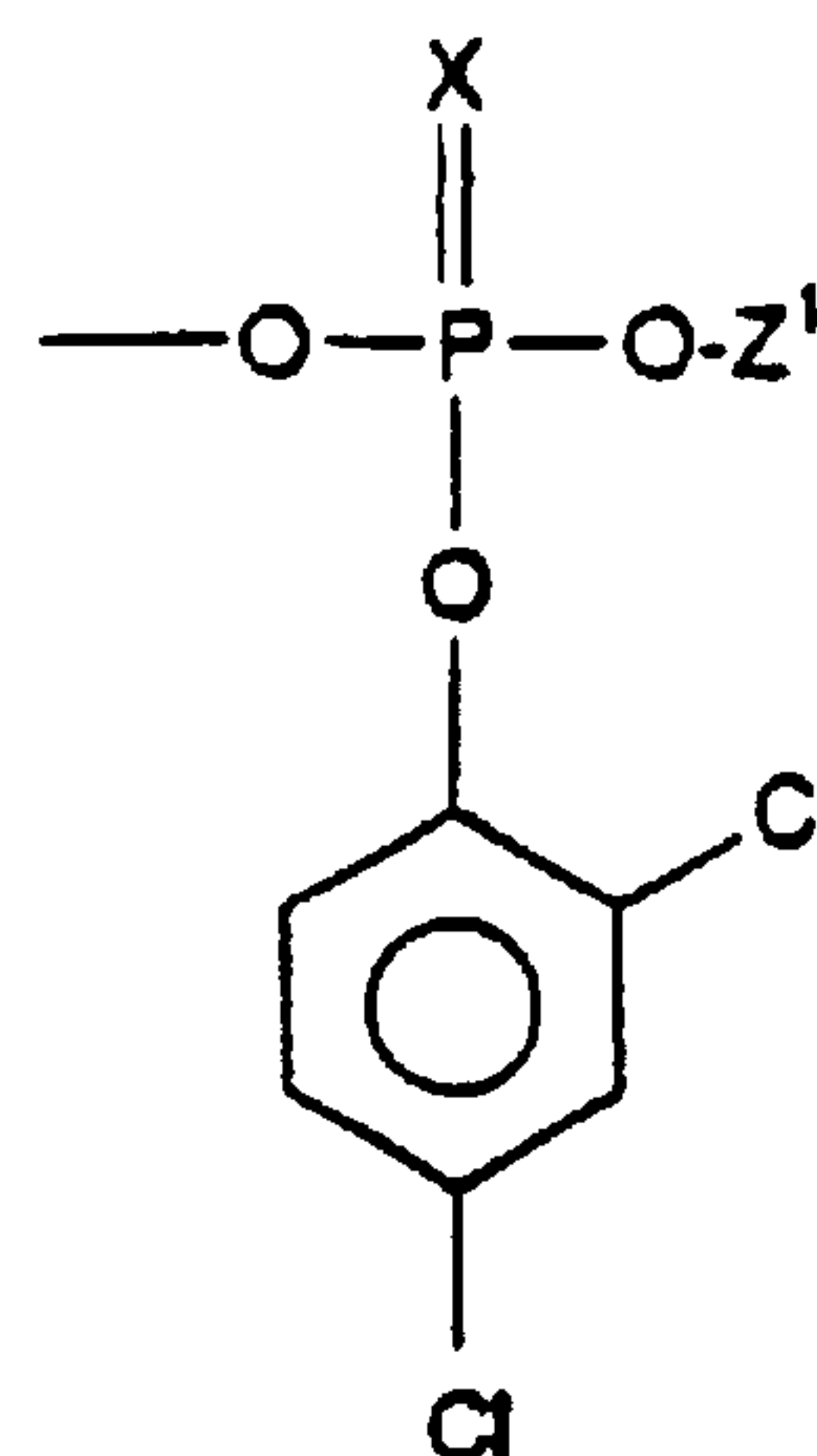
2,4-dichlorophenyl phosphate
