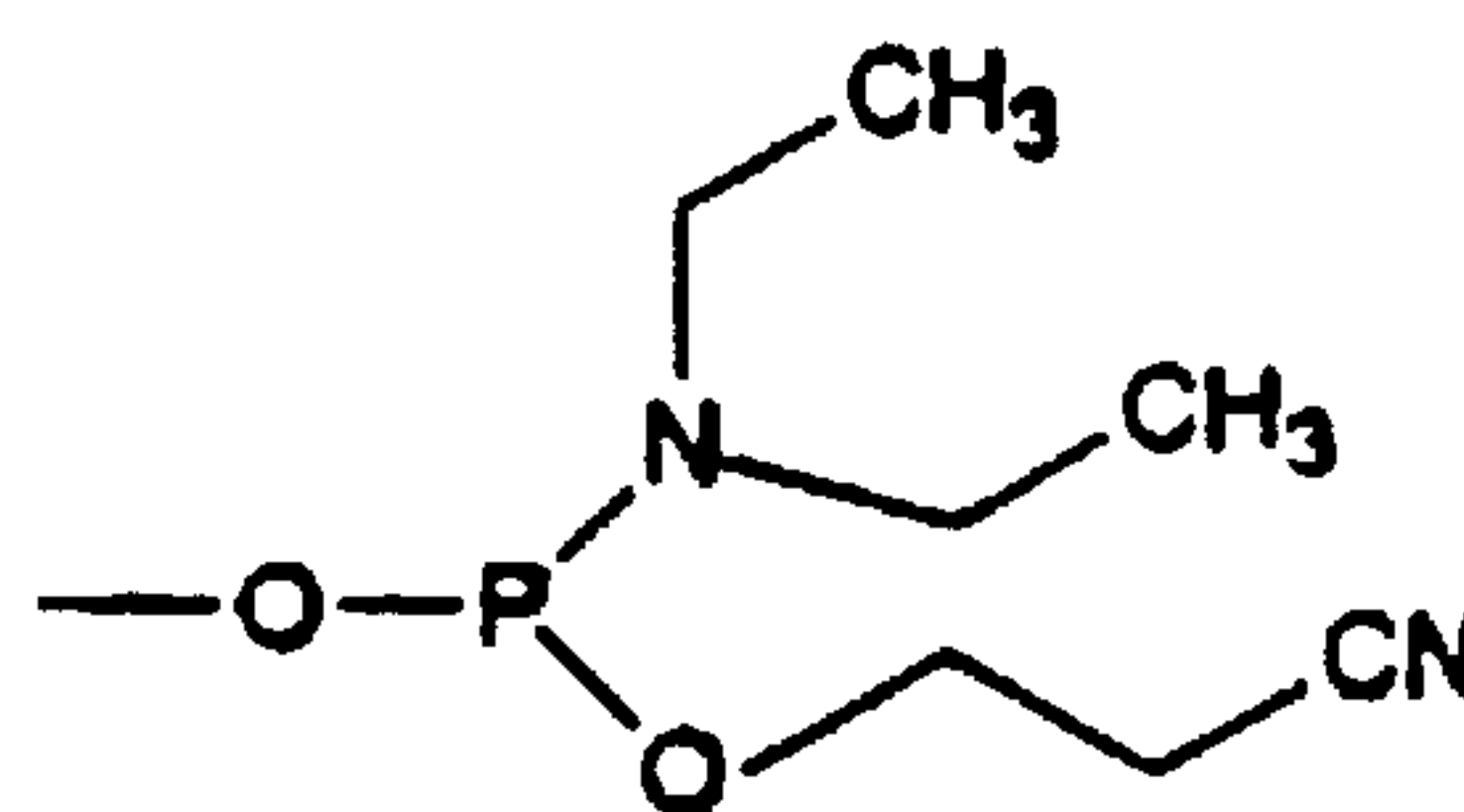
N,N-diethylamino-β-cyanoethoxyphosphine
