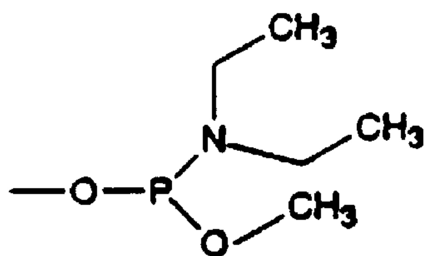
N,N-diethylamino-methoxyphosphine
