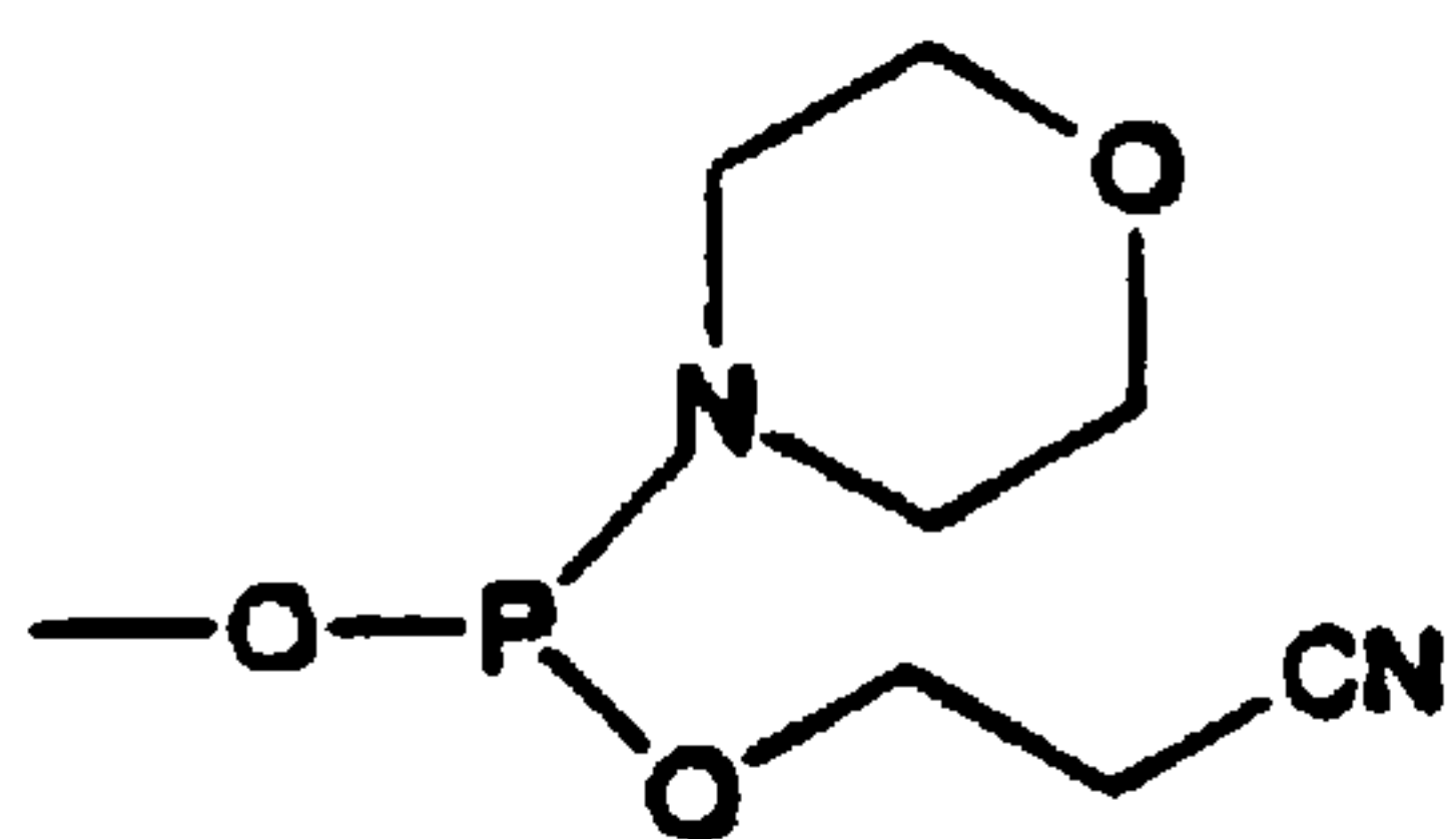
N-morpholino-β-cyanoethoxyphosphine
