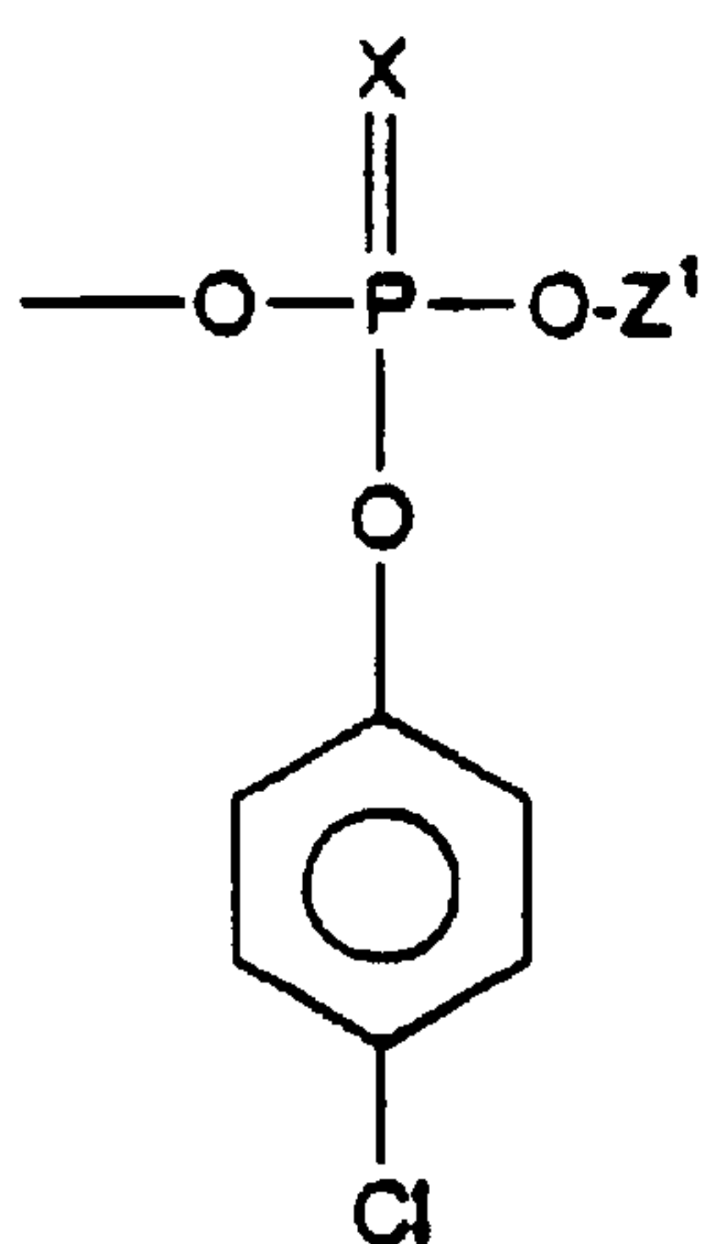
4-chlorophenyl phosphate
