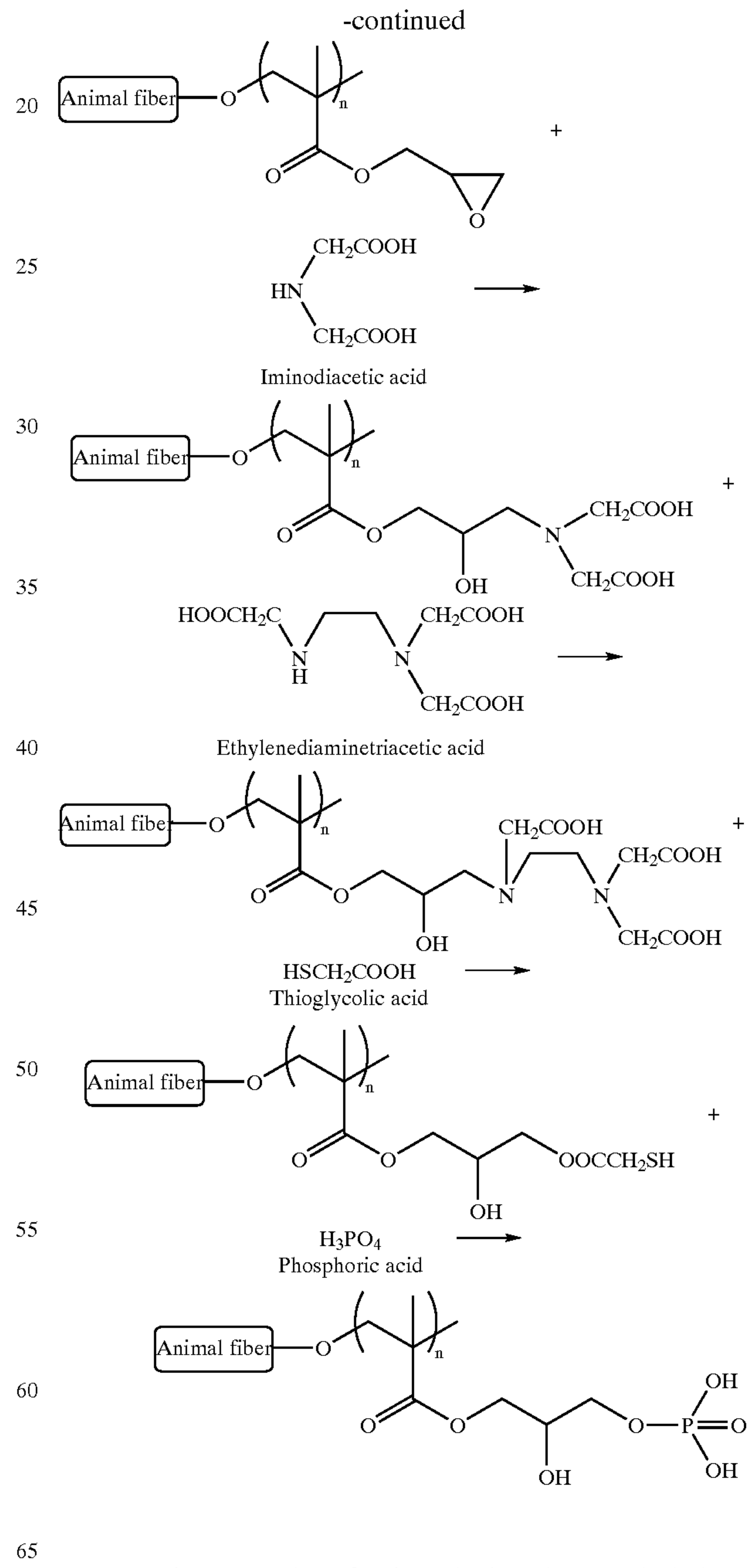
A reaction procedure for introducing the metal chelate-forming functional group into a molecule of a natural fiber
