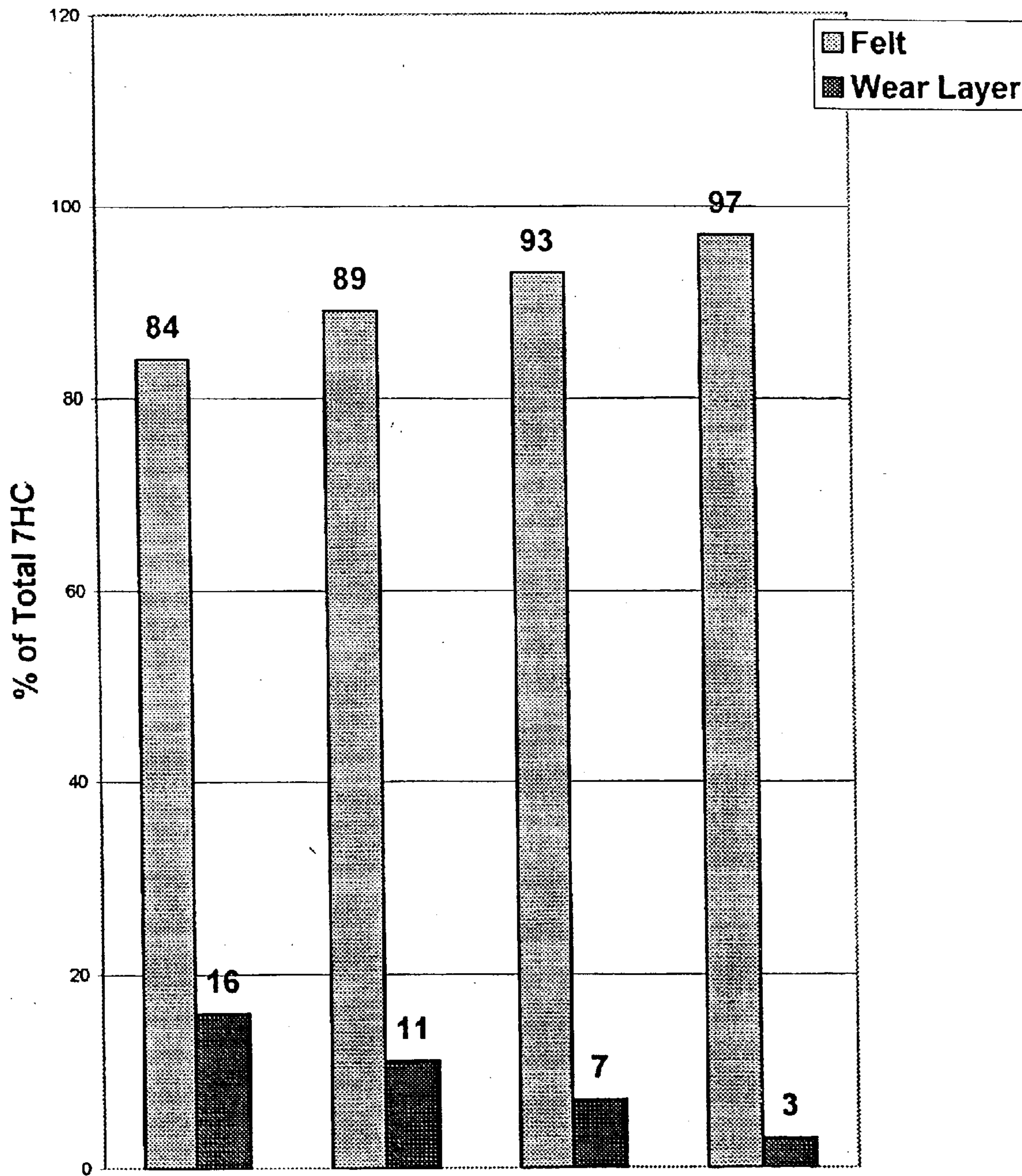
Weight % Activated Charcoal in Felt FIG. 4
