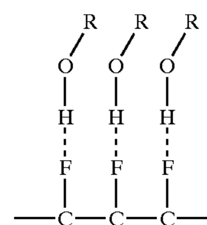
Scheme 1
