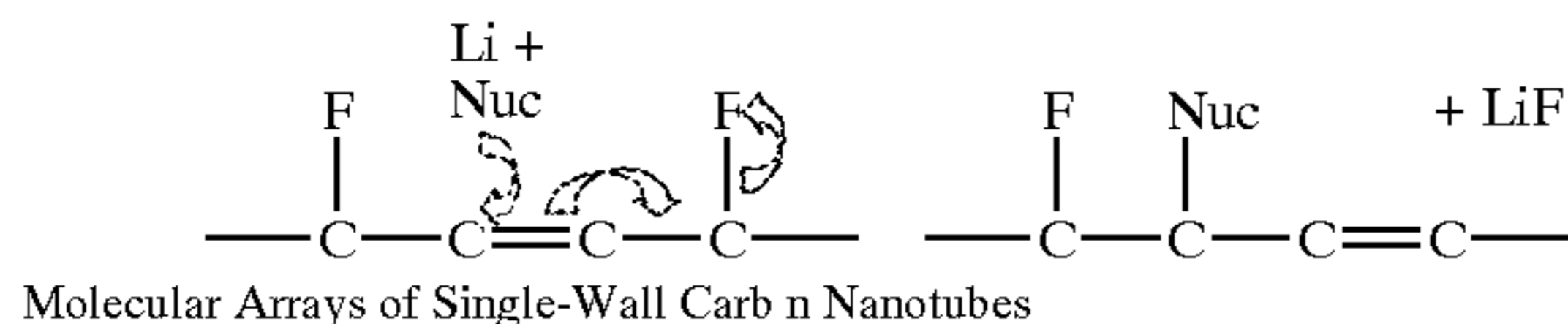
Scheme 2
