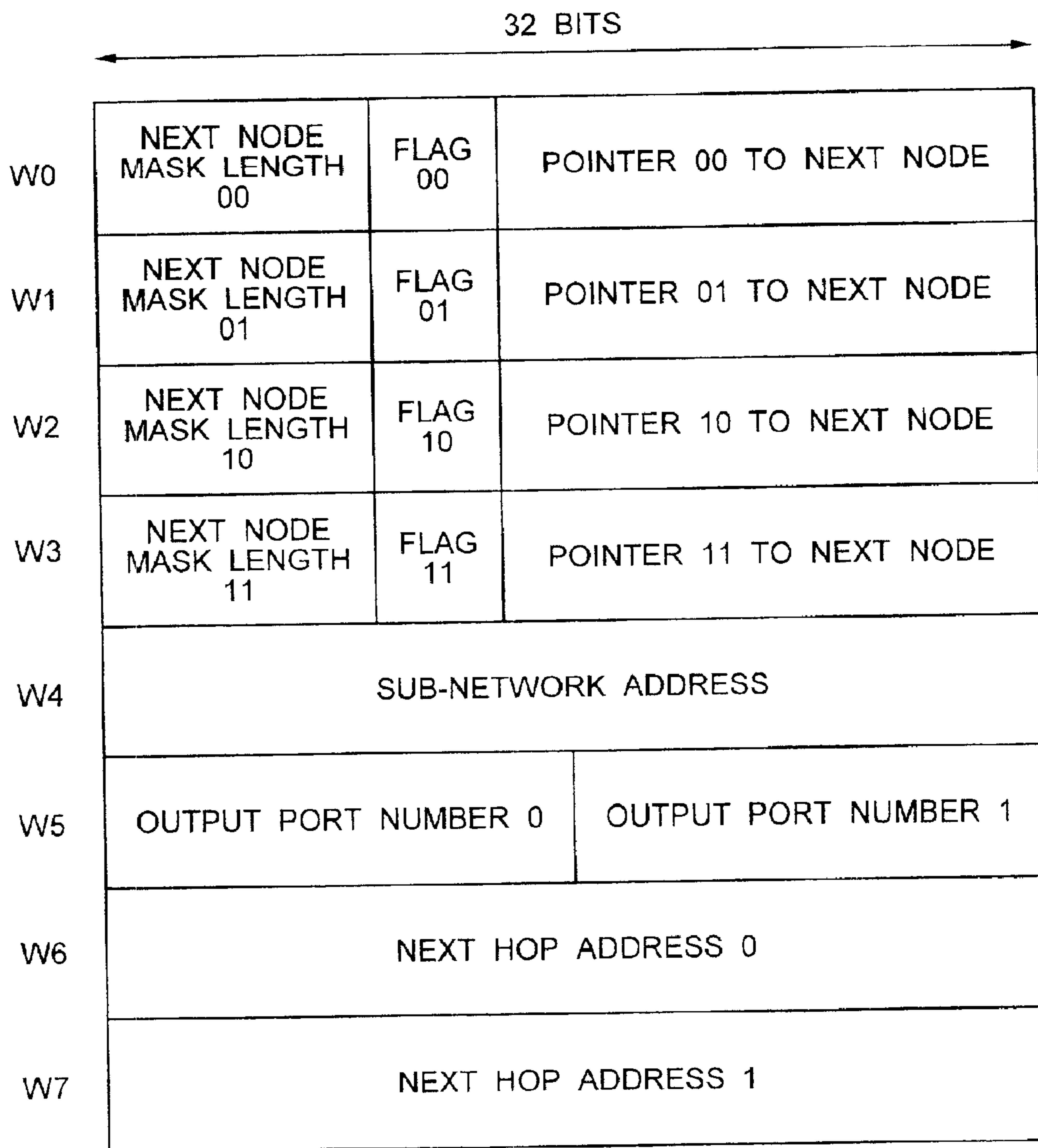
4-BRANCH TREE NODE
