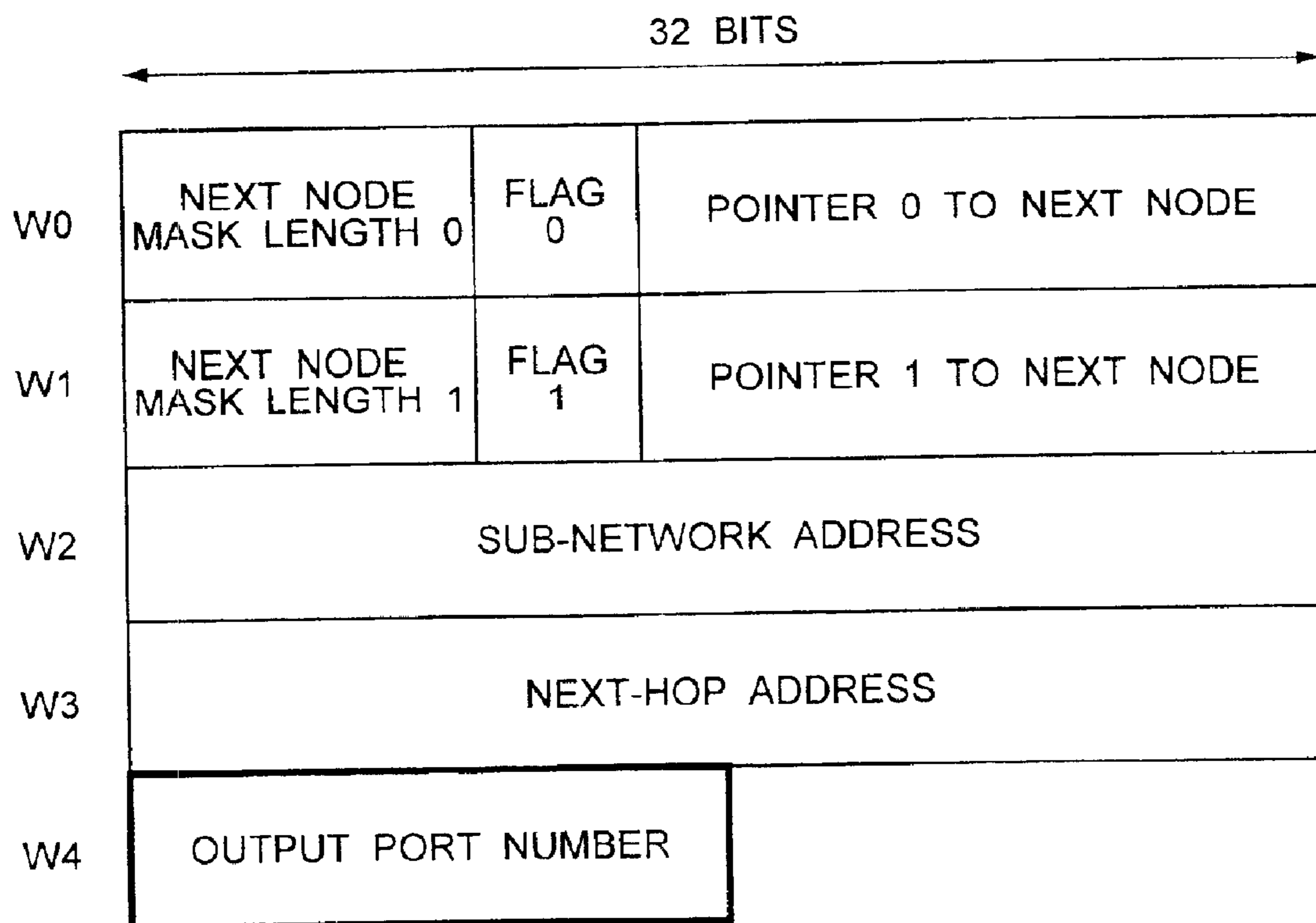
2-BRANCH TREE NODE
