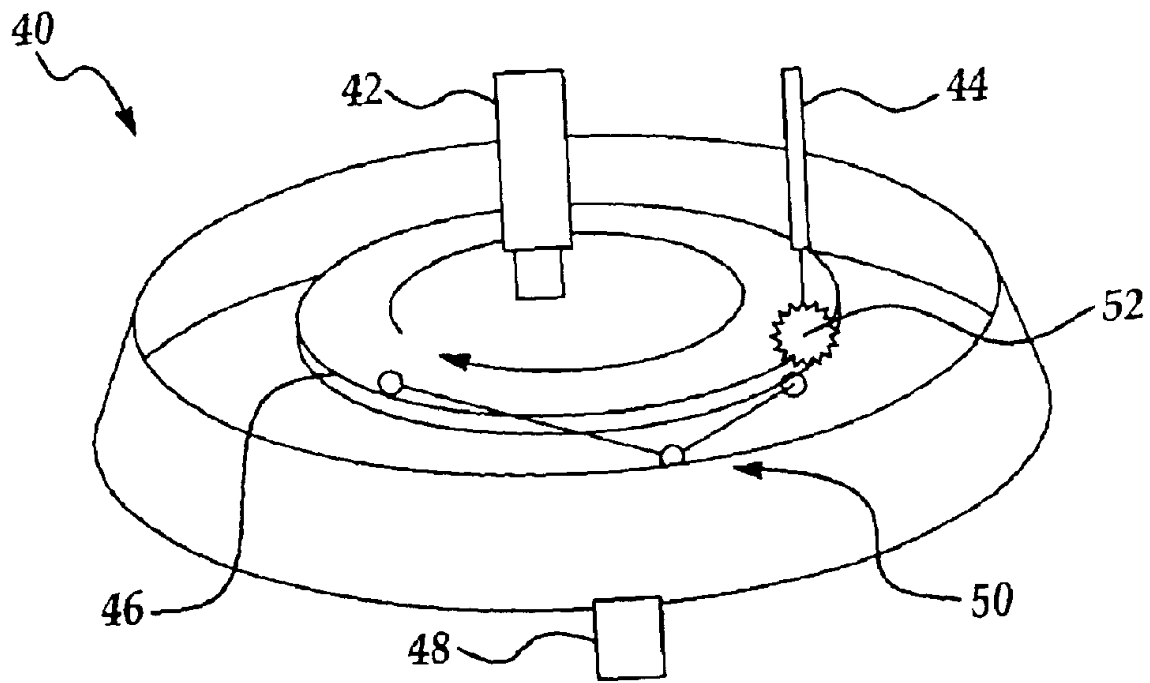
Figure 2 Prior Art
