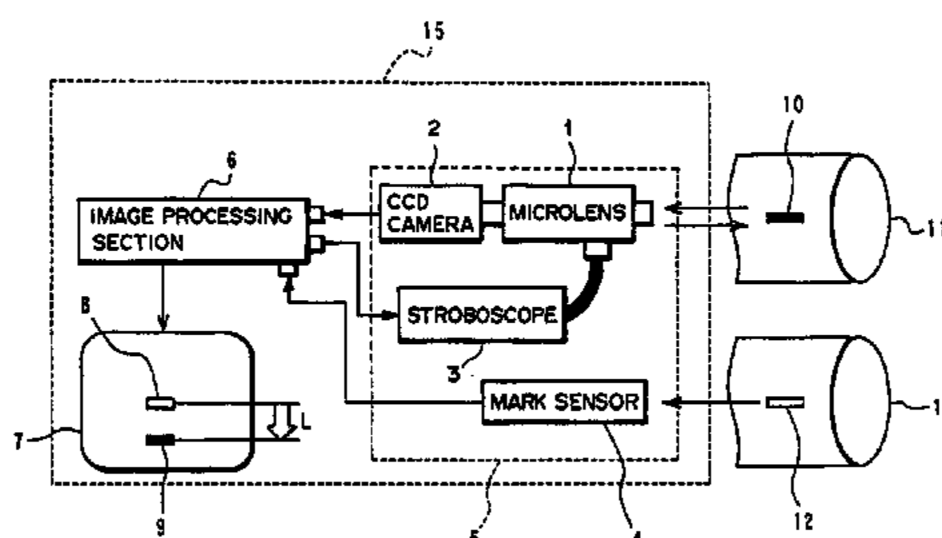
BLOCK DIAGRAM OF A ROTATIONAL PHASE DIFFERENCE DETECTING SYSTEM OF A FIRST EMBODIMENT OF THE PRESENT INVENTION
