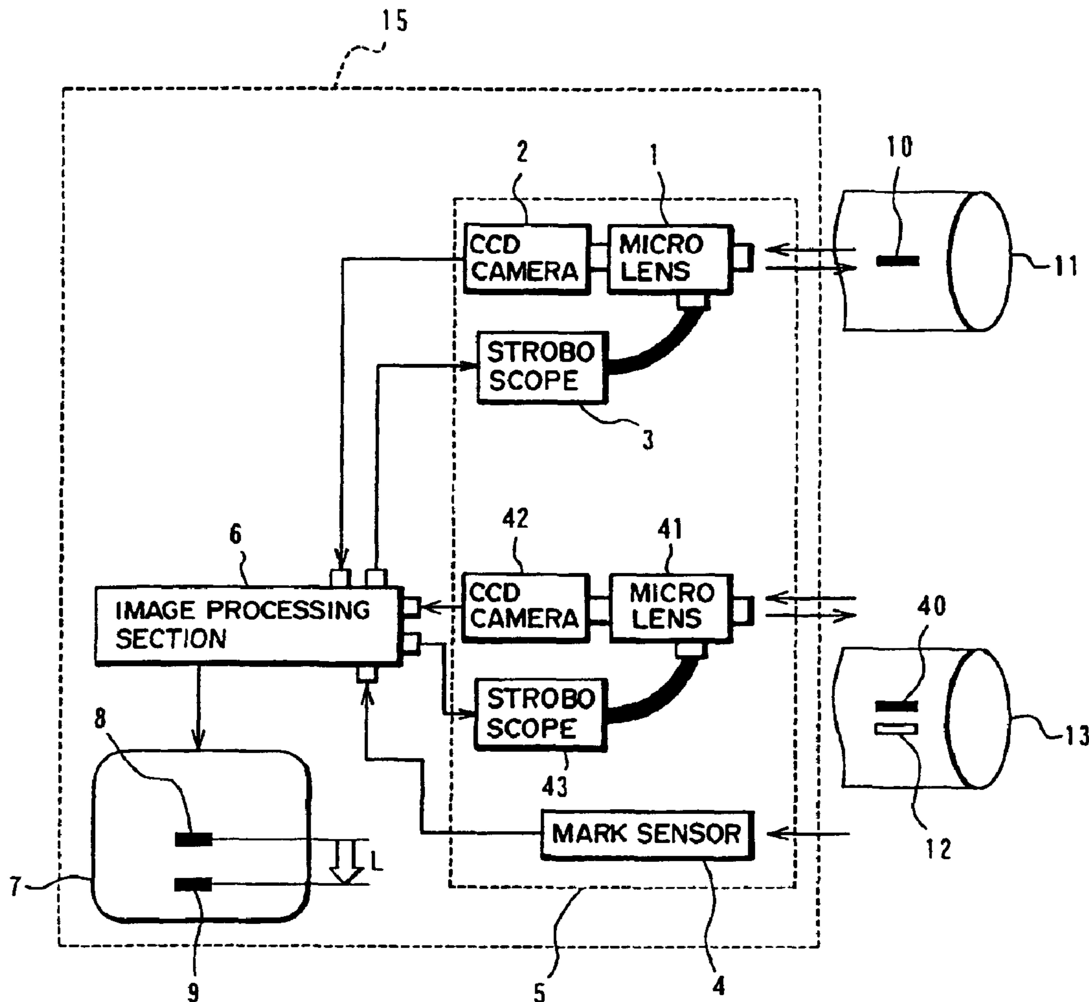
BLOCK DIAGRAM OF A ROTATIONAL PHASE DIFFERENCE DETECTING SYSTEM OF A SECOND EMBODIMENT OF THE PRESENT INVENTION
