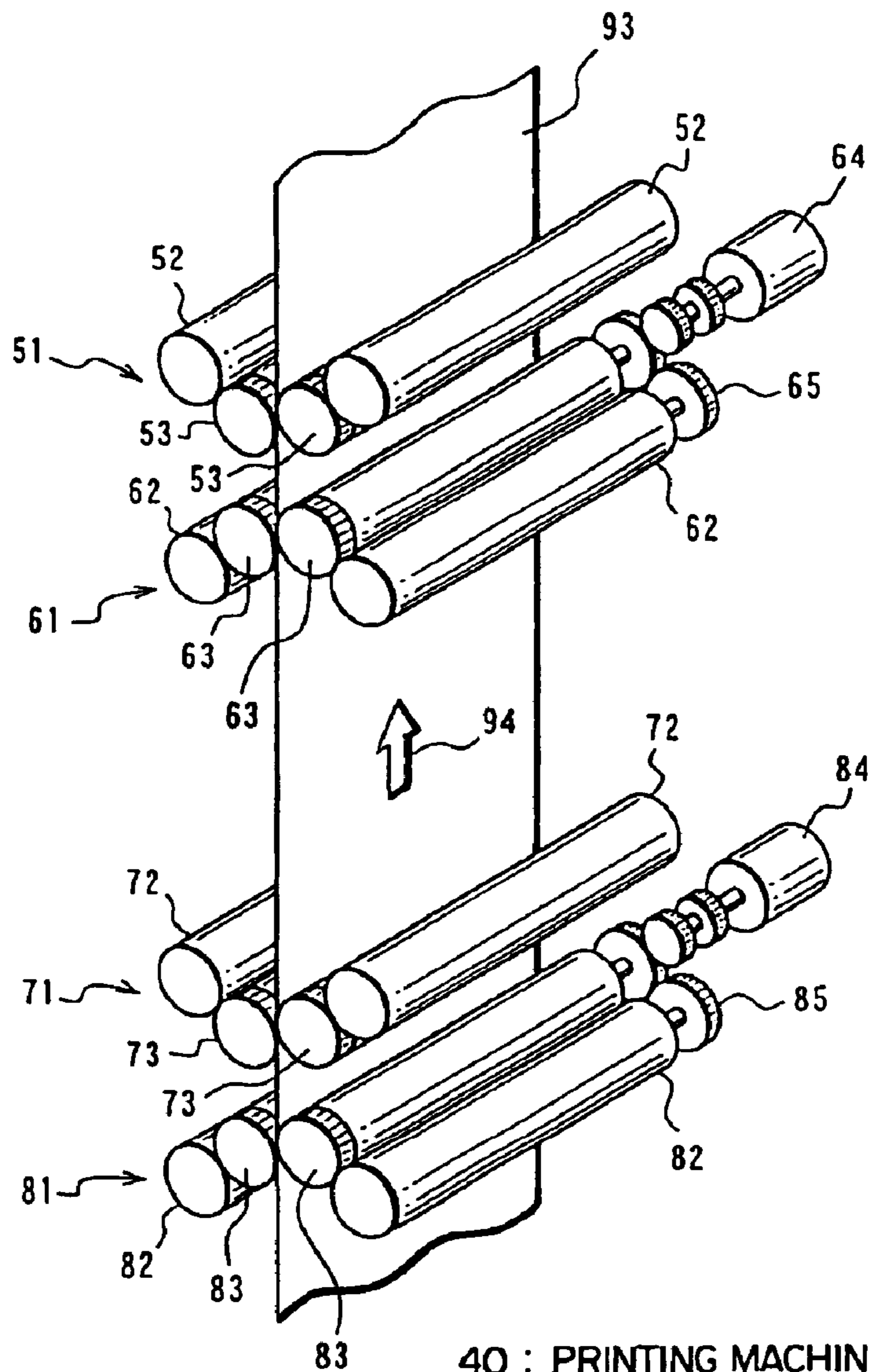
OUTLINE DIAGRAM OF AN OFFSET ROTARY PRINTING MACHINE
