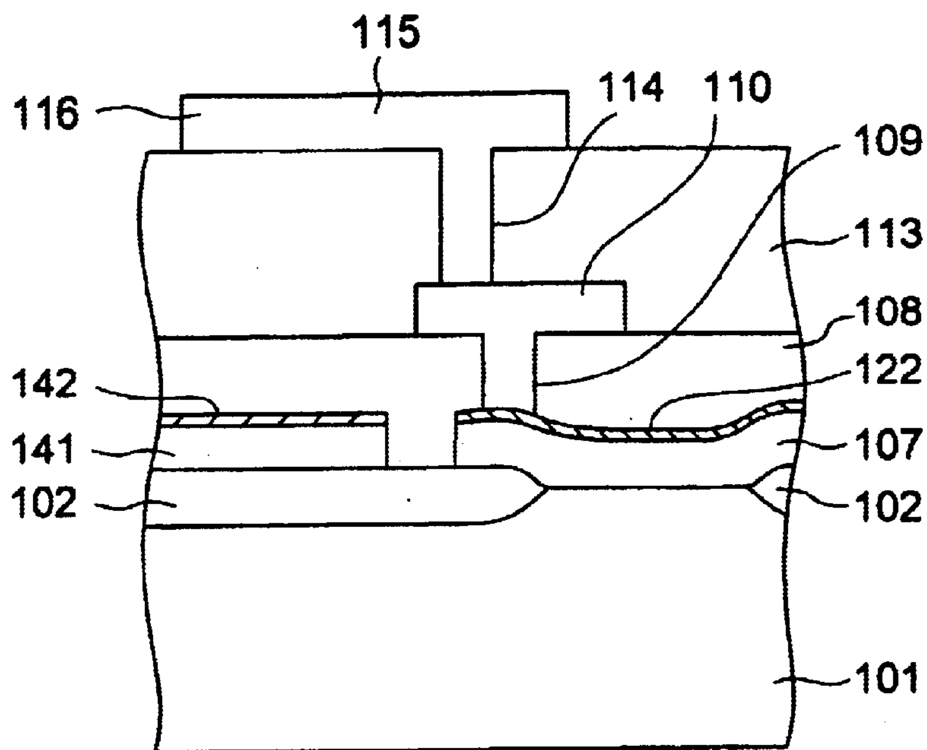
FIG. 6A c-c' SECTION
