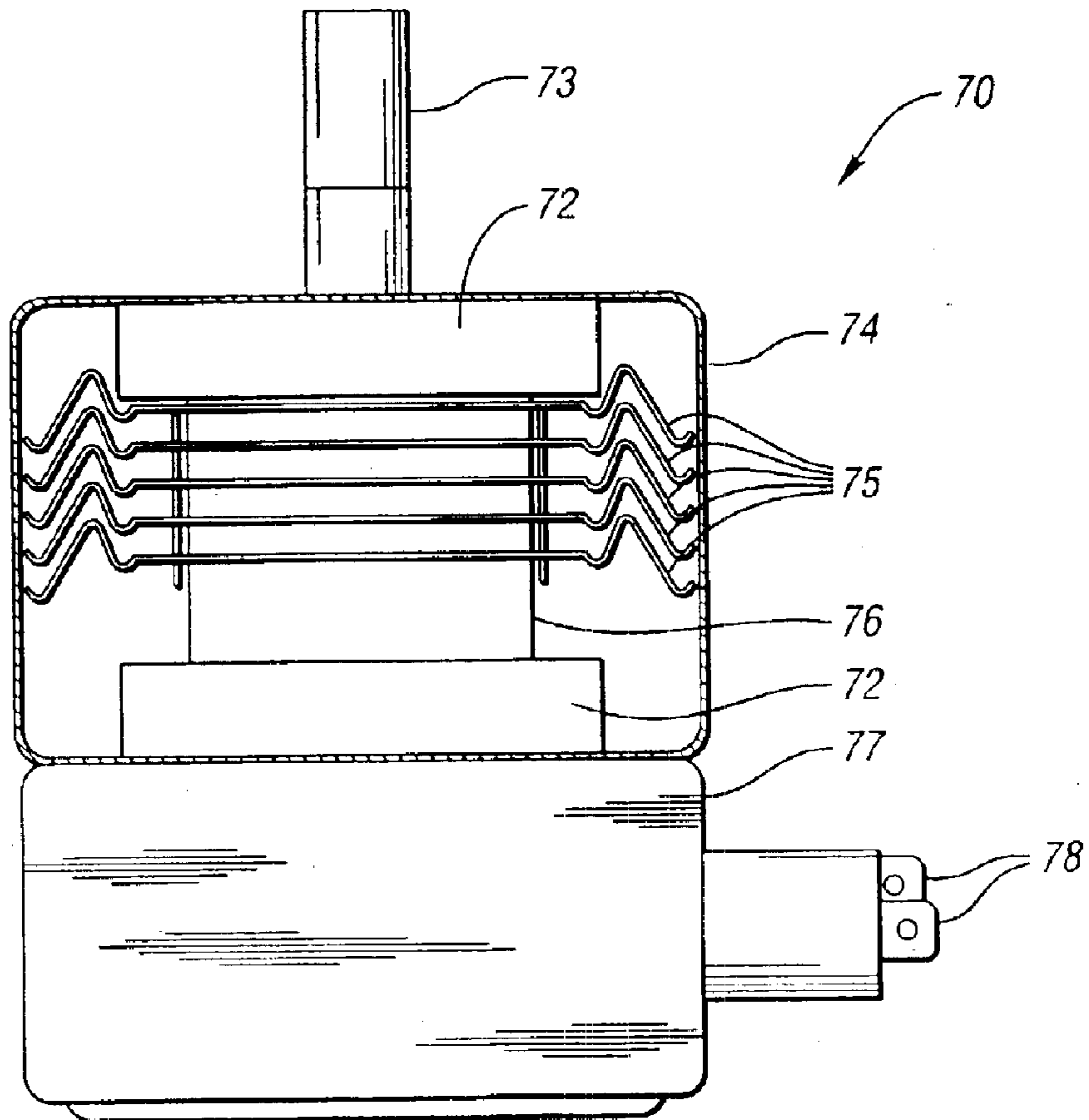
Fig. 7 (PRIOR ART)
