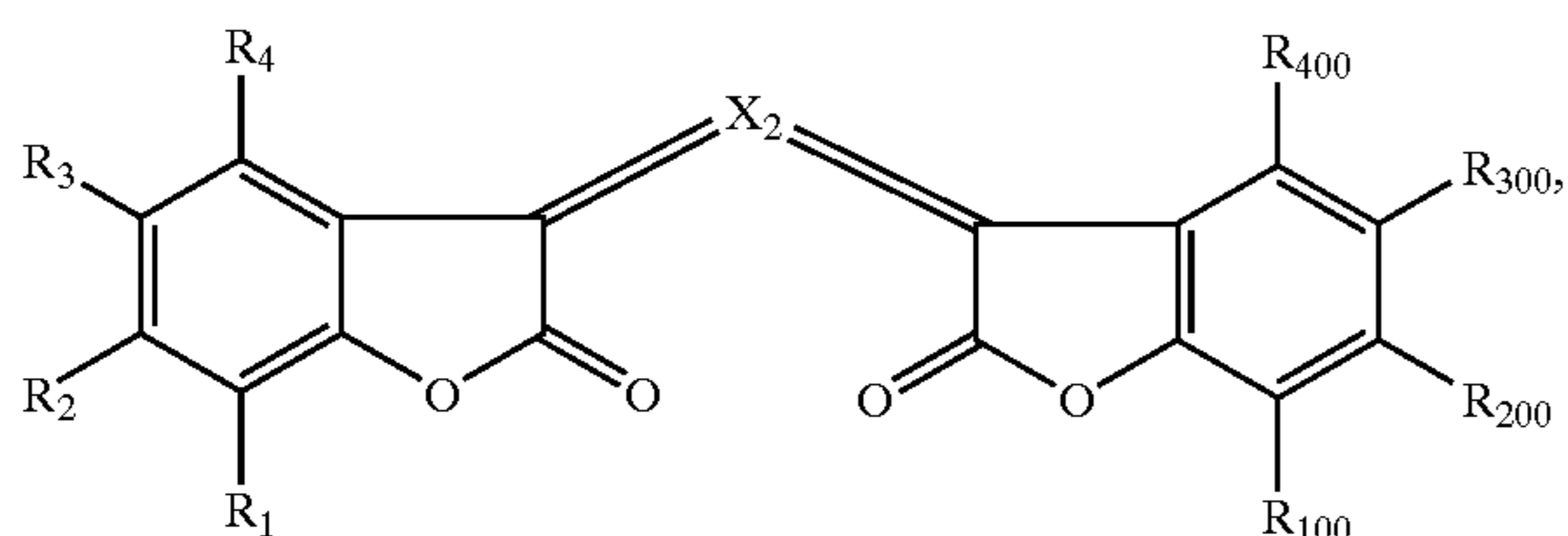
(XLIb)
