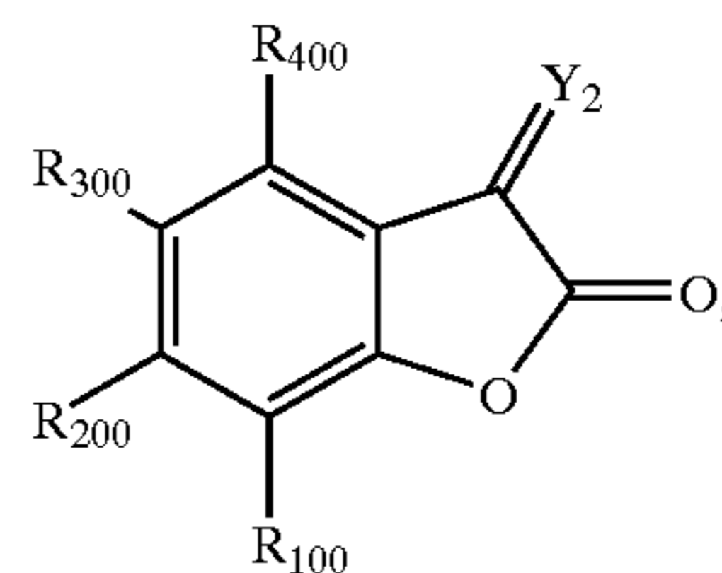
(XXXVIIa)
