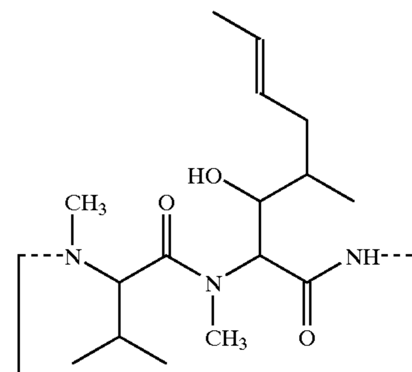
Cyclosporin A
