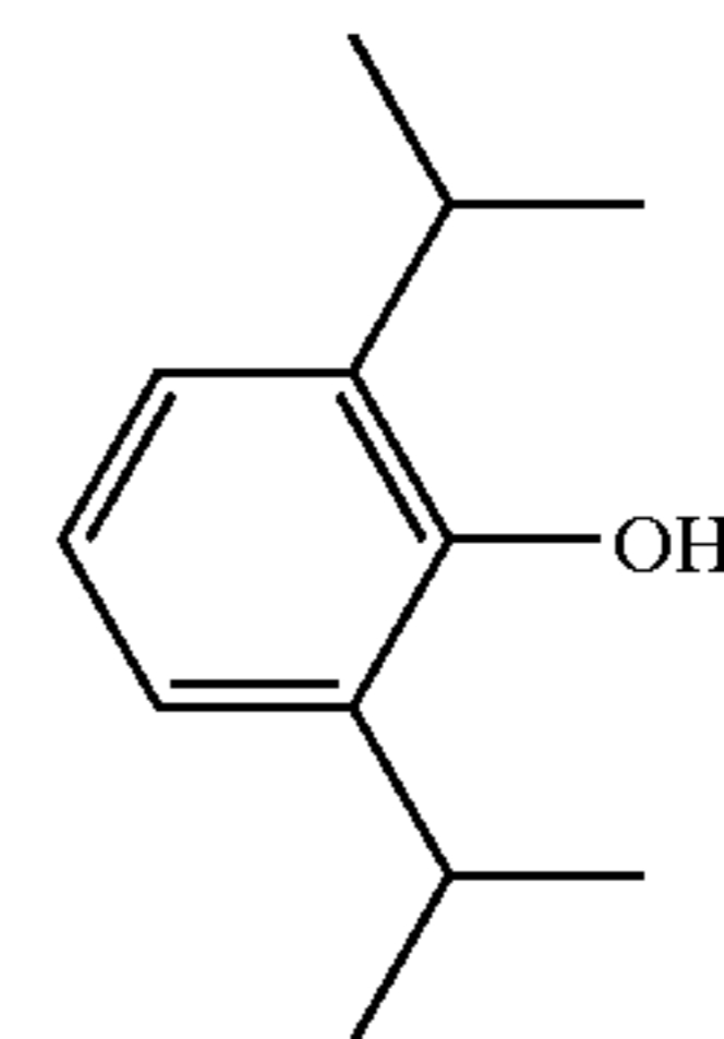
Propofol (2,6-diisopropylphenol)
